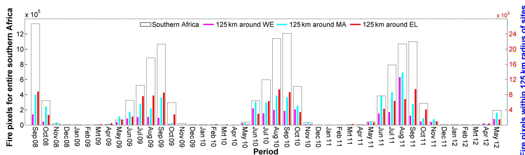
Figure 7. Fire pixels within the entire southern Africa domain ( 10\text{--}35^{\circ}\text{S} , and 10\text{--}41^{\circ}\text{E} ) indicated on the primary y axis, as well as fires pixels within a radius of 125 km around Elandsfontein (EL), Marikana (MA) and Welgegund (WE) measurement sites indicated on the secondary y axis, as determined from the MODIS collection 5 burned area product (Roy et al., 2008).
