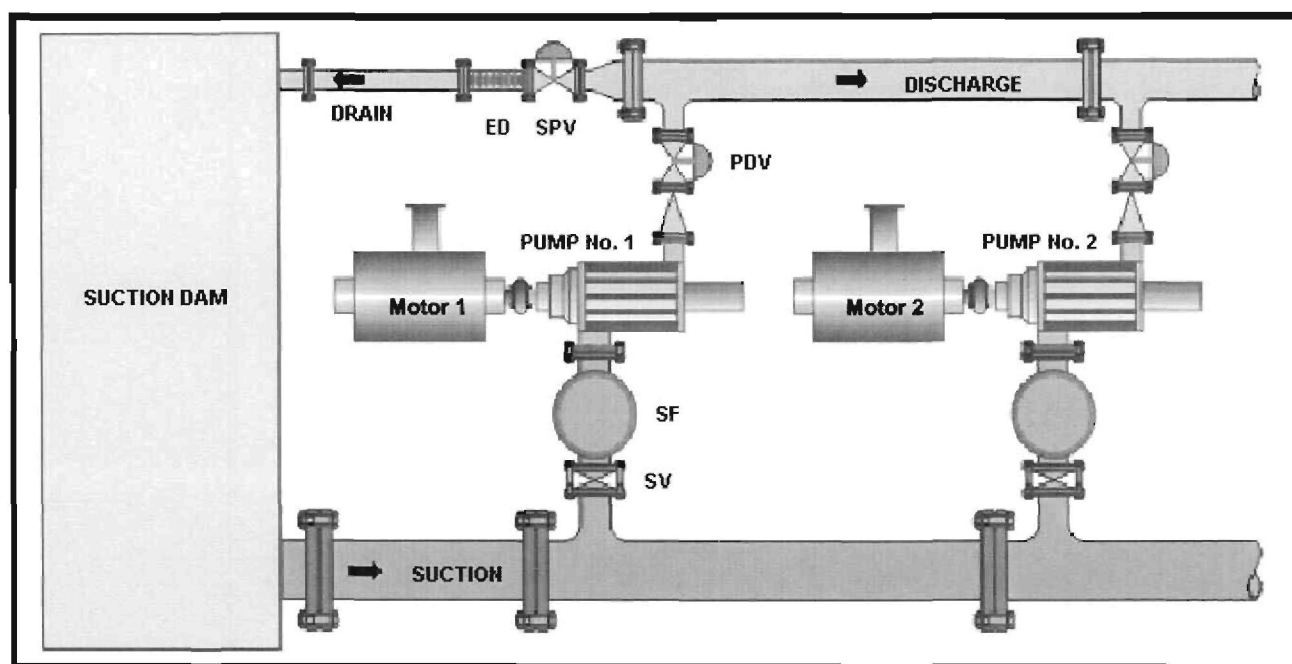
Figure 104: Layout of a typical pump station
