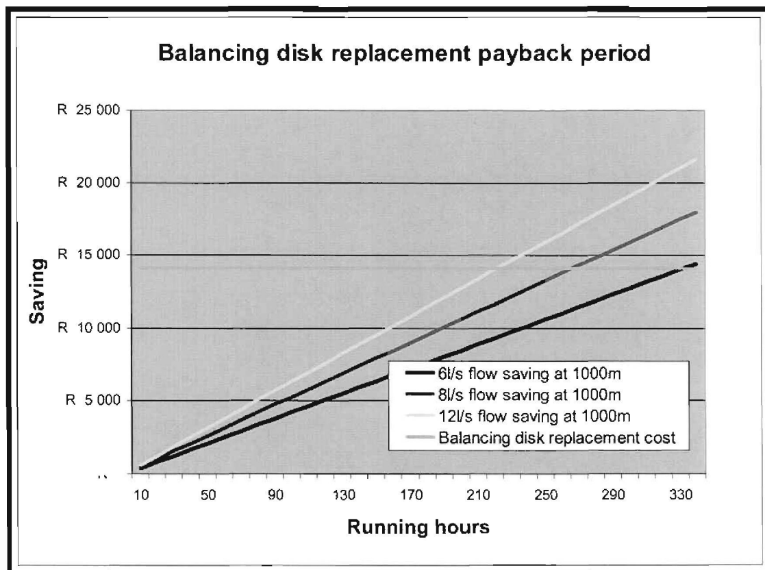
Figure 35: Balancing disk replacement payback period
