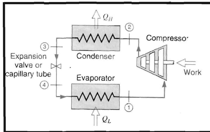
Figure 121: The compression refrigeration cycle [79]
