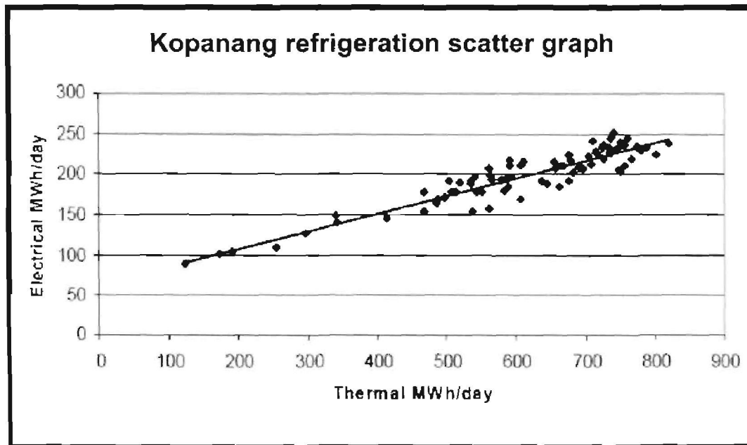
Figure 84: Kopanang thermal and electrical power scatter graph
