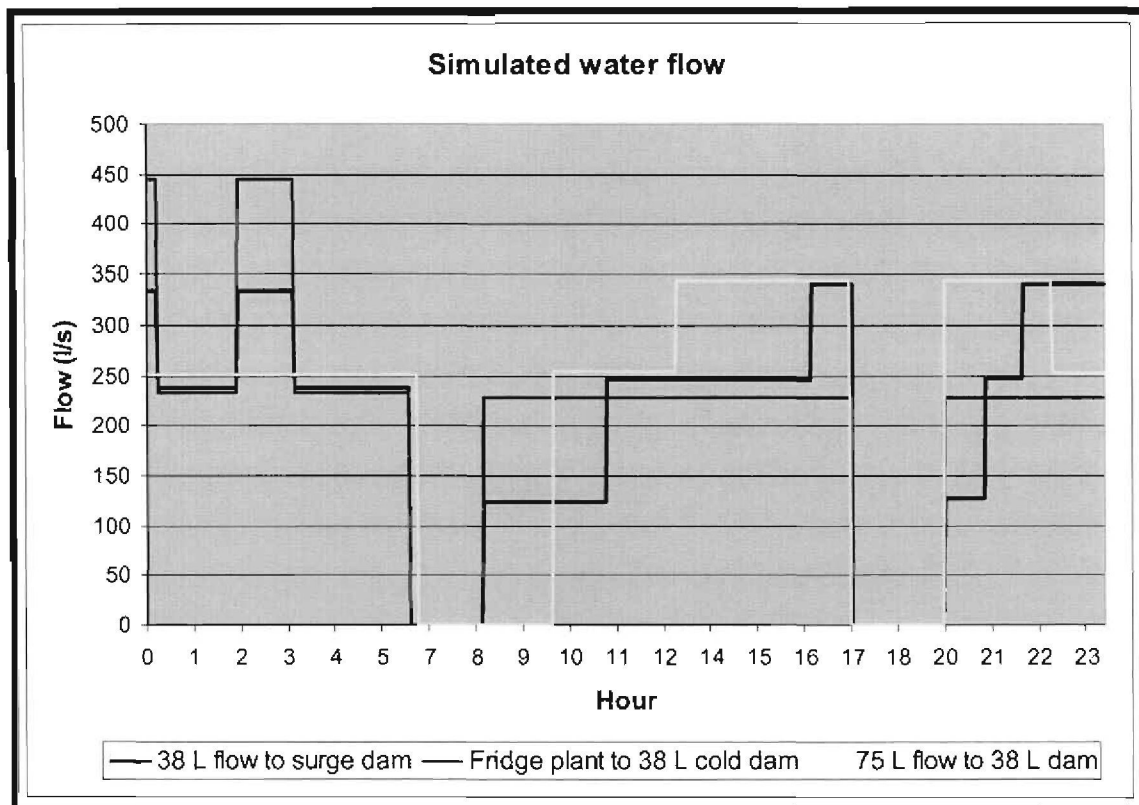
Figure 80: Simulated flow trends of Kopanang Mine
