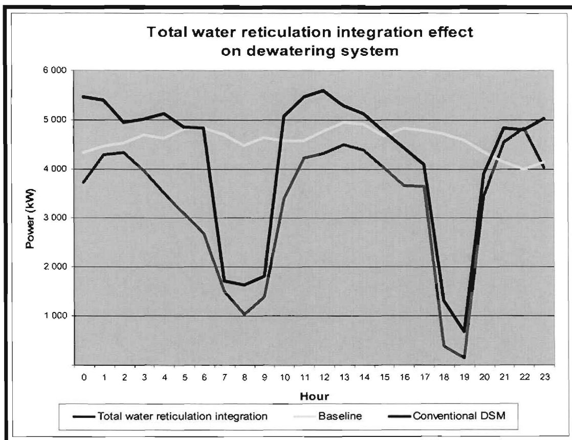
Figure 101: Tshepong dewatering results
