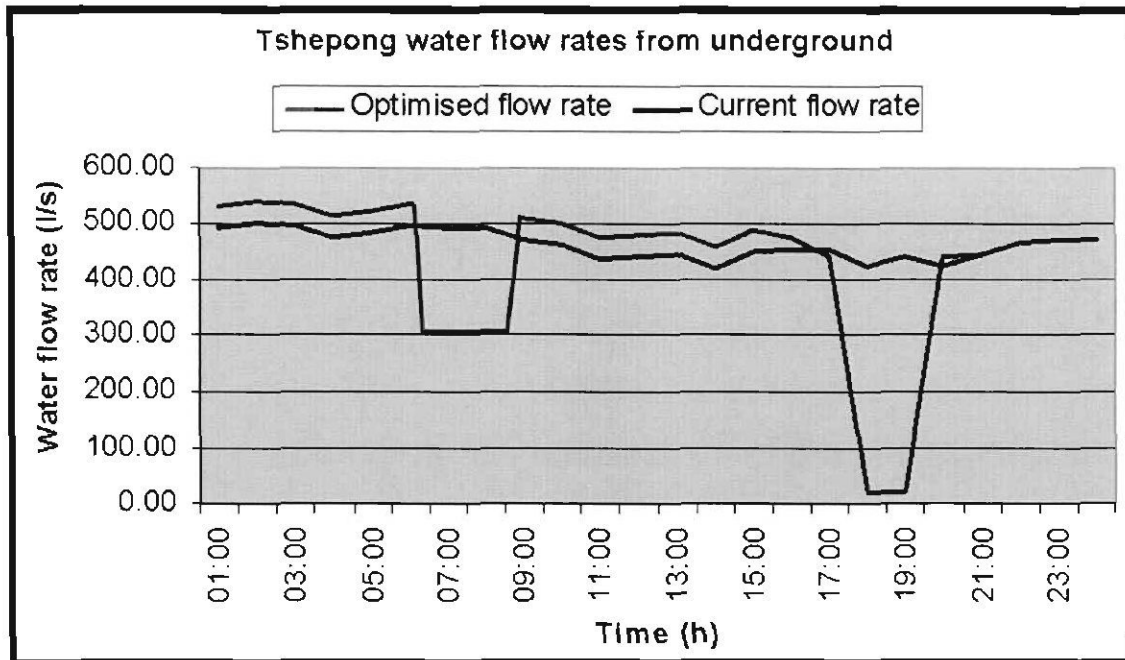
Figure 94: Optimum water flow rates from underground
