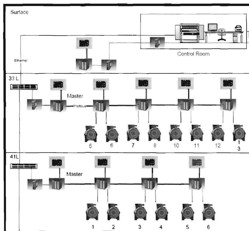
Figure 112: Typical fibre optic network layout
