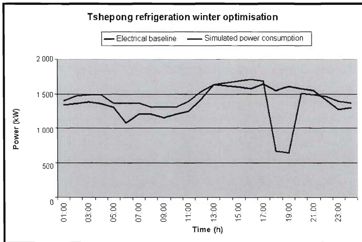
Figure 92: Simulated Tshepong optimised intervention (winter)
