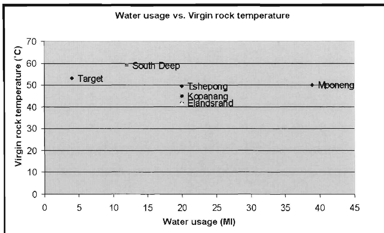
Figure 24: Virgin rock temperatures vs. water usage
