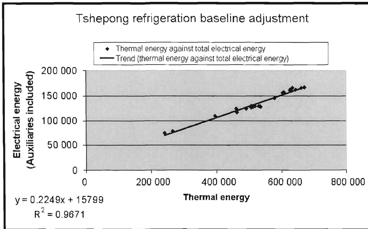
Figure 98: Total system thermal energy against total system electrical energy
