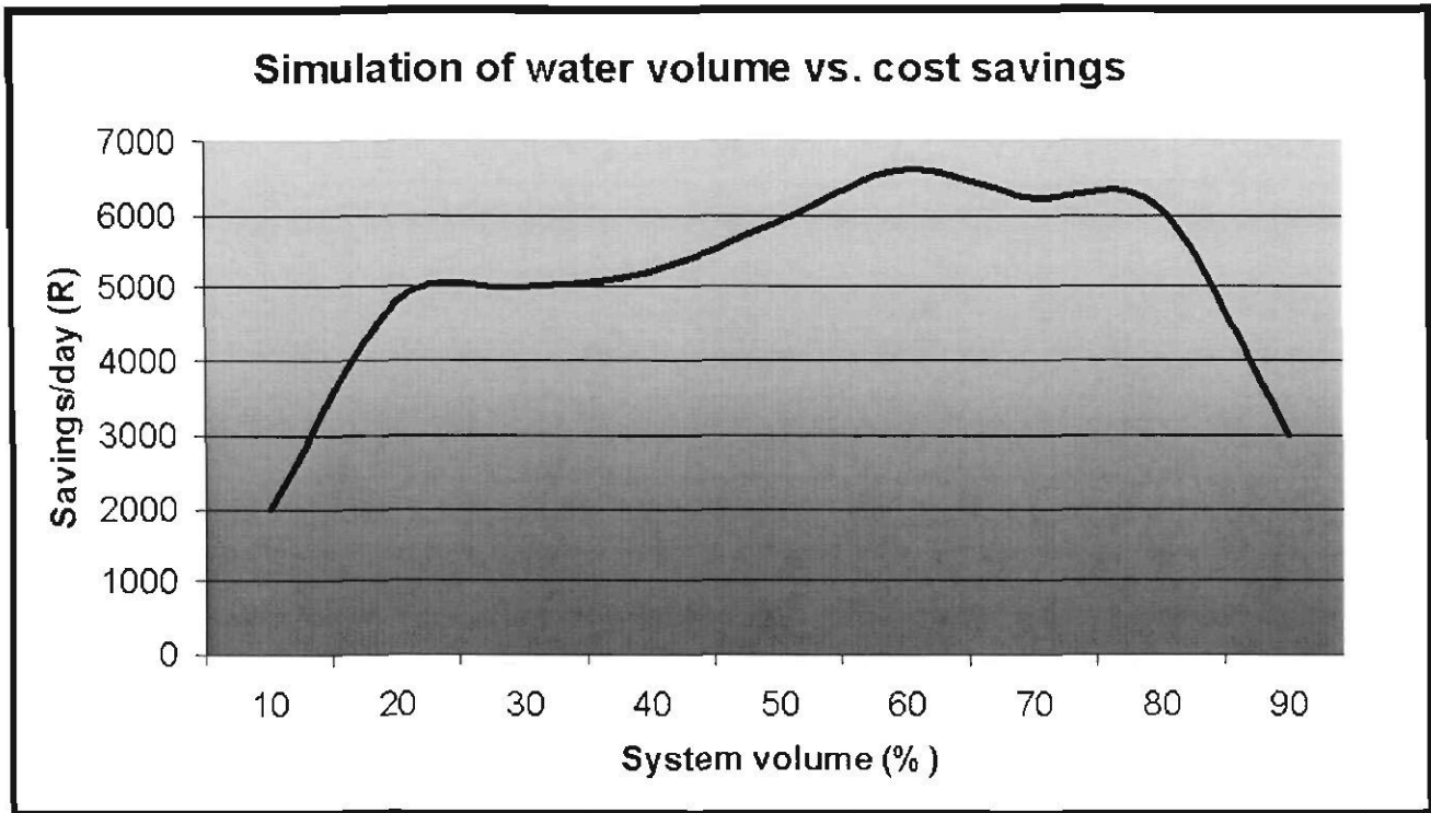
Figure 75: Simulation of system water volume vs. savings/day
