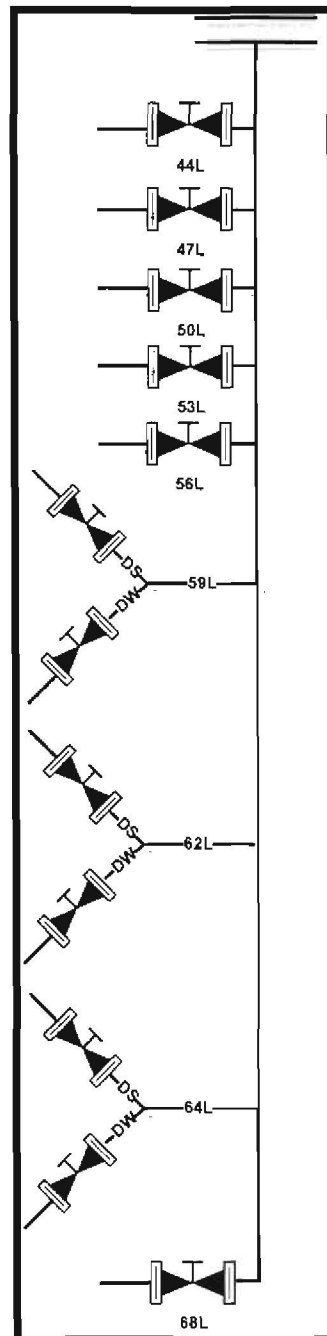
Figure 62: Underground level water distribution layout
