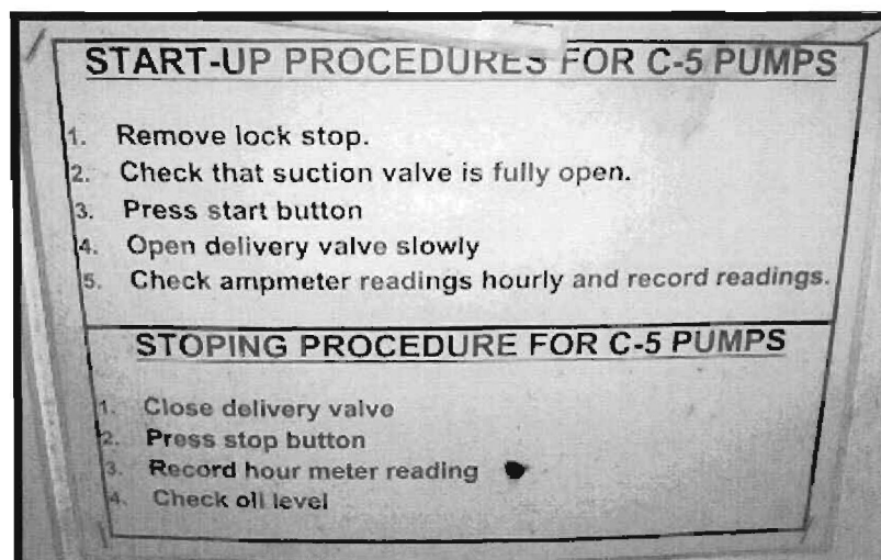
Figure 16: Start-up and stopping procedures for C-5 pumps [32]
