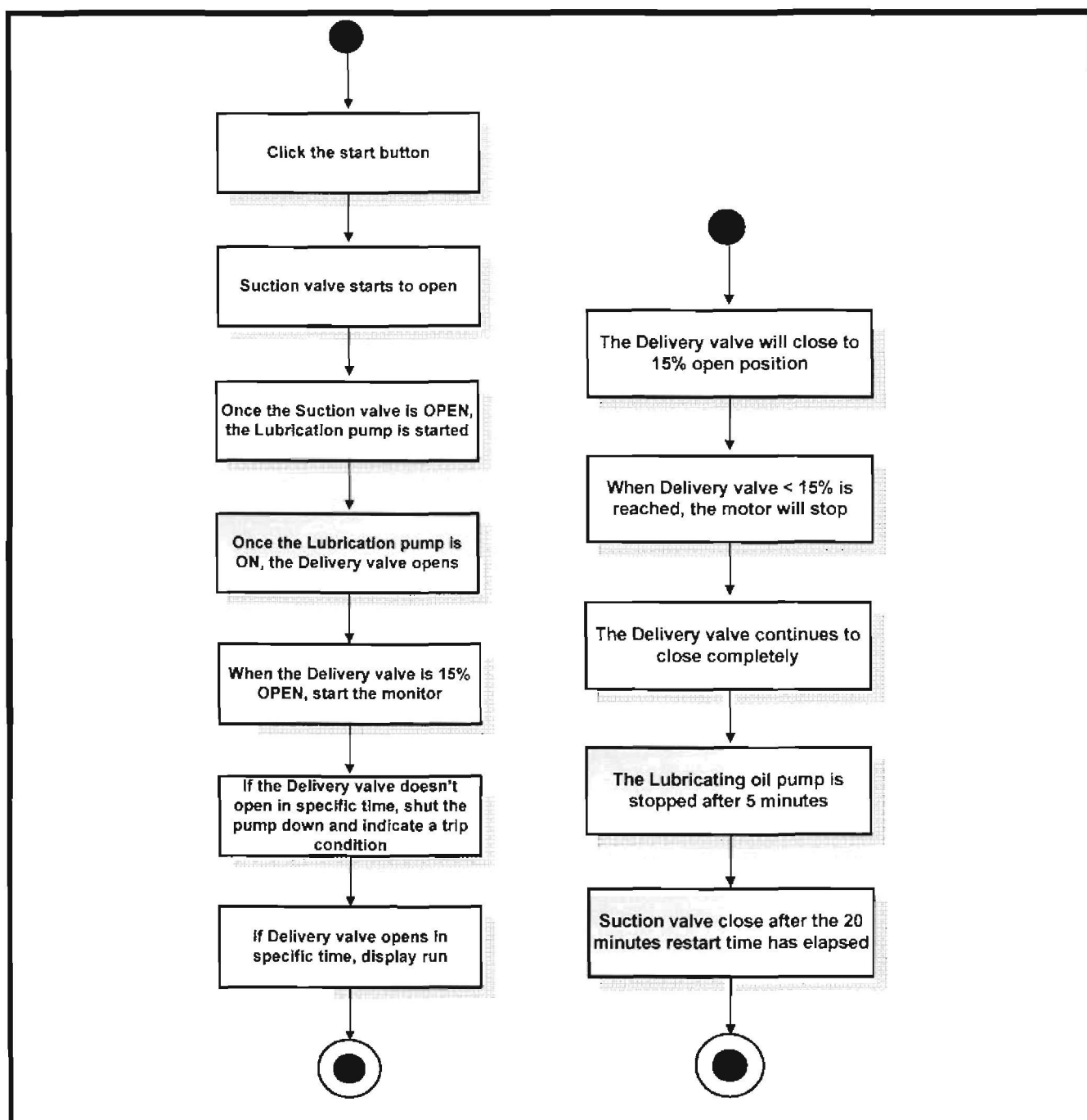
Figure 114: Start and Stop sequence of a typical mine automated dewatering pump
