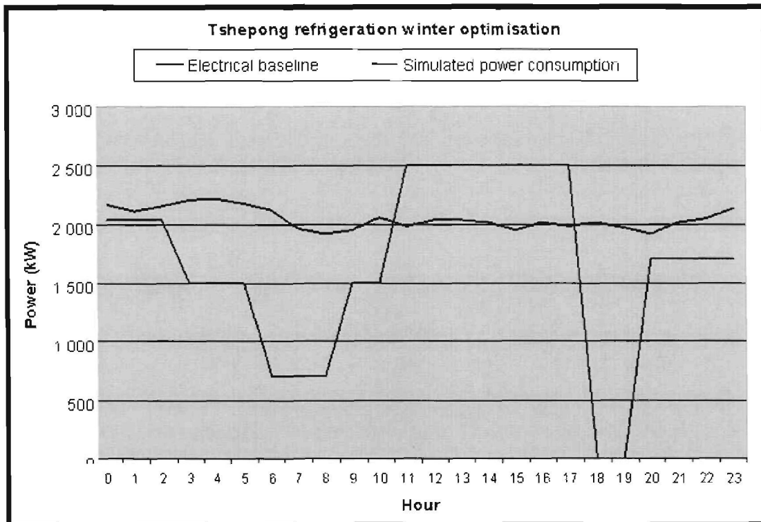
Figure 96: New Tshepong refrigeration optimised intervention (winter)
