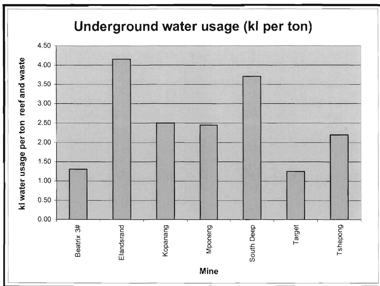
Figure 28: Graph representation of underground water usage
