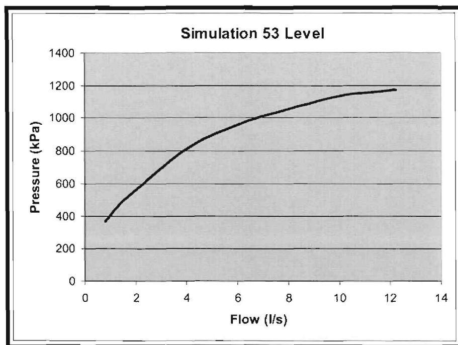
Figure 48: Relation between water pressure and flow
