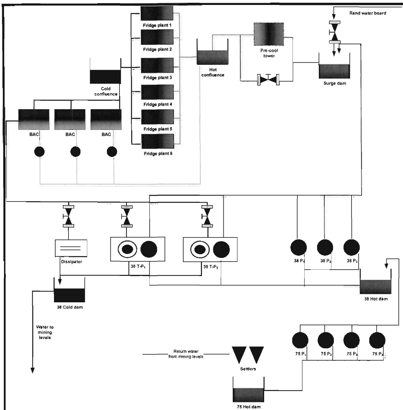
Figure 77: Kopanang total water reticulation layout
