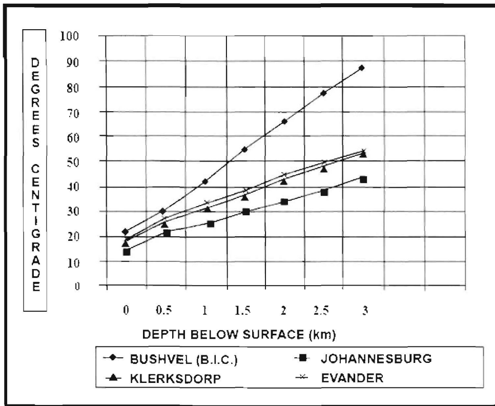
Figure 23: Virgin rock temperatures below surface [49]
