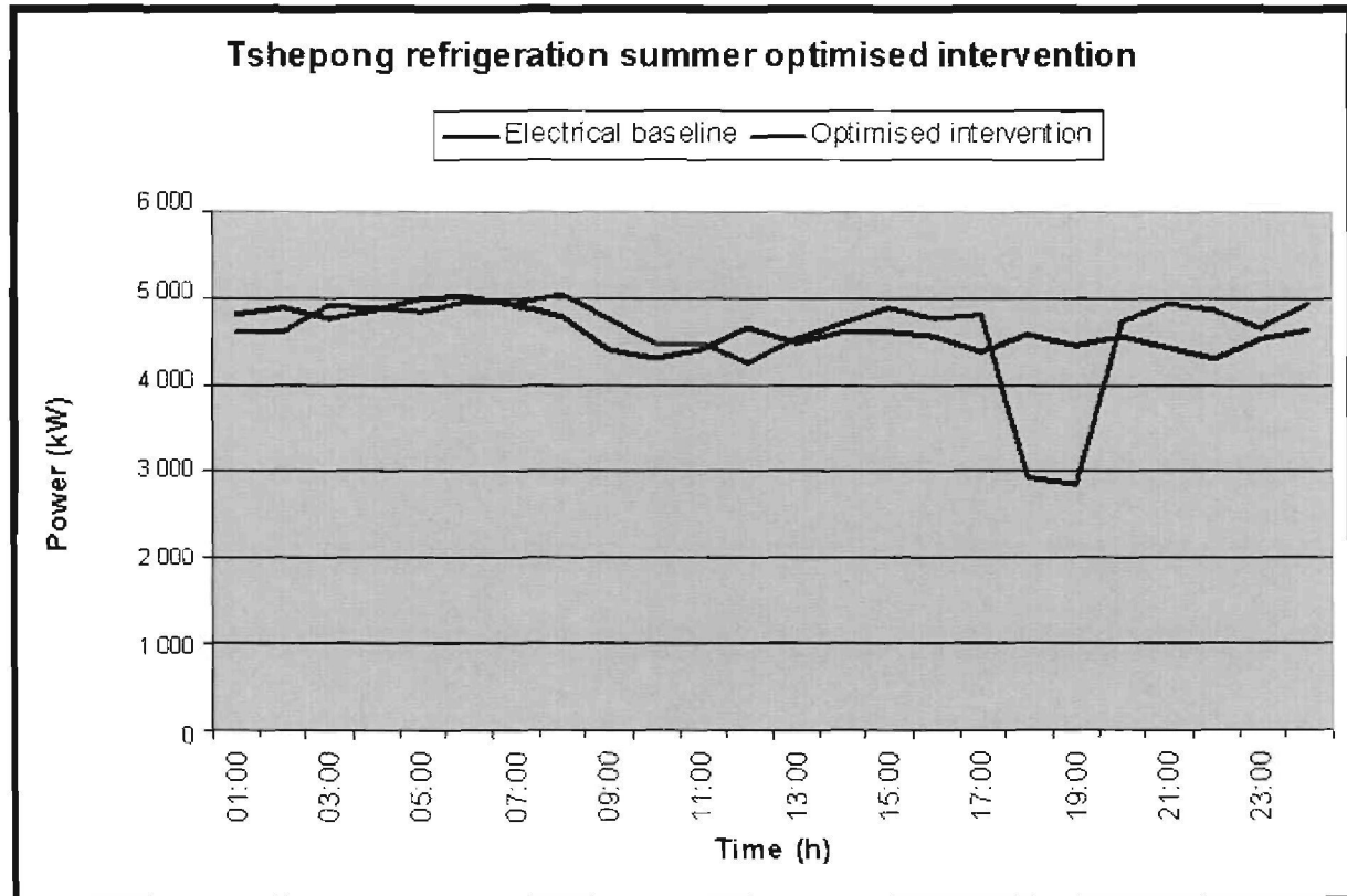
Figure 91: Simulated Tshepong optimised intervention (summer)
