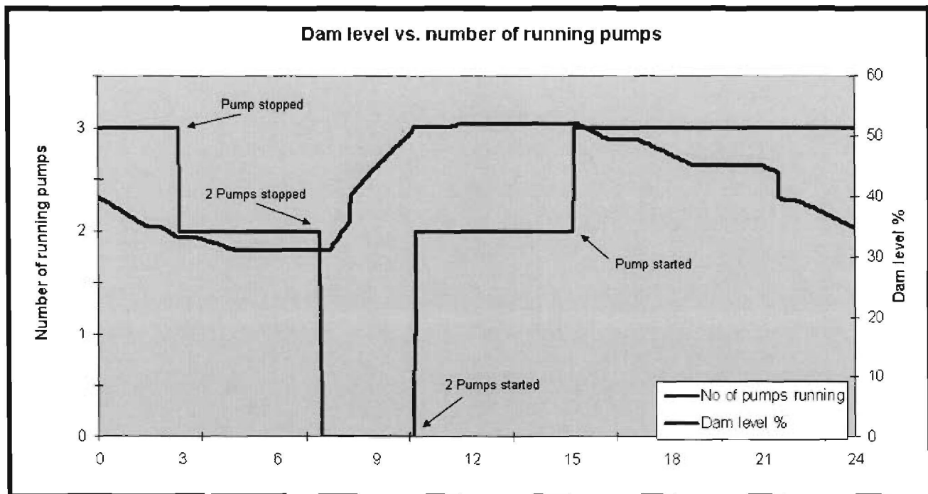
Figure 15: Typical control philosophy of underground pump operators
