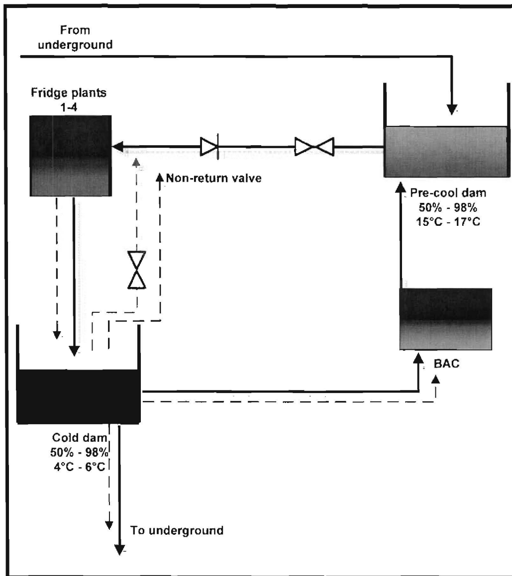
Figure 90: Proposed water balance during peak period.
