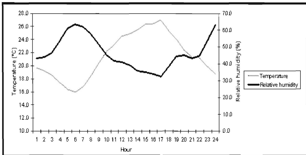
Figure 74: Relation of the outdoor air temperature to the relative humidity [23]
