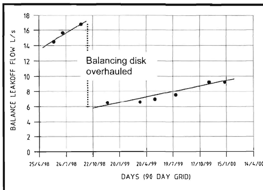
Figure 34: Data plot of balance leak off-flow for a multi-stage pump [54]
