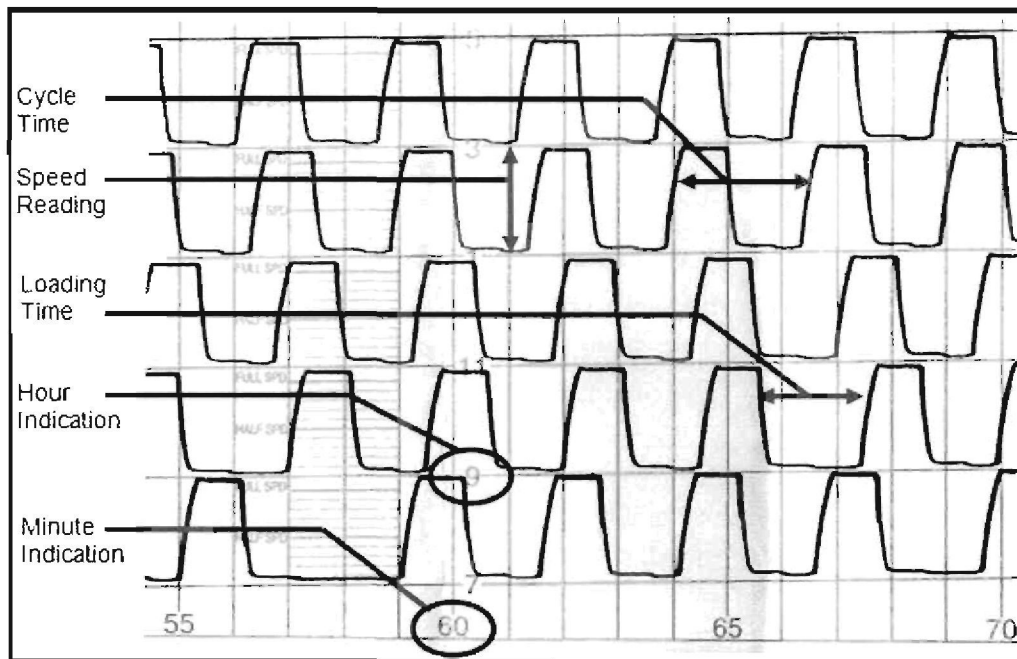
Figure 25: Example of a rock winder tachograph
