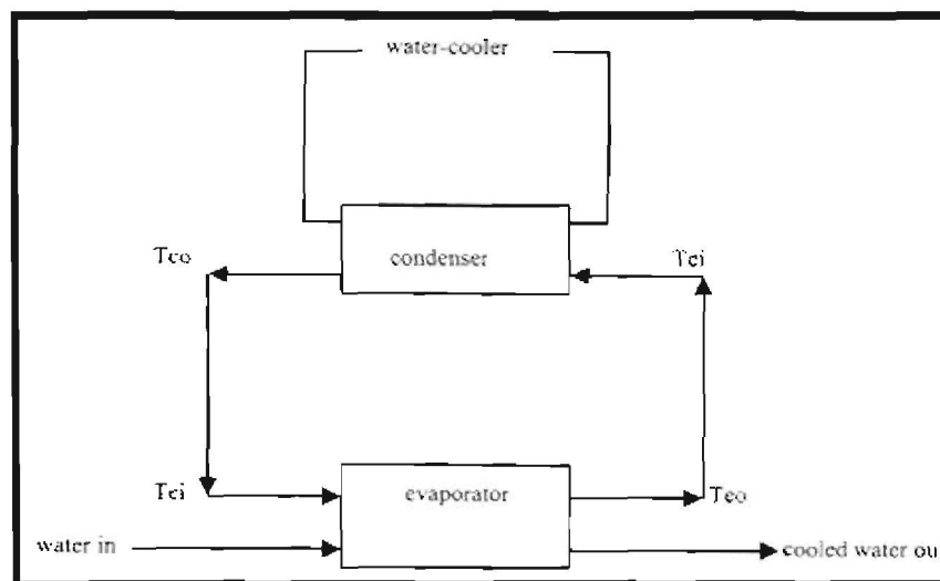
Figure 120: Schematic layout of a water-cooled refrigeration plant [78]
