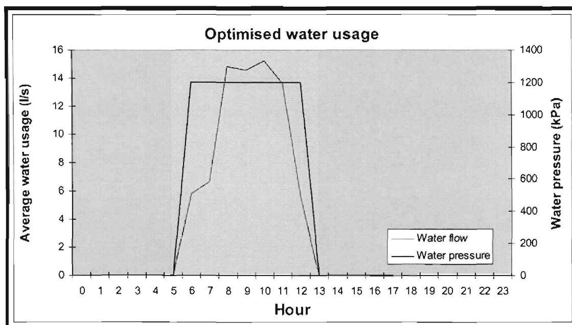
Figure 49: Optimised water schedule
