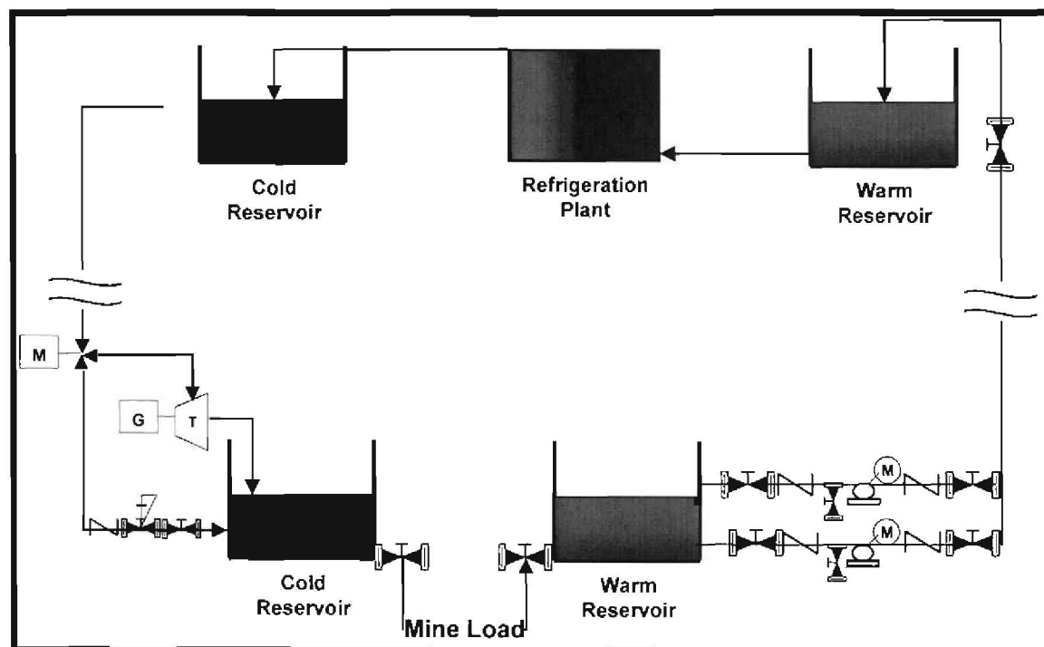
Figure 117: Turbine-generator configuration
