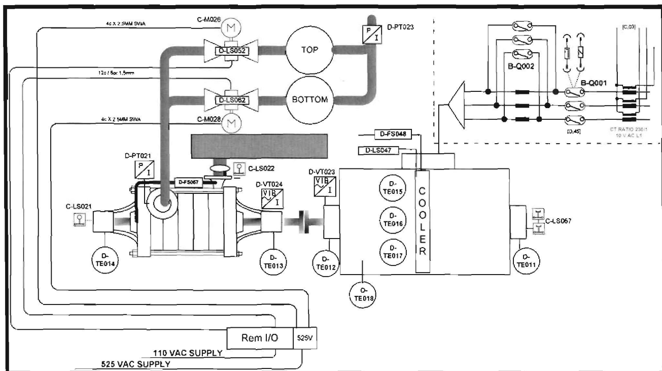
Figure 113: Instrumentation layout of a pump
