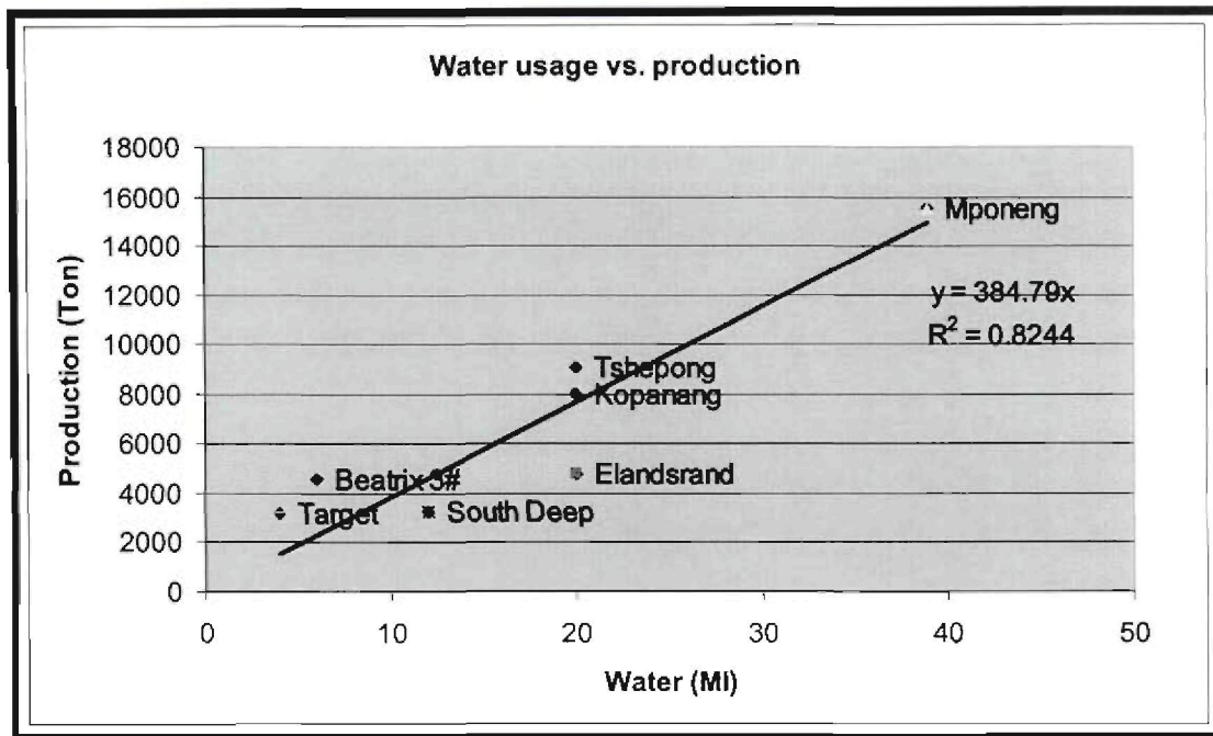
Figure 26: Production vs. water usage
