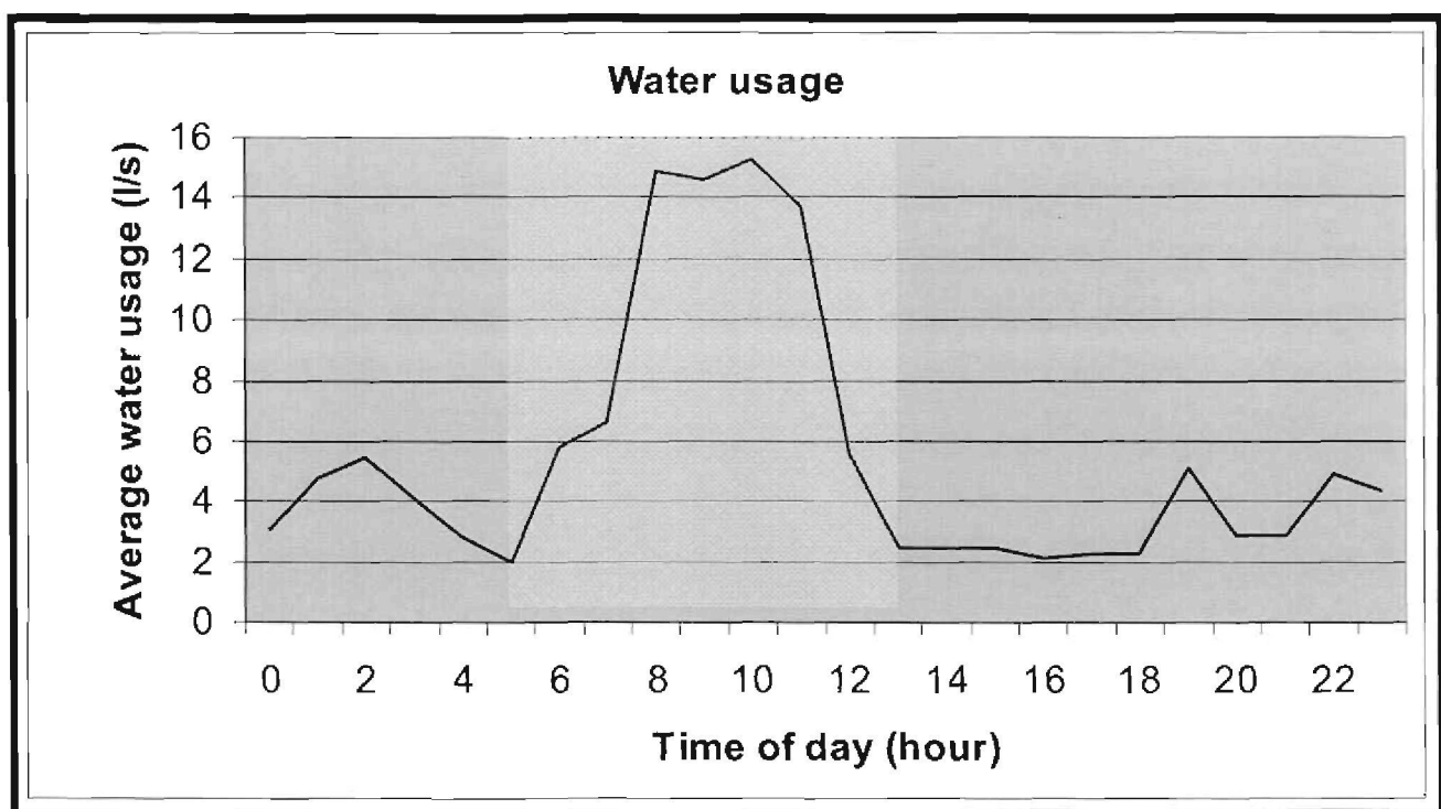
Figure 46: Water usage on a typical production level
