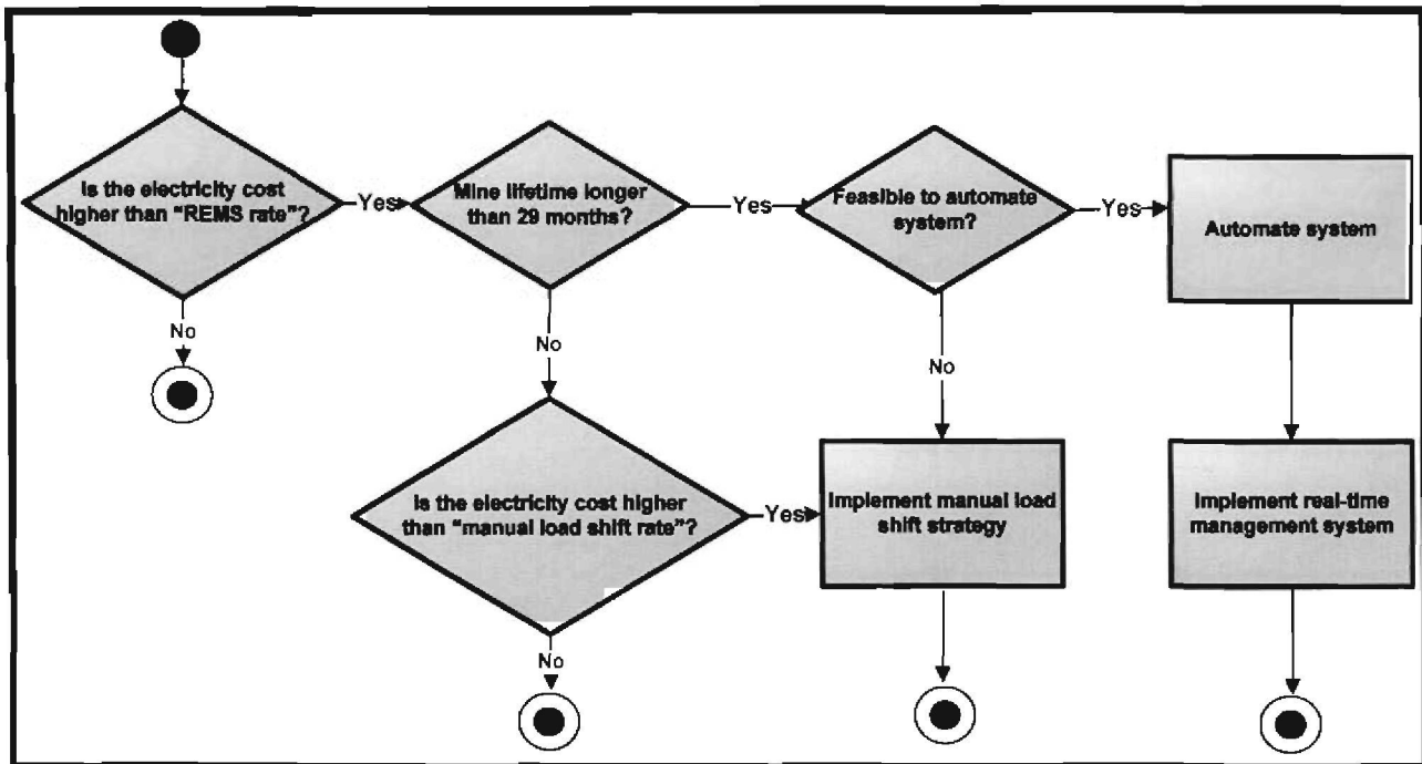
Figure 39: Electricity cost (c/kWh) optimisation model
