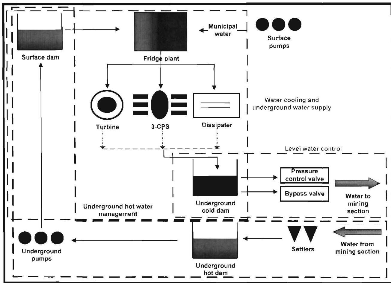
Figure 69: Water reticulation layout
