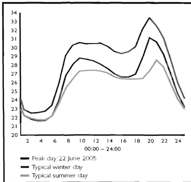
Figure 1: Daily electricity demand [11]
