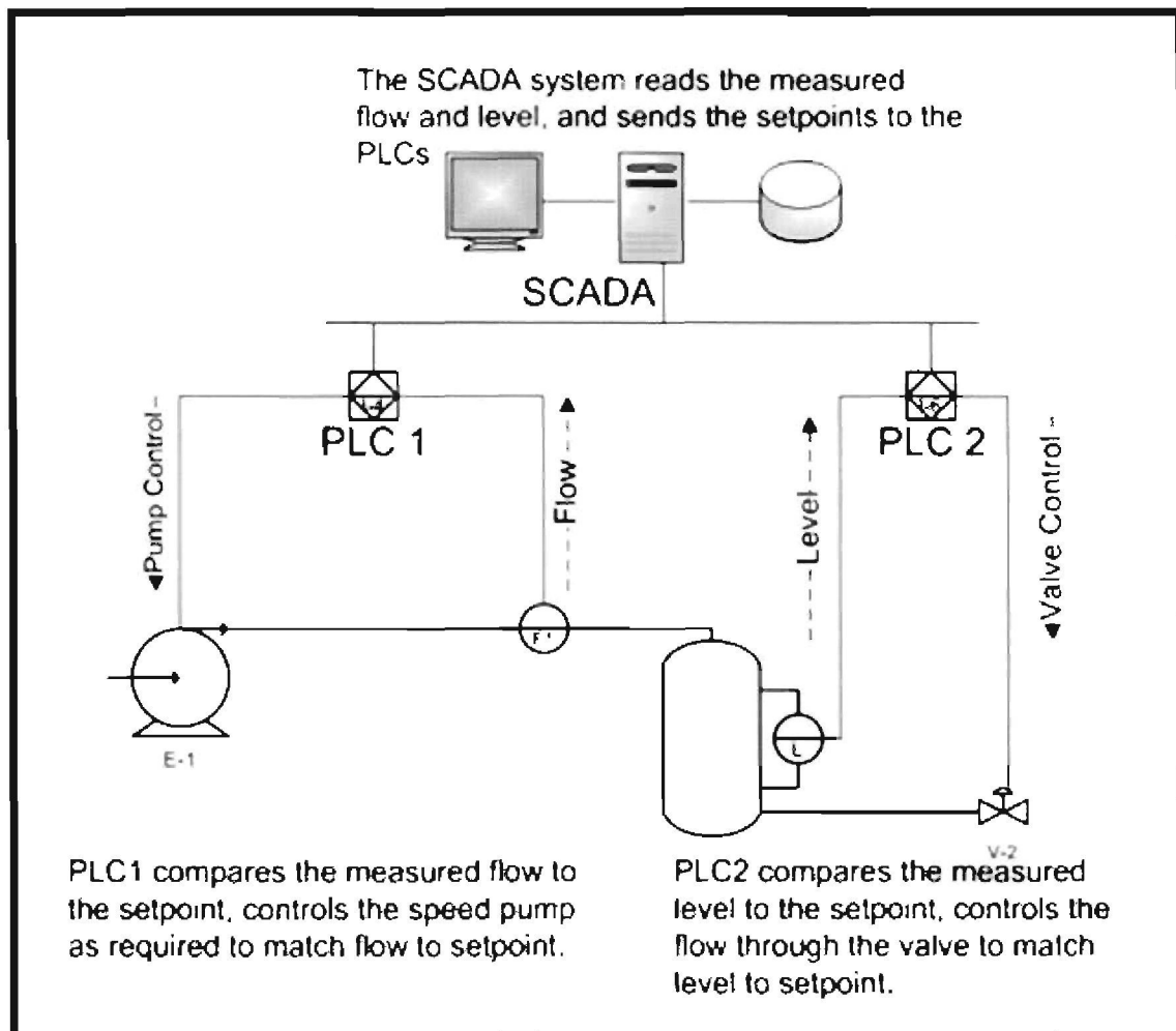
Figure 17: Typical PLC and SCADA layouts
