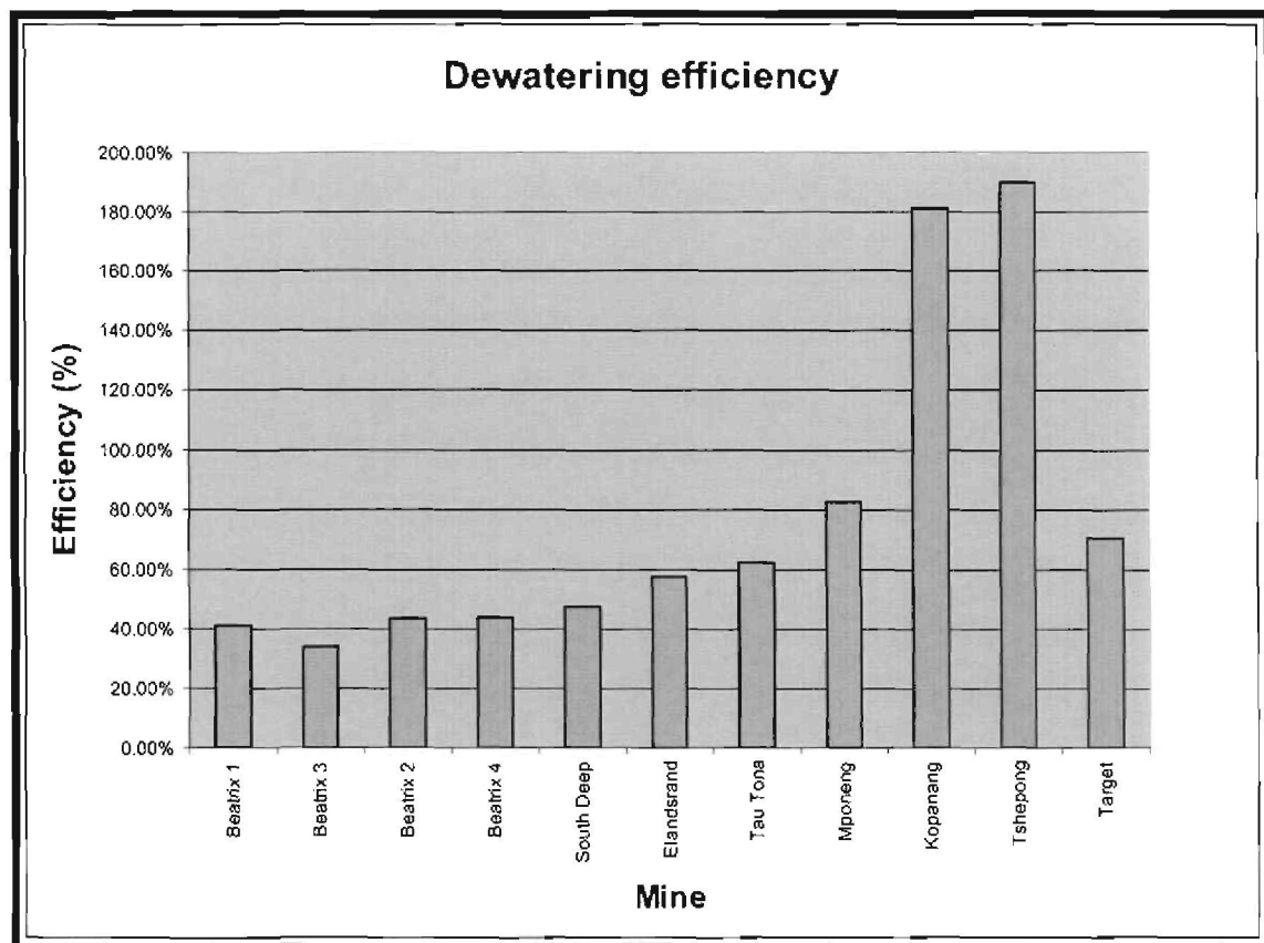
Figure 20: Dewatering efficiency
