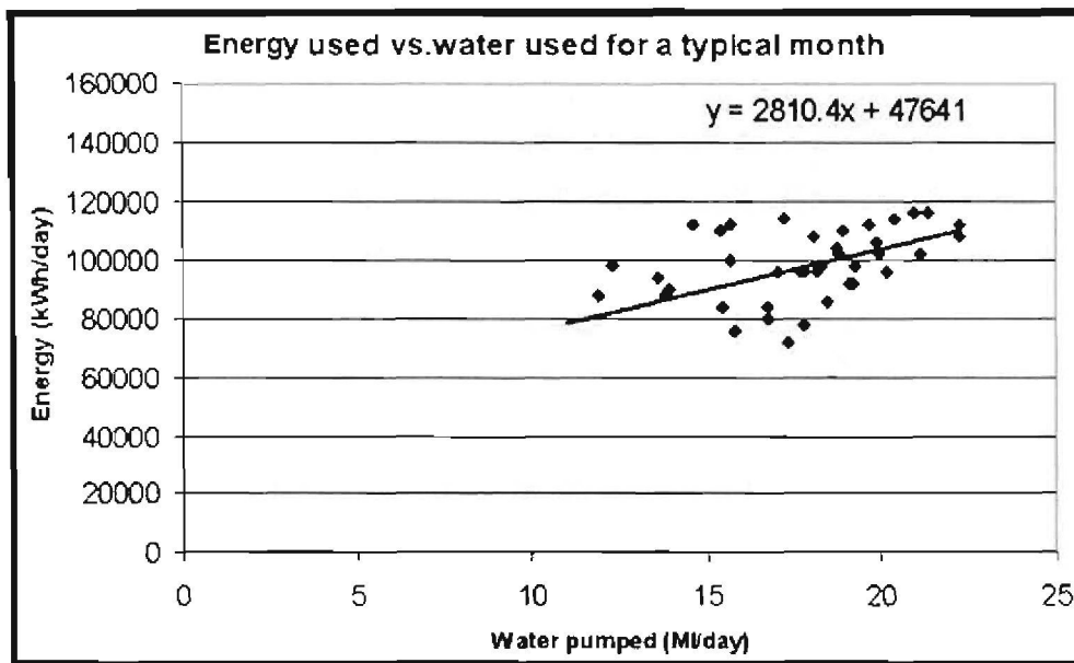
Figure 57: Beatrix 1 Shaft water pumped against power used
