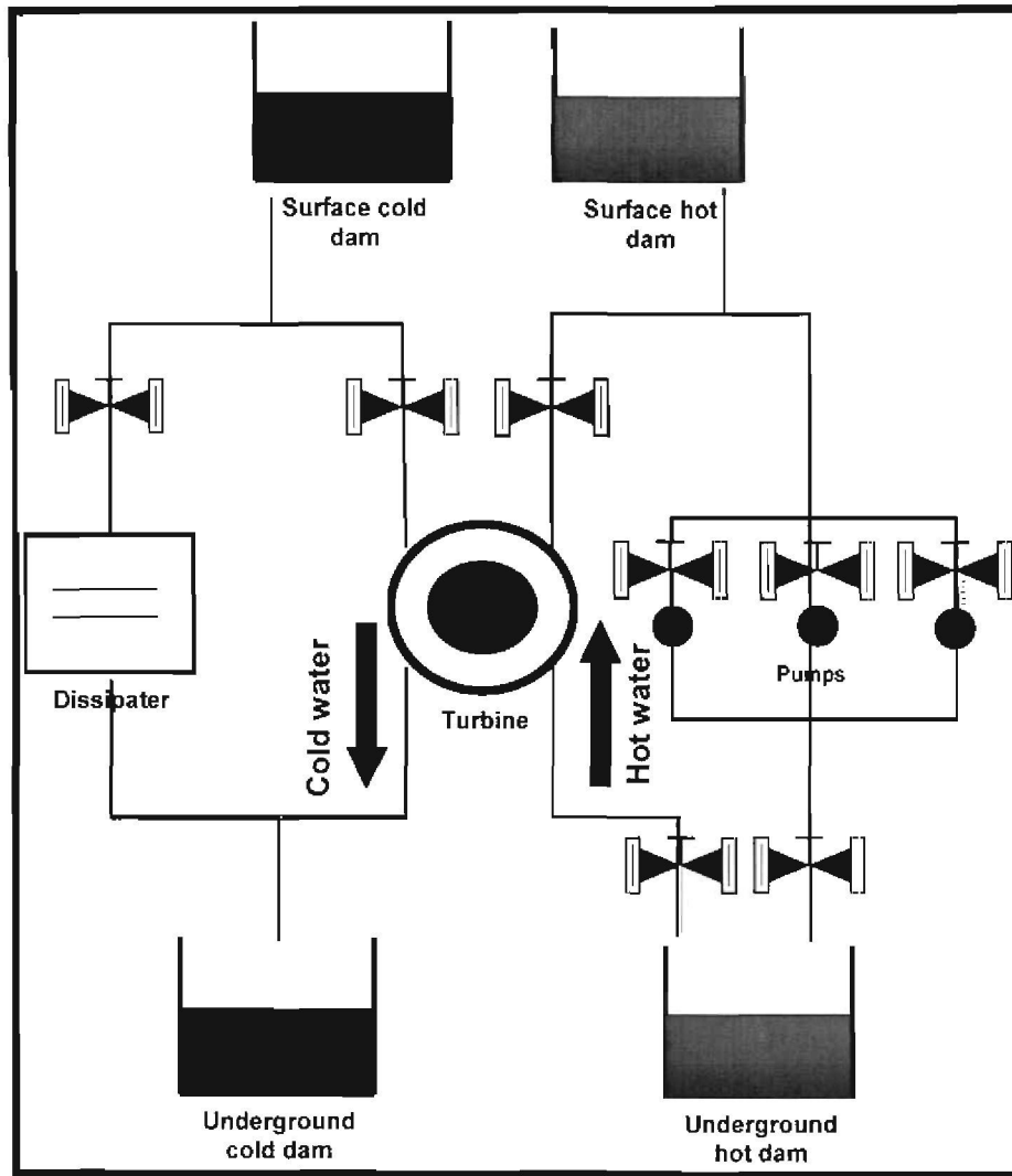
Figure 71: Turbine-pump system
