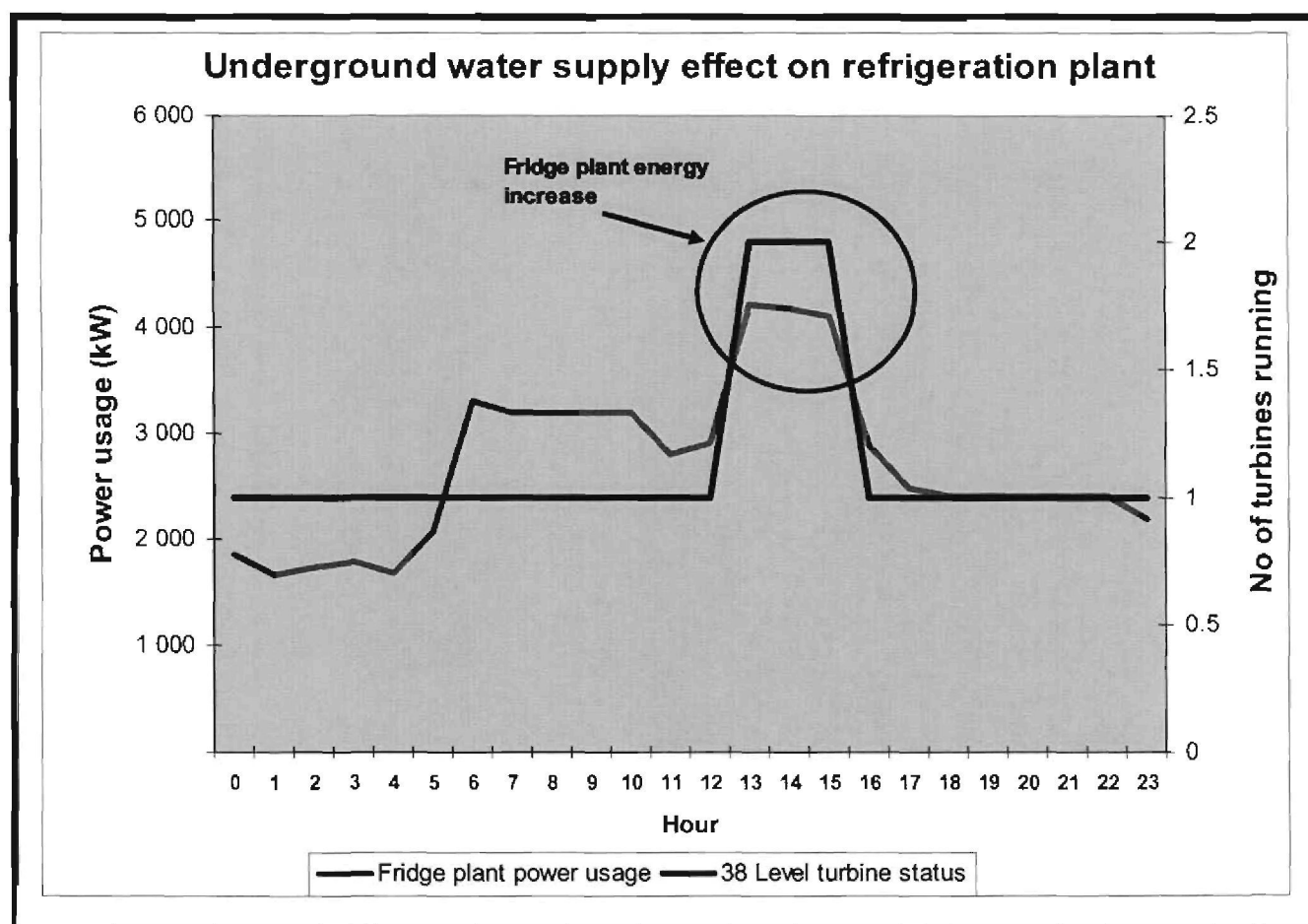
Figure 79: Underground water supply effect on refrigeration plant
