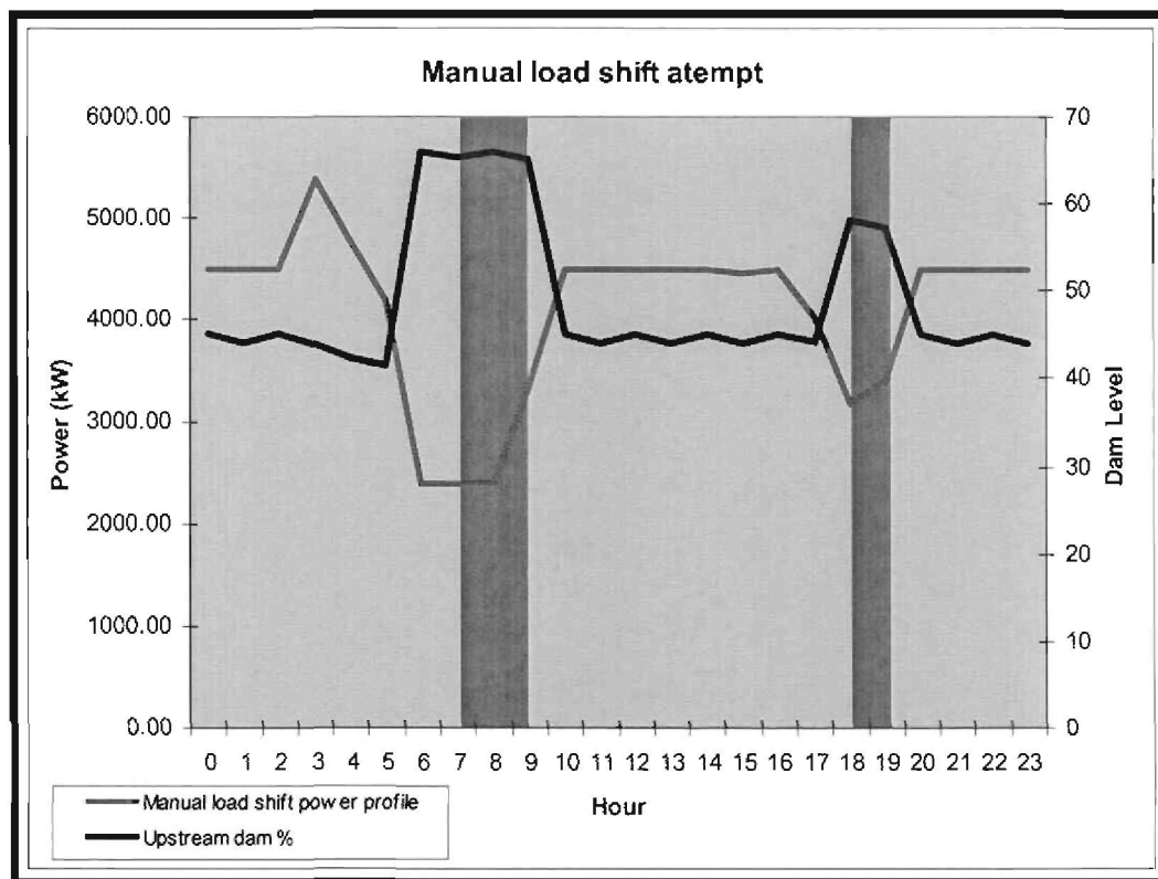
Figure 41: Manual load shift prediction
