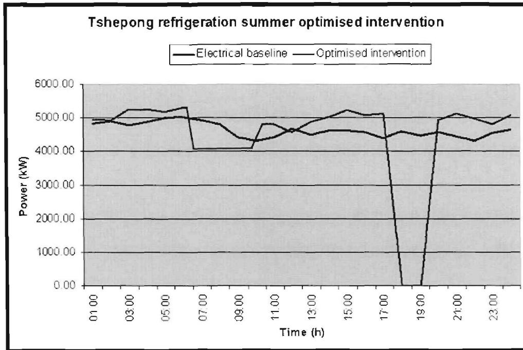
Figure 95: New Tshepong refrigeration optimised intervention (summer)
