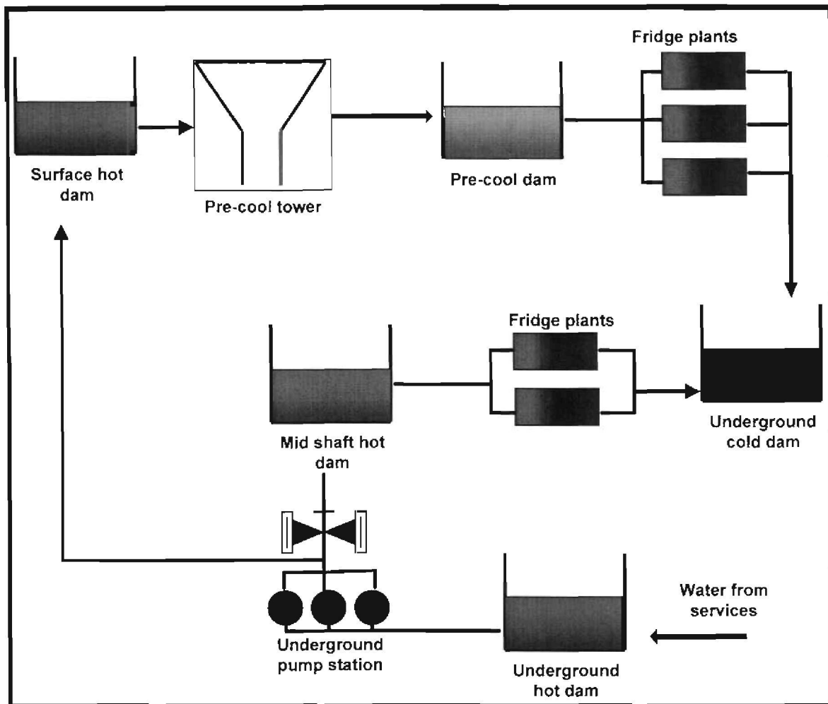
Figure 72: Dewatering supply to refrigeration plant
