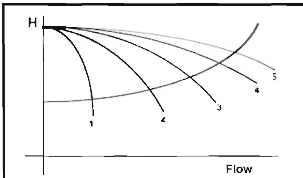
Figure 32: Performance curve for multiple pumps
