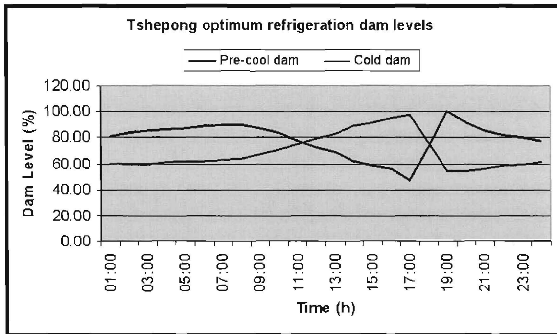
Figure 97: Tshepong optimum refrigeration dam levels
