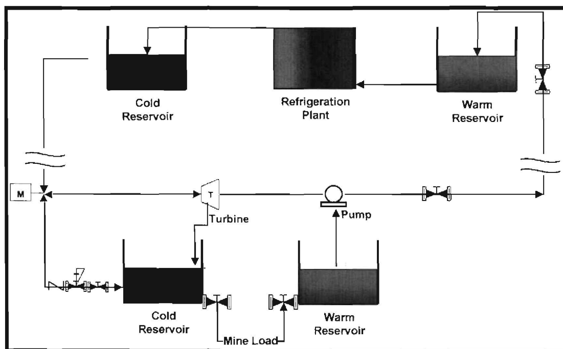
Figure 118: Turbine-pump configuration
