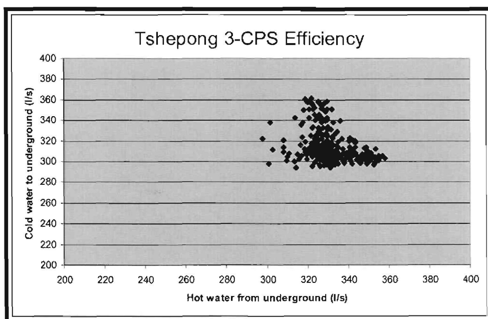
Figure 38: Tshepong mine 3-CPS efficiency calculation
