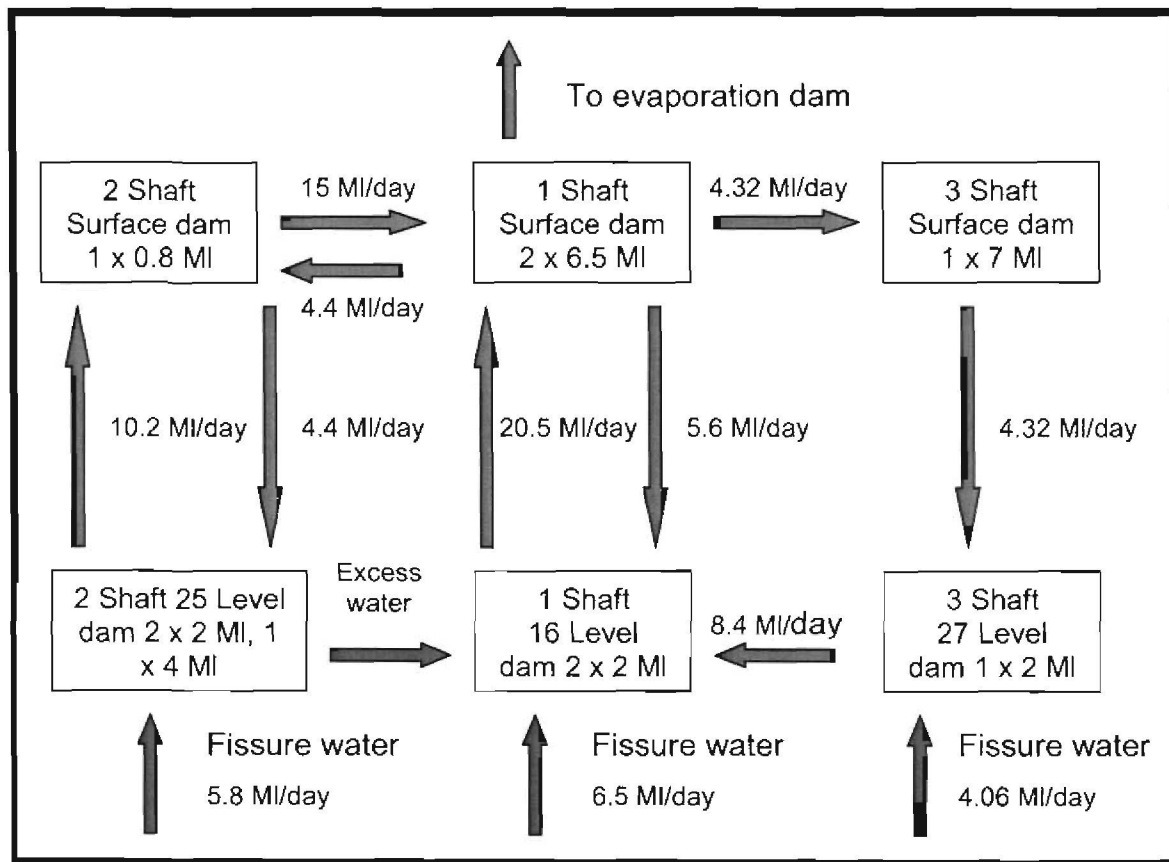
Figure 51: Beatrix 1 Shaft, 2 Shaft and 3 Shaft water network
