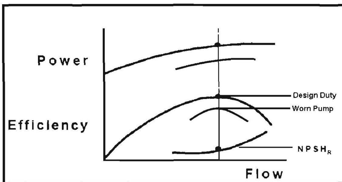
Figure 14: Effect of deterioration on pump characteristics
