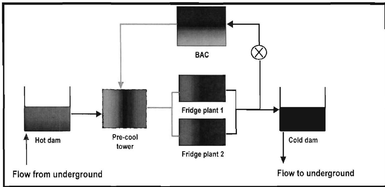
Figure 8: Typical refrigeration of a mine
