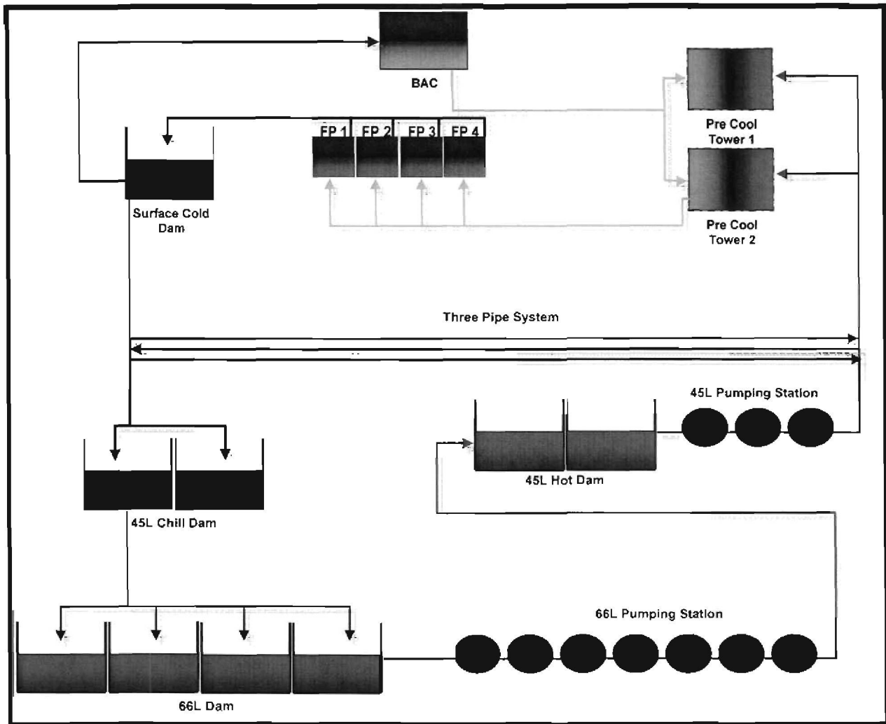
Figure 88: Tshepong 3-CPS, refrigeration and dewatering integration
