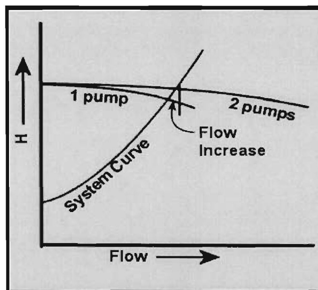
Figure 31: Flow increase due to parallel operation [53].
