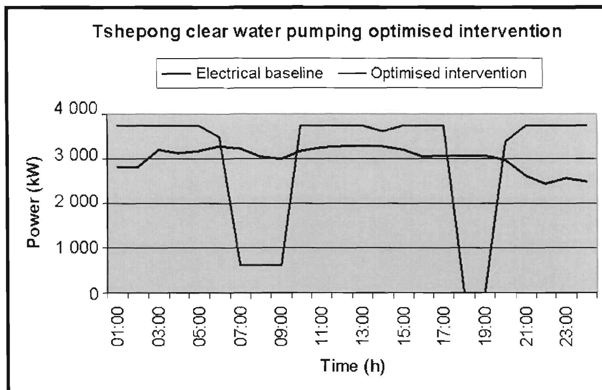
Figure 93: Tshepong pumping optimised intervention
