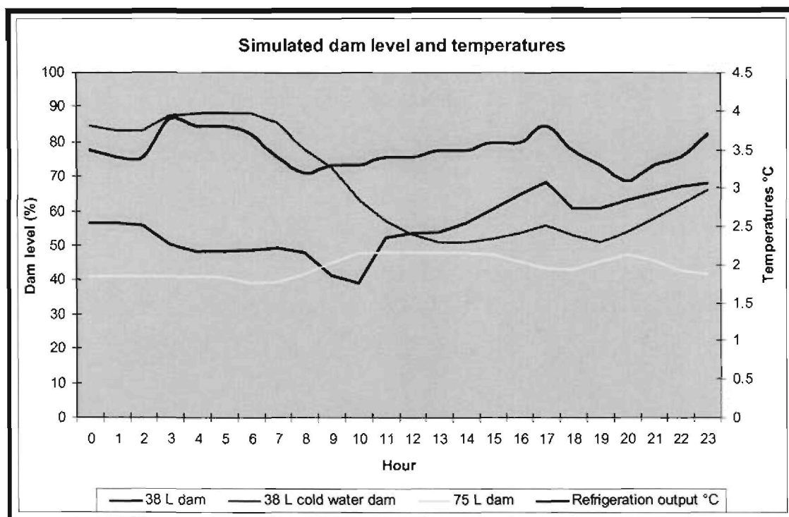
Figure 81: Simulated dam levels
