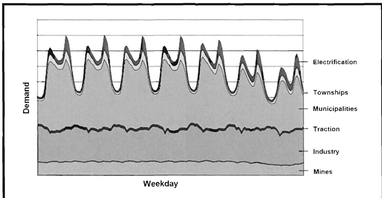
Figure 7: Weekly Total electricity demand (%)
