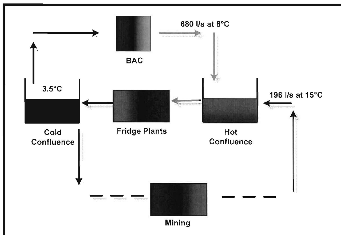
Figure 66: Water reticulation of Kopanang refrigeration plant system
