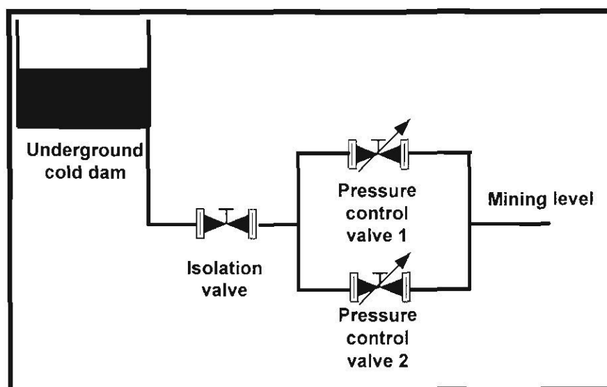
Figure 44: Water supply valve configurations
