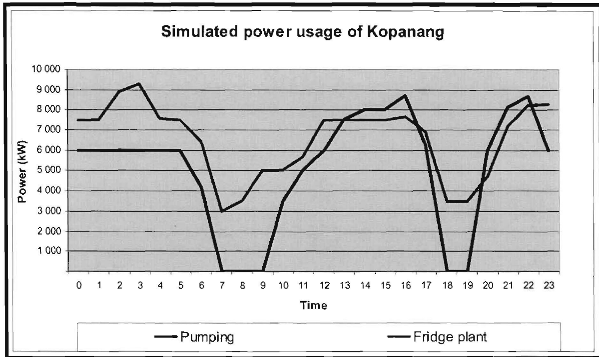
Figure 82: Simulated power profiles
