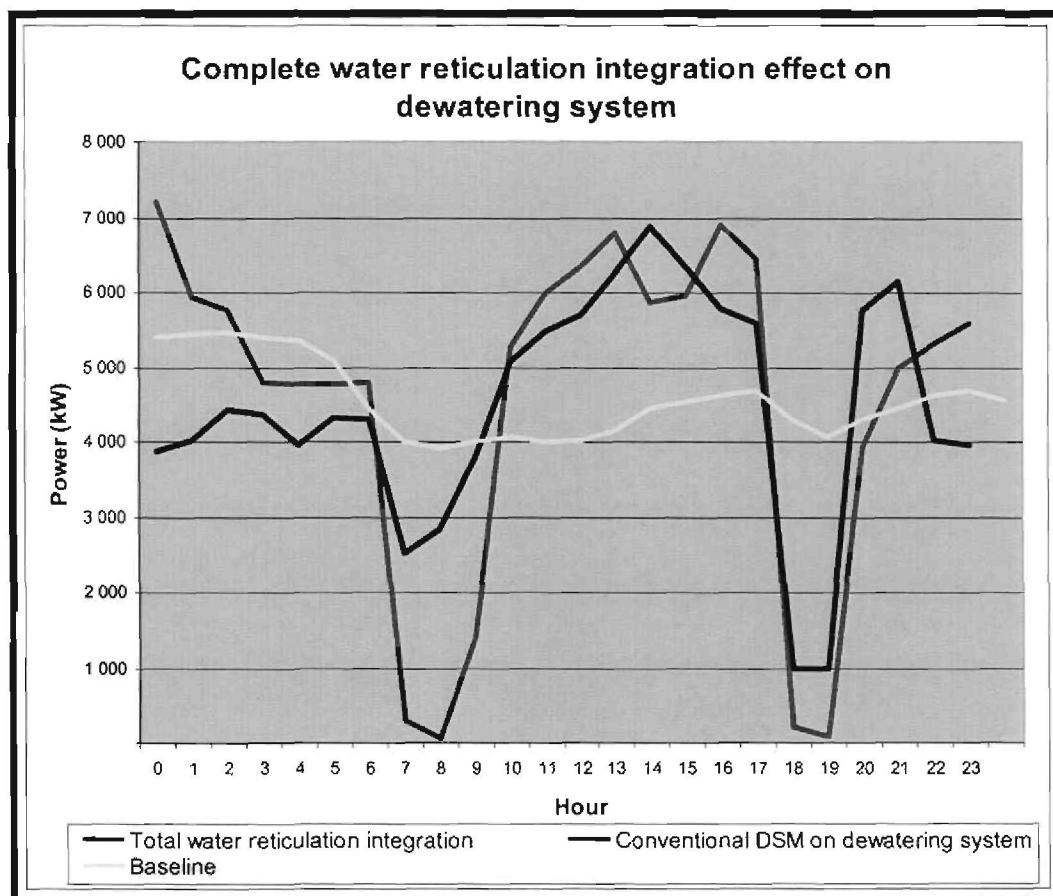
Figure 83: Optimised electricity profile of the dewatering system
