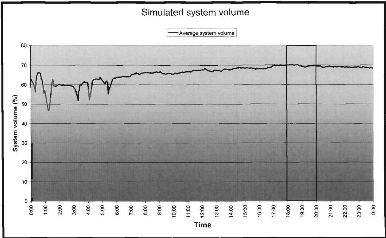
Figure 76: Simulated system volume
