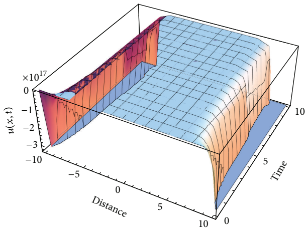
FIGURE 4: We present in Table I the numerical values of the approximate solutions obtained via both methods for different values of alpha.
