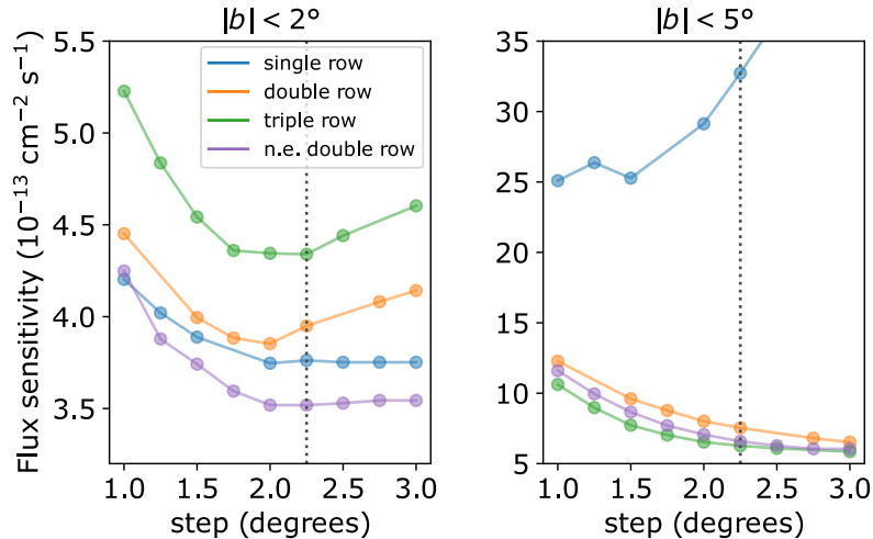
Figure 3. Integral flux sensitivity to an isolated point-like source at energies E > 125 \text{ GeV} averaged over two latitude bands |b| < 2^\circ and |b| < 5^\circ for observations with the southern array at 40^\circ zenith angle. We assume an observing time of 6.5 hours per degree in longitude. The dashed line highlights the step chosen for the non-equilateral double row pattern used in the rest of the paper.
