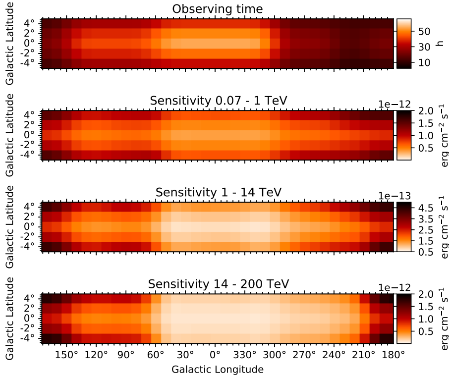
Figure 4. Top panel: observing time as a function of position in the sky, including all observations at an offset < 5^\circ for a given direction. Other panels: sensitivity to a point-like source with power-law spectrum of index 2.34 in three energy bands. The sensitivity is defined as the minimum energy flux integrated over the energy range of interest to achieve a 5\sigma detection. The sensitivity estimates assume that the longitude range 210^\circ - 60^\circ is observed using the southern array, the rest of the plane using the northern array.
