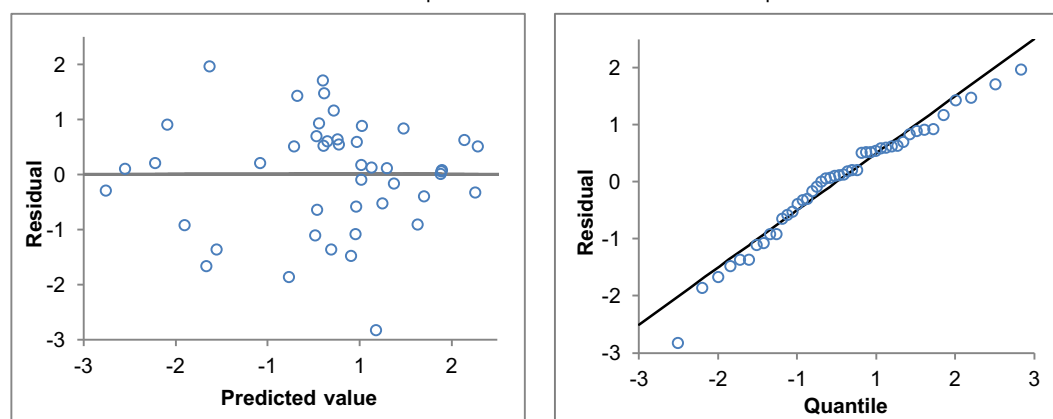
Figure 6 Dataset H's stepwise and forward models' residual plot
