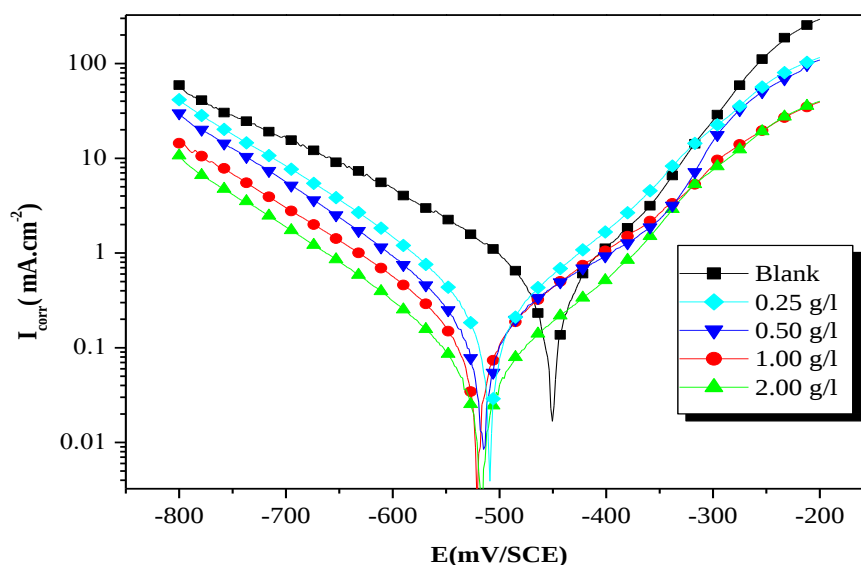
Figure 1. The PDP curves of CS in 1M HCl containing different concentrations of GTE at 298K
