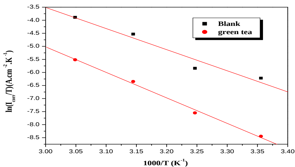
Figure 7. Relation between \ln(I_{\text{corr}}/T) and 1000/T at different temperatures.
