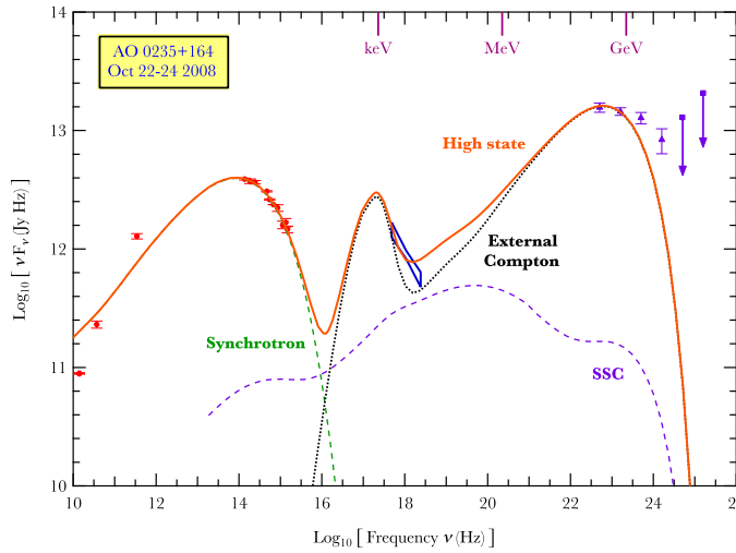
Figure 2: Fit to the SED of the LBL AO 0235+164 (data from [2]), with \eta_1 = 225 and \alpha = 3 . Note that the soft X-ray excess is reproduced by the bulk Compton emission of the thermal electron population. From [3].
