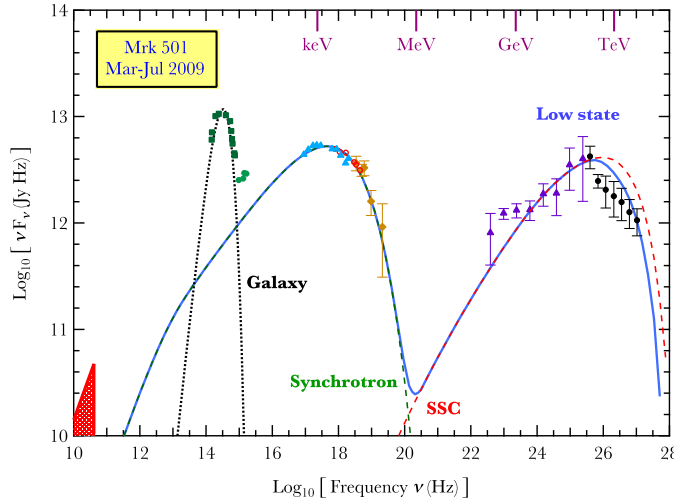
Figure 1: Fit to the SED of the HBL Mrk 501 (data from [1]), with \eta_1 = 100 and \alpha = 1.5 . From [3].
