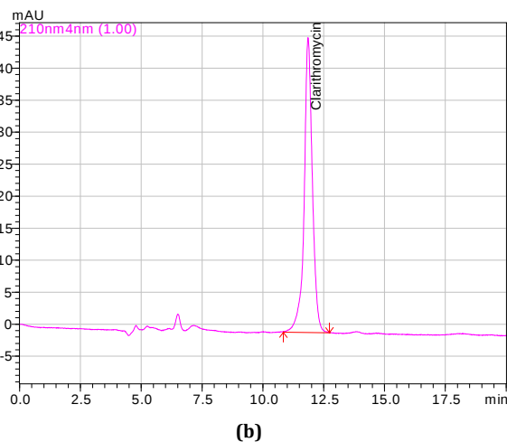
Fig. 2: Chromatograms obtained for clarithromycin during specificity testing with chromatogram (a) showing the peak obtained for clarithromycin from a standard solution and (b) showing the peak obtained for clarithromycin detected from a commercial sample
