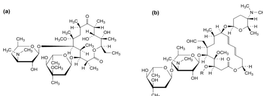
Fig. 1: Molecular structure of (a) clarithromycin and (b) spiramycin [8]
