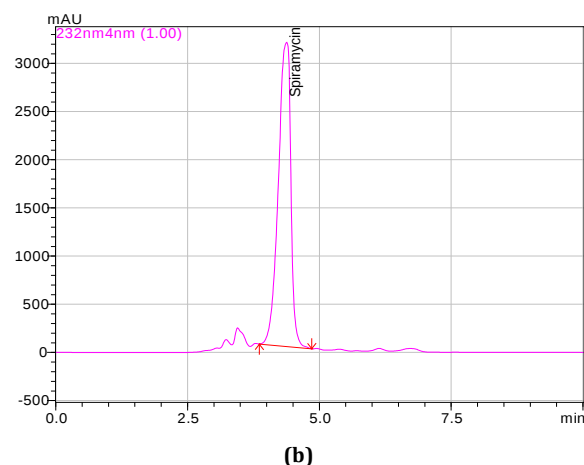
Fig. 3: Chromatograms obtained for spiramycin during specificity testing with chromatogram (a) showing the peak obtained for spiramycin from a standard solution and (b) showing the peak obtained for spiramycin detected from a commercial sample
