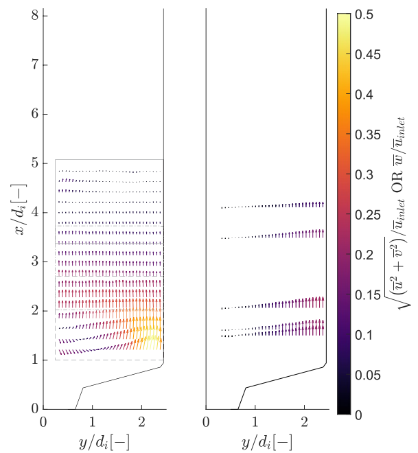
(a) Velocity magnitude of radial and axial velocity in a vertical plane. Each UIV measurement domain is shown with a grey box with a distinctive line pattern. (b) Tangential velocity in multiple horizontal lines, depicting the legend for both subplots at the side.
