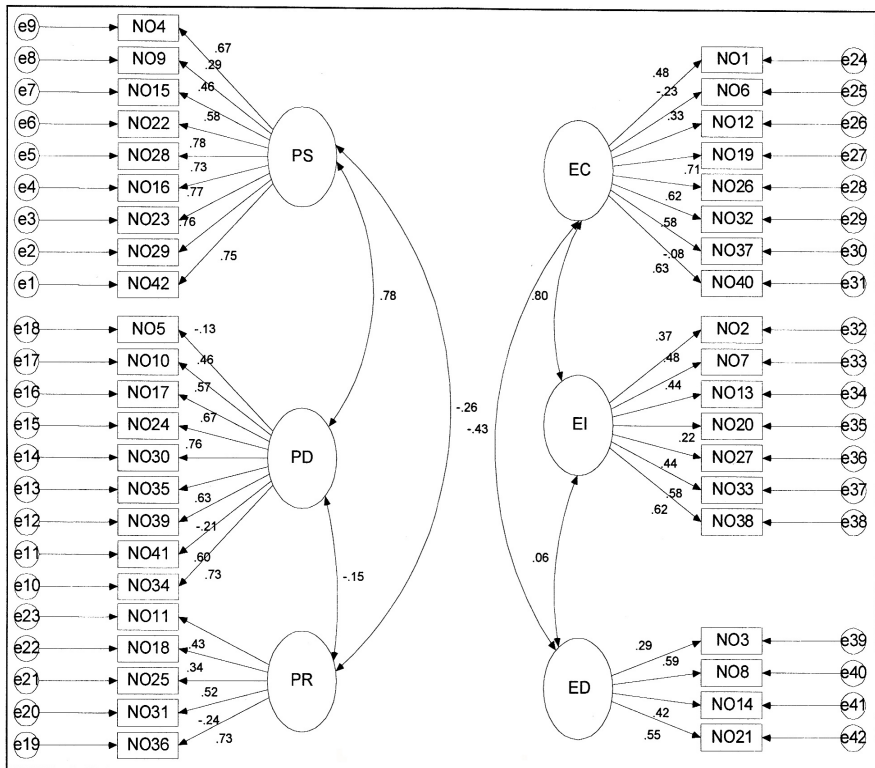
Figure 1 Confirmatory factor analysis of the six factors of the original OCDQ-RE questionnaire
