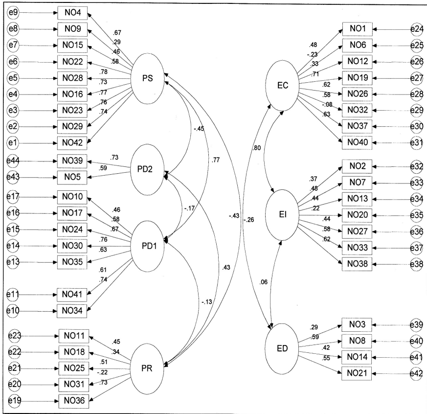
Figure 2 Confirmatory factor analysis with the partition of directive behaviour of the principal
