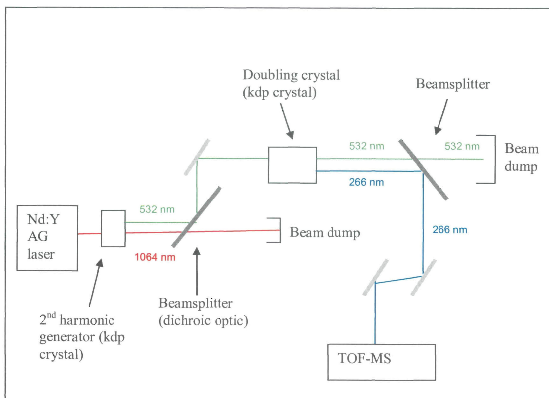
Figure 6.3: Schematic diagram showing the doubling and the quadrupling of the frequency of the Nd:YAG laser beam
