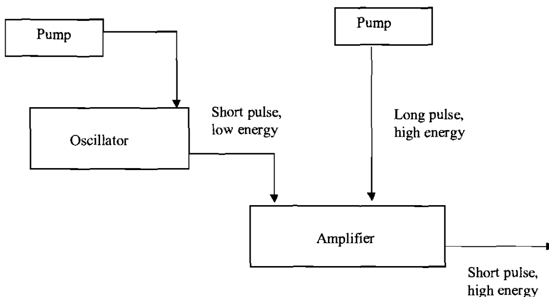
Figure 3.13: Schematic diagram of femtosecond laser system.
