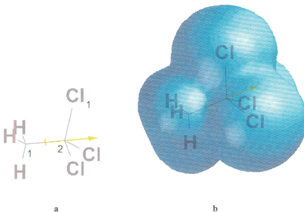
Figure 2.4: (a) Direction of dipole moment (yellow arrow) for TCE and (b) dipole vector with electron density
