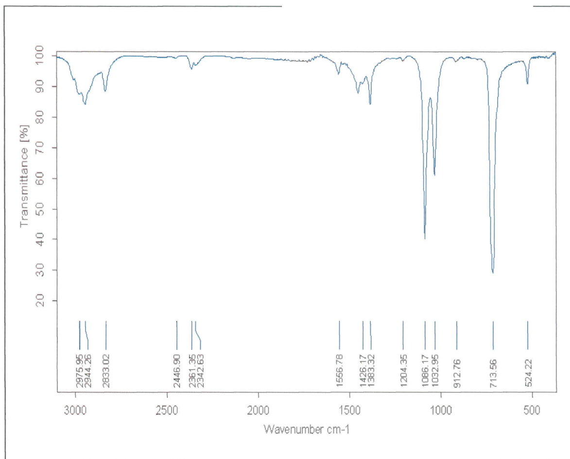
Figure 2.3: FTIR spectrum for liquid TCE measured on Bruker's VERTEX 70 FTIR spectrometer coupled to RAM II FT-Raman module
