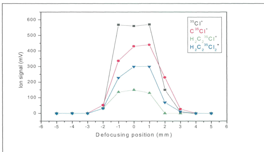
Figure 6.11: Graph showing the effect of defocusing of the lens on selected ion signals. This data is obtained by observing mass peak signals and varying the focus position with nanosecond laser pulses of 266 nm, 6 ns and 2.9 mJ
