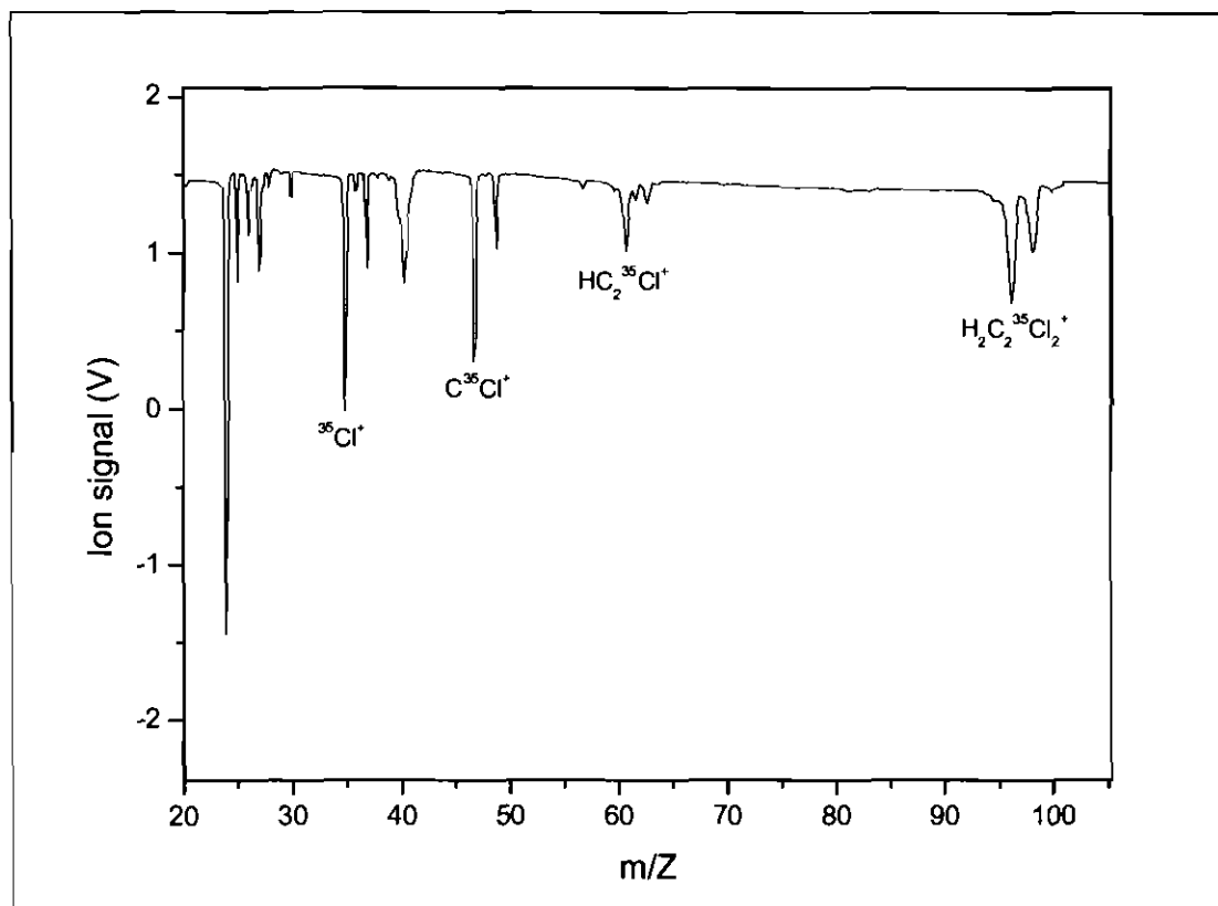
Figure 6.9: Time of flight mass spectrum of TCE using nanosecond laser ionization at 266 nm, 6 ns and 2.9 mJ pulses showing the selected peaks for optimization of TOF system
