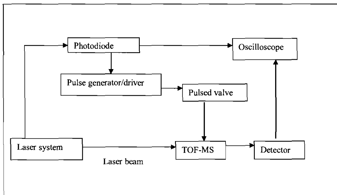
Figure 6.5: Schematic diagram of the timing in the experimental setup for the femtosecond laser system
