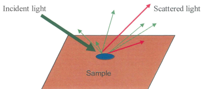
Figure 3.3: Schematic representation of the Raman scattering principle (Red arrows: Raman scattering and bright green arrows: Rayleigh scatter) [ http://www.andor.com , 28 March 2007]
