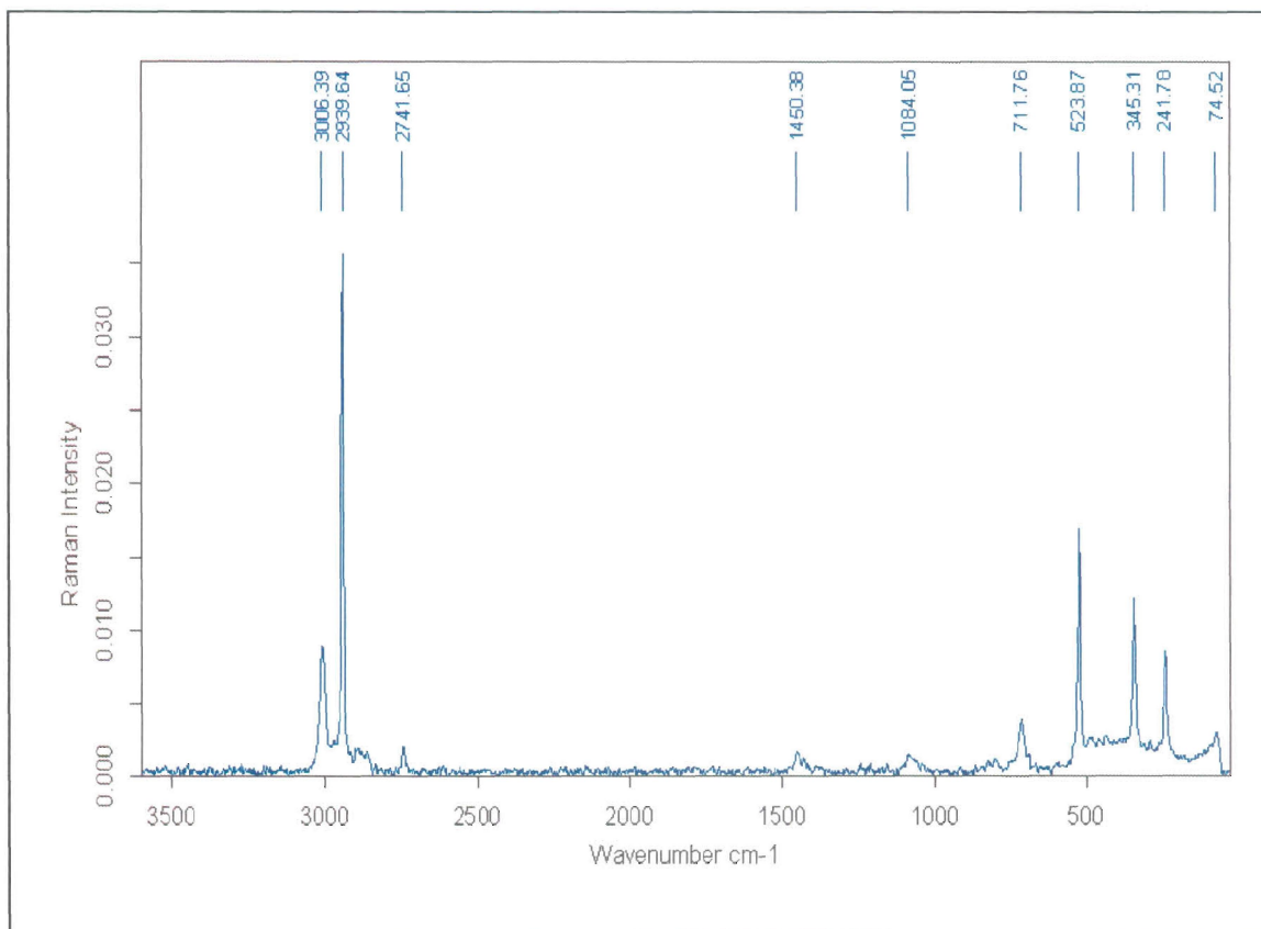
Figure 5.2: Experimental FT-Raman spectrum of TCE in liquid phase
