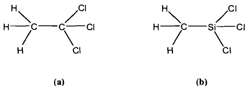
Figure 1.1: Molecular structure for (a) TCE and (b) MTS
