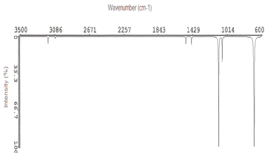
Figure 2.2: Calculated FTIR spectrum for TCE with B3LYP/6-31G* method
