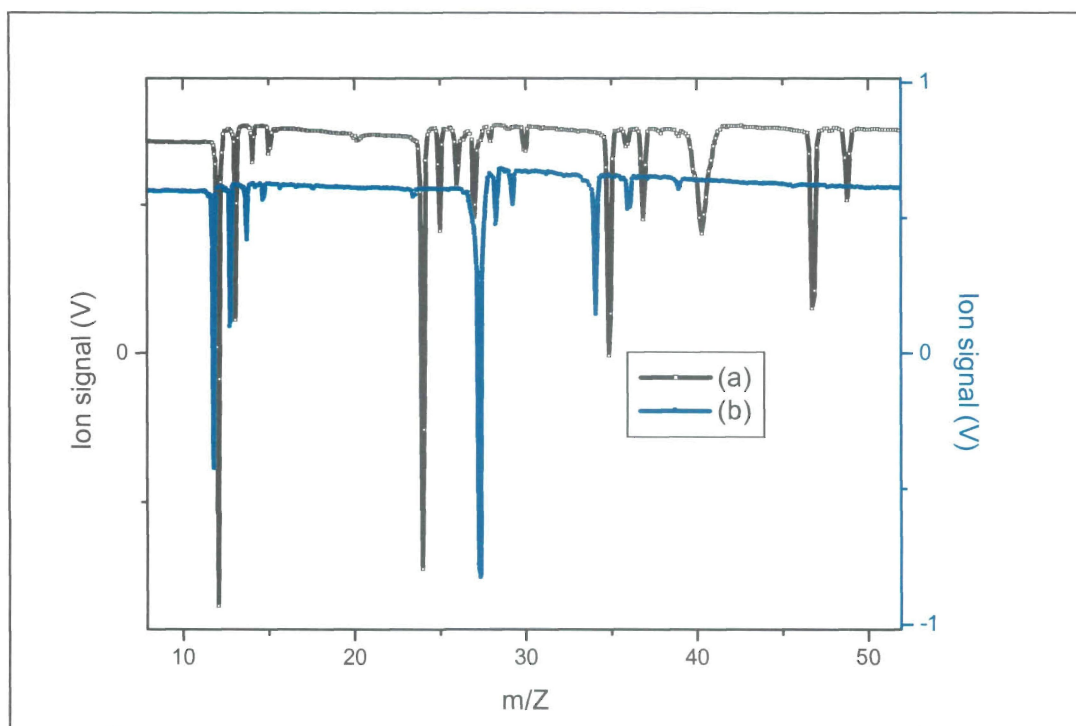
Figure 6.24: Expanded laser photoionization mass spectra of (a) TCE and (b) MTS using nanosecond laser at 266 nm, 6 ns, and 2.9 mJ pulses
