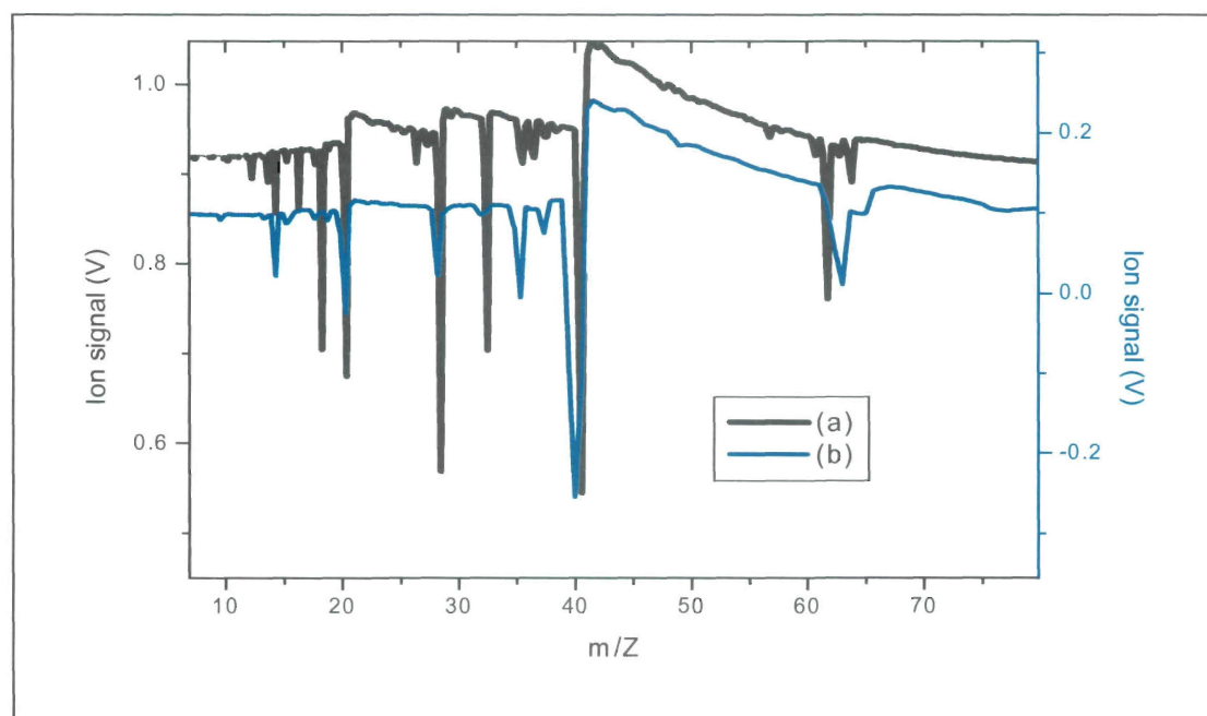
Figure 6.21: Laser photoionization mass spectra of (a) TCE and (b) MTS using femtosecond laser at 795 nm, 120 fs, and 1 mJ pulses
