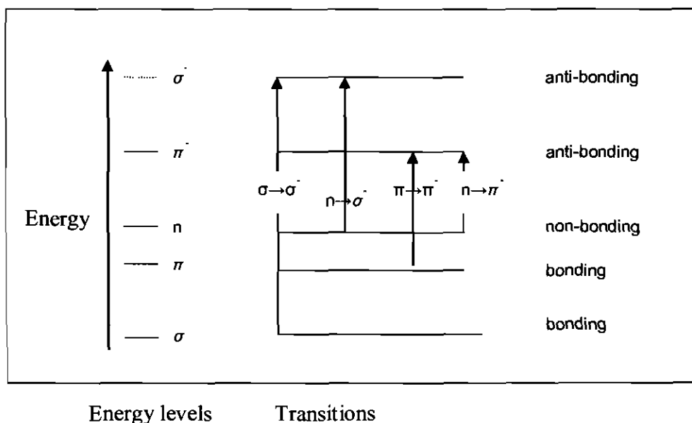
Figure 3.6: Energy level diagram showing transitions involving \pi , \sigma and n electrons [Skoog et al. , 1998]
