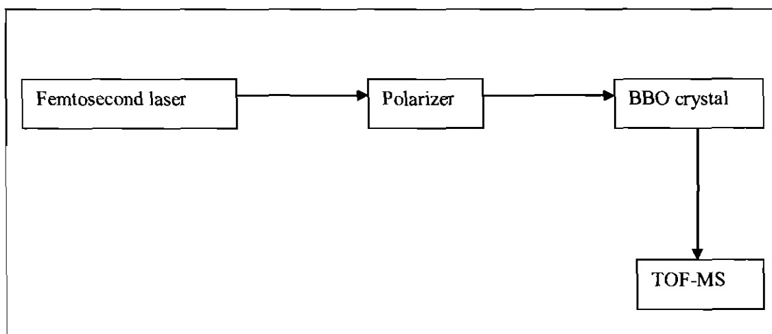
Figure 6.6: Schematic diagram showing the experimental setup for the time of flight using femtosecond laser beam for ionization of TCE
