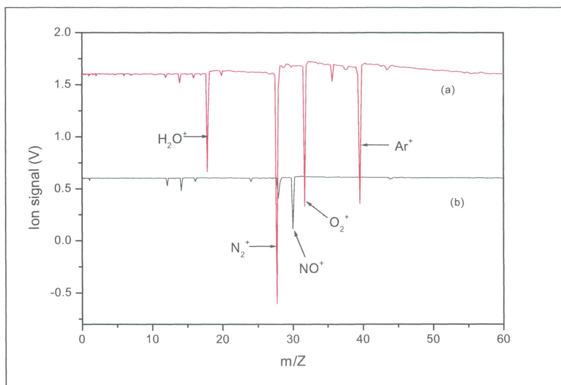
Figure 6.8: Measured time of flight mass spectra of \text{N}_2\text{O} gas (a) using femtosecond laser at 795 nm, 120 fs, 1 mJ and (b) nanosecond laser at 266 nm, 6 ns, and 2.9 mJ pulses
