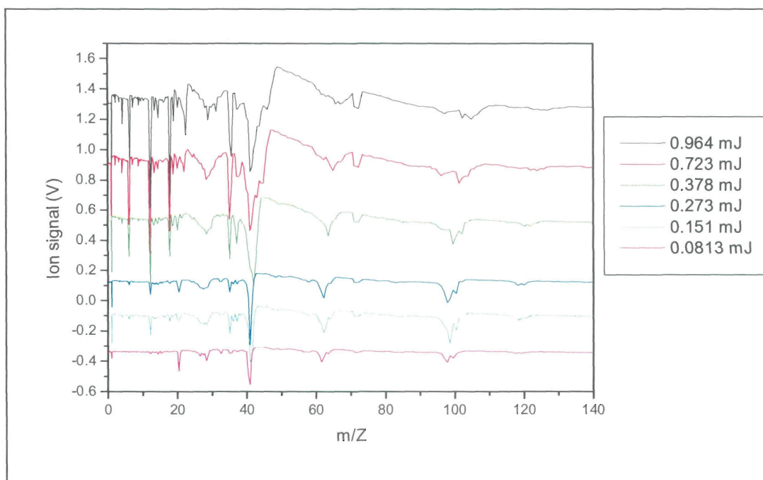
Figure 6.17: Laser photoionization time of flight mass spectra of TCE using femtosecond laser pulses at 795 nm with different laser energies
