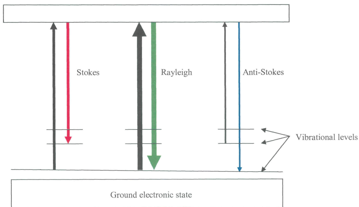
Figure 3.4: Schematic representation of the energy levels of Raman and Rayleigh scattering. Raman scattering takes place to the longer wavelengths (Stokes Raman scattering) and shorter wavelengths (anti-Stokes Raman scattering) [http://www.raman.de, 16 April 2007]
