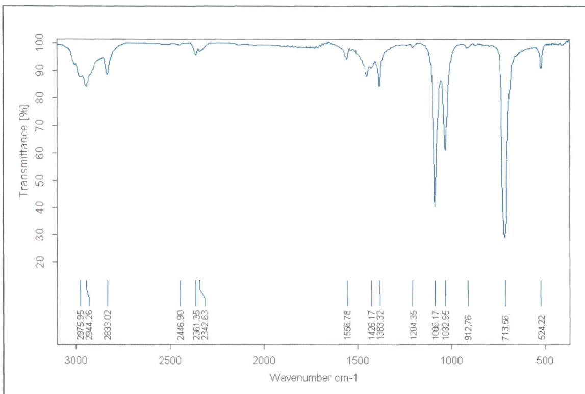
Figure 5.1: Experimental FTIR spectrum of TCE in liquid phase
