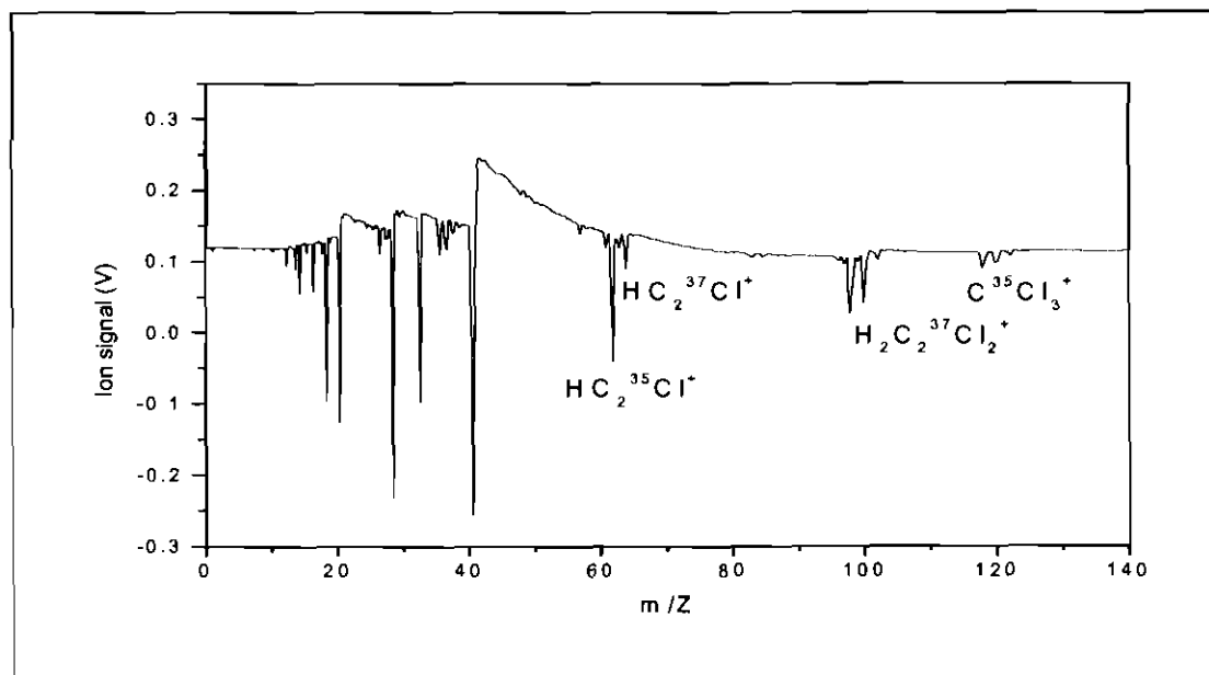
Figure 6.16: Laser photoionization time of flight mass spectrum of TCE using the femtosecond laser with 795 nm, 120 fs, 1 mJ pulses
