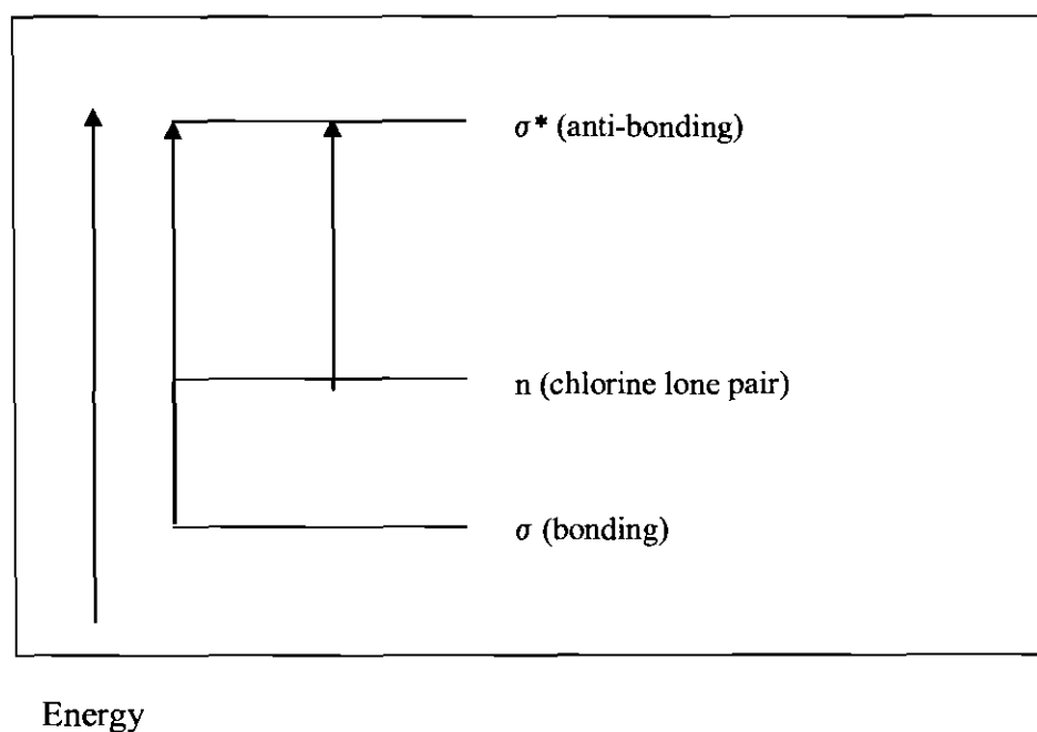
Figure 5.4: Assumed UV energy diagram for TCE (not to scale)
