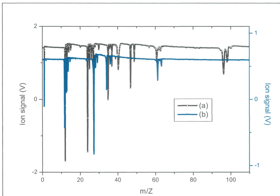
Figure 6.23: Laser photoionization mass spectra of (a) TCE and (b) MTS using nanosecond laser at 266 nm, 6 ns, and 2.9 mJ pulses
