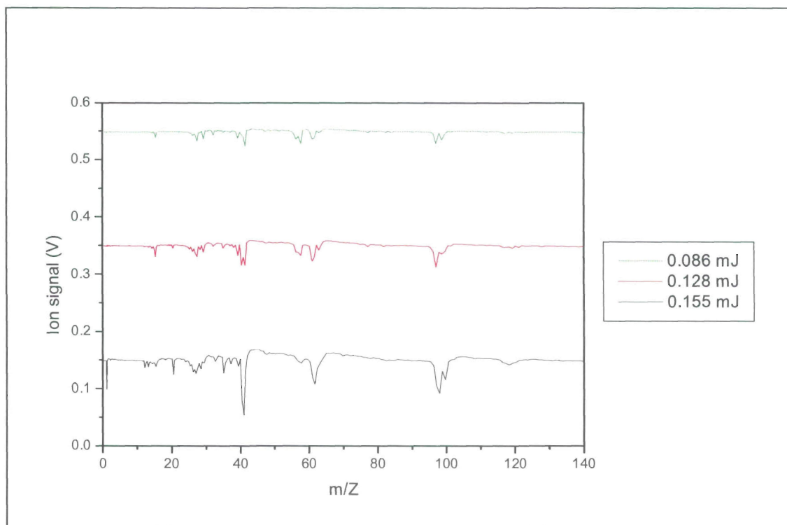
Figure 6.18: Laser photoionization time of flight mass spectra of TCE with femtosecond laser pulses at 397.5 nm and different laser energy
