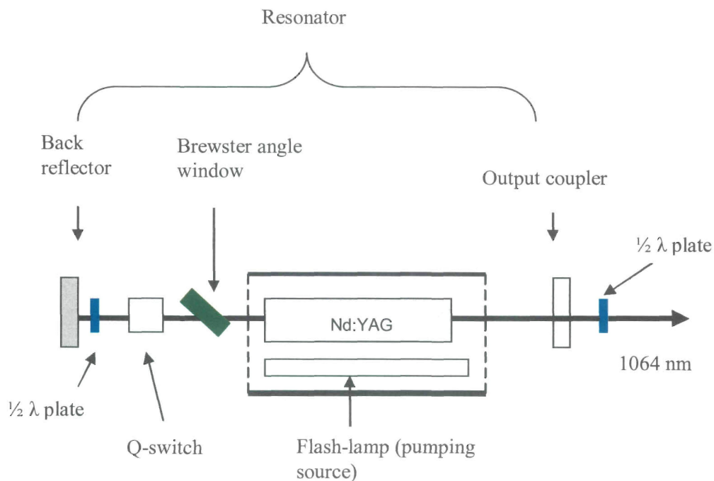
Figure 3.8: Schematic diagram of Nd:YAG laser [Telle et al. , 2007]
