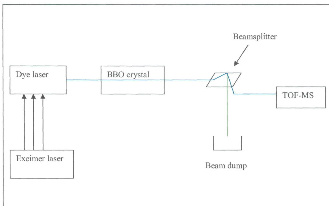
Figure 6.4: Schematic diagram showing the doubling of the frequency of the dye laser beam
