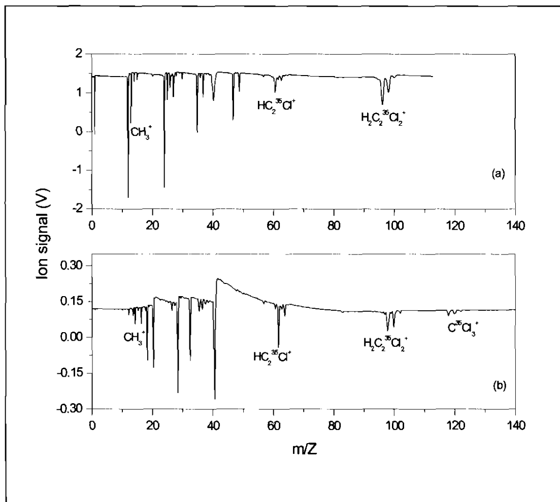
Figure 6.20: Laser photoionization mass spectra of TCE (a) using nanosecond laser at 266 nm, 6 ns, 2.9 mJ pulses, and (b) using femtosecond laser at 795 nm, 120 fs and 1 mJ pulses
