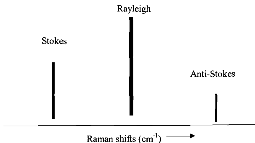
Figure 3.5: Comparison of intensities of lines in a Raman spectrum [http://www.andor.com, 28 March 2007]
