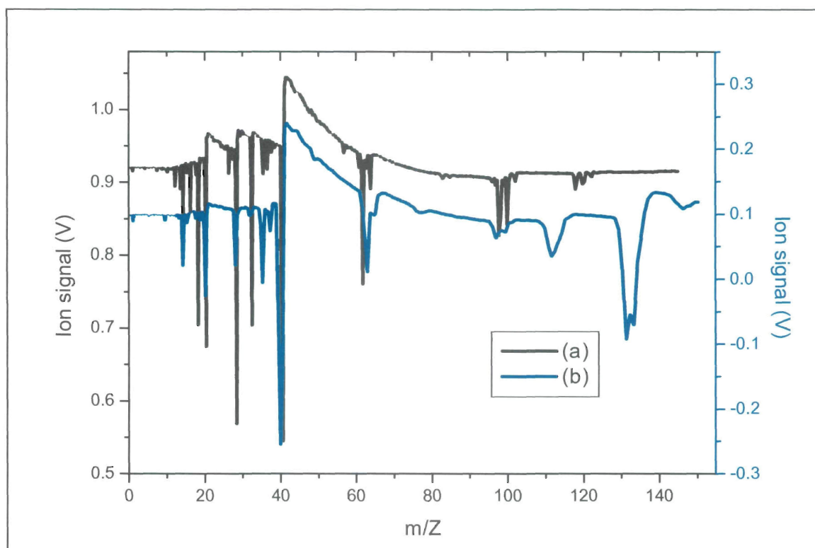
Figure 6.21: Laser photoionization mass spectra of (a) TCE and (b) MTS using femtosecond laser at 795 nm, 120 fs, and 1 mJ pulses
