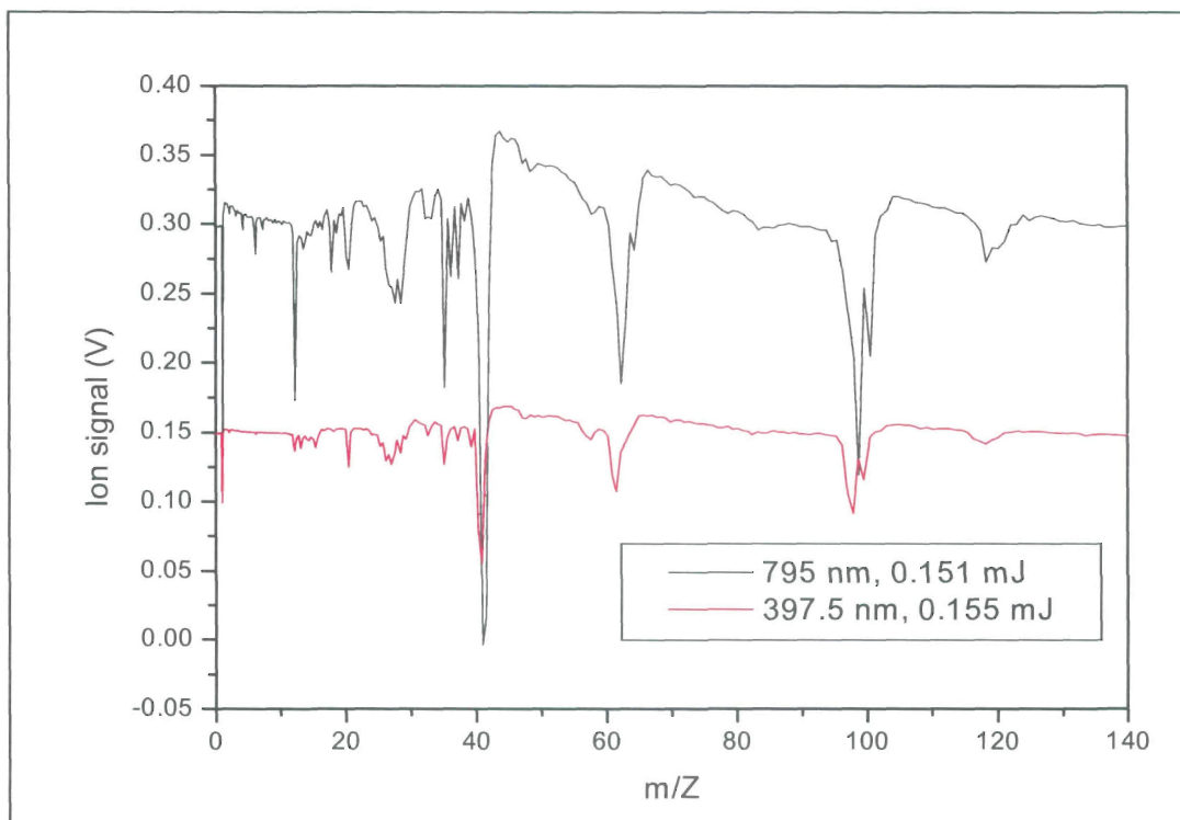
Figure 6.19: Laser photoionization time of flight mass spectra of TCE with femtosecond laser at 795 nm, 0.151 mJ and 397.5 nm, 0.155 mJ pulses
