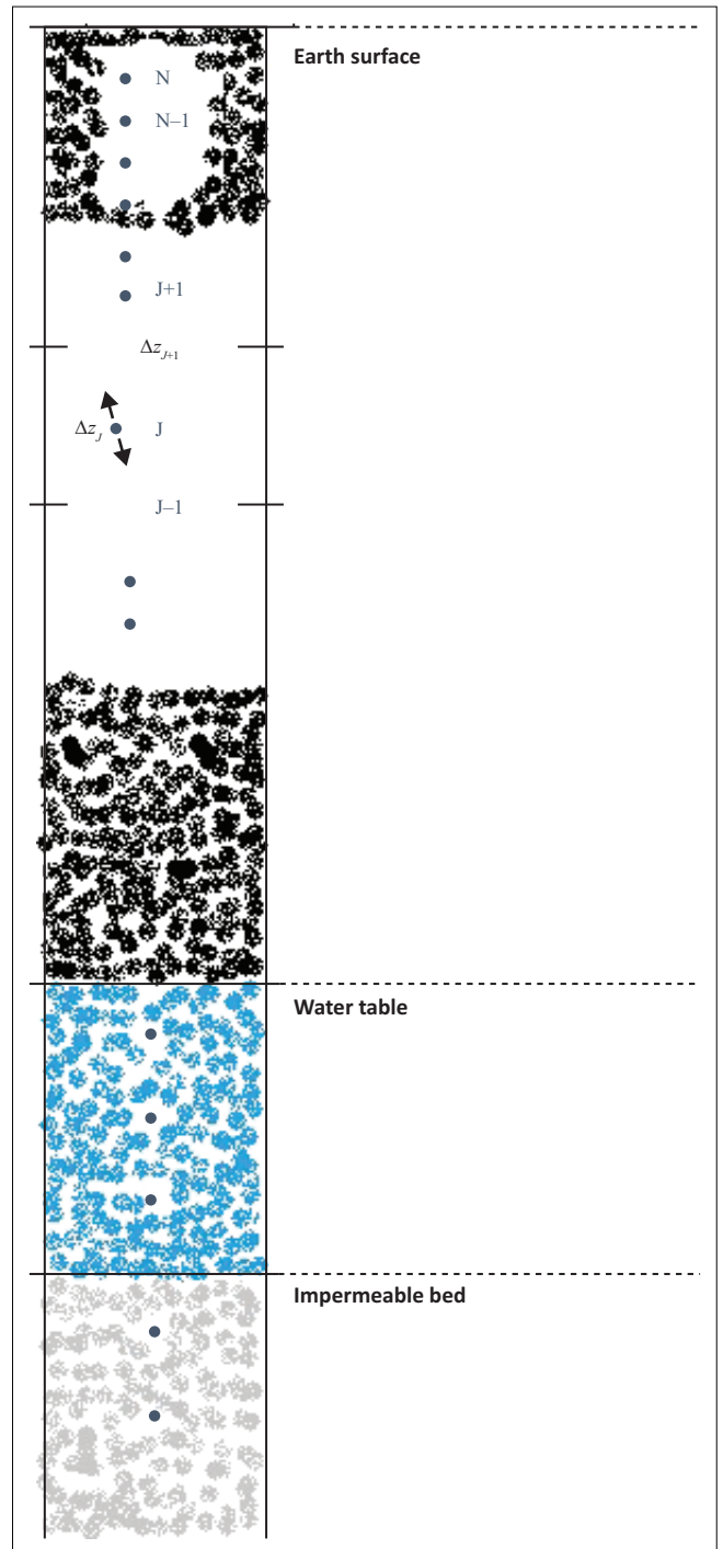
FIGURE 1: Vertical discretisation of a soil profile.
