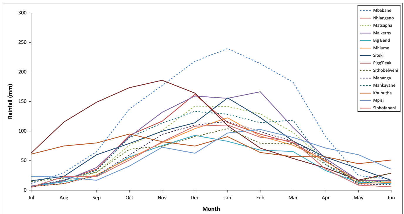
FIGURE 2: Mean historical monthly rainfall for Eswatini during the time period 1986–2017.
