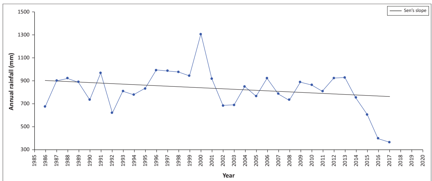
FIGURE 3: Annual rainfall trend for Eswatini (1986–2017).
