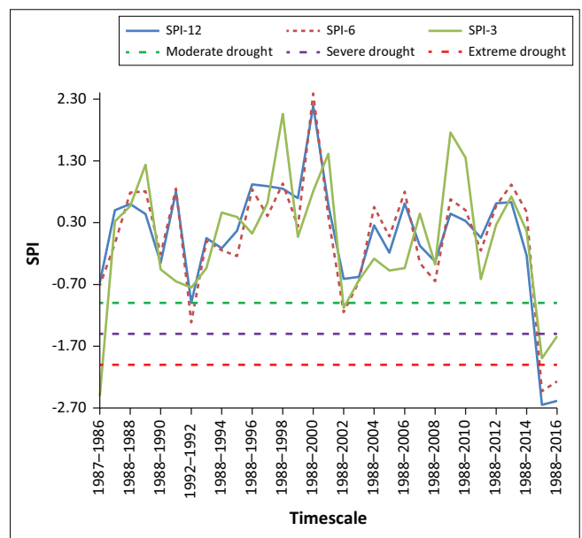
FIGURE 4: Standard Precipitation Index values of Eswatini for three different timescales (3, 6 and 12 months).
