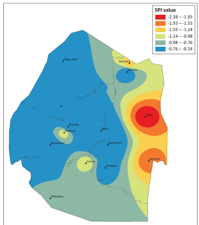
FIGURE 6: Standard Precipitation Index 3-month timescale during 1985–1986.
