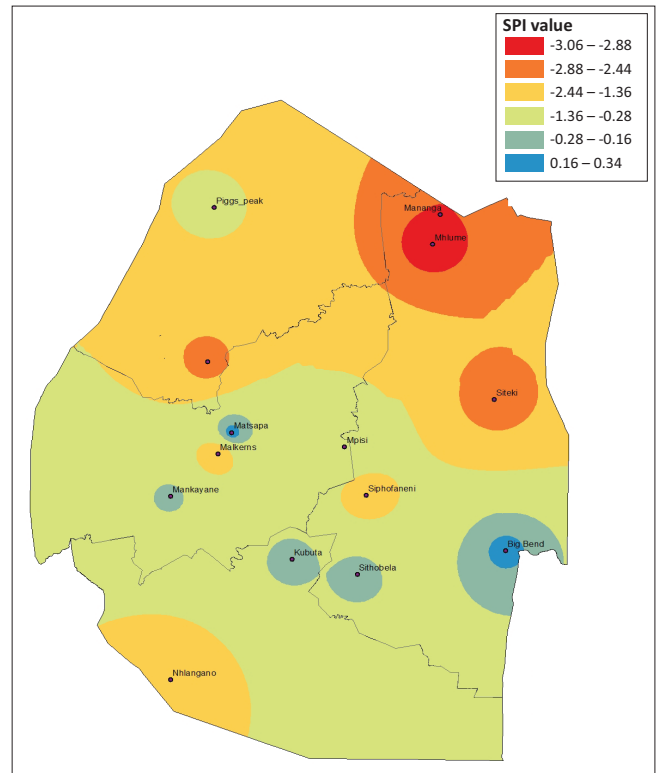
FIGURE 9: Standard Precipitation Index 3-month timescale during 2015–2016.
