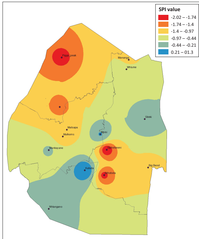
FIGURE 7: Standard Precipitation Index 3-month timescale during 2004–2005.
