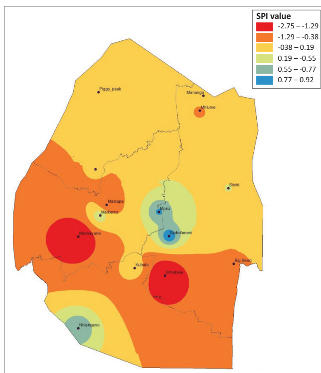
FIGURE 8: Standard Precipitation Index 3-month timescale during 2005–2006.
