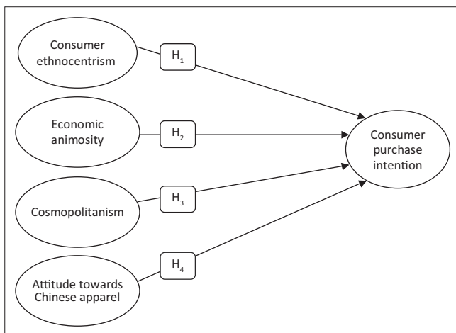
FIGURE 3: Alternative Model 3.
