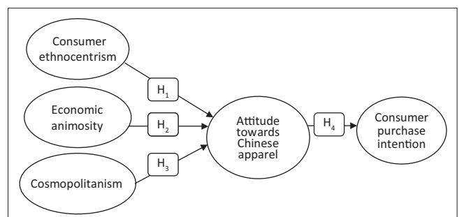
FIGURE 1: Research model 1.
