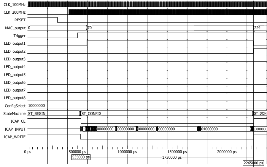
Figure 13: Timing diagram of the second experimental design
