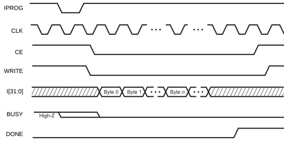
Figure 10: Timing diagram for ICAP data loading
