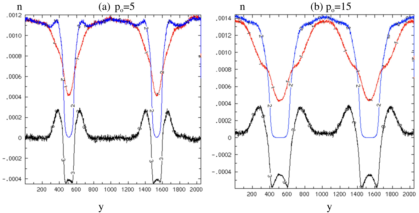
Figure 4. Comparison of density profiles n vs. y (averaged over x ) between the p_o = 5 and p_o = 15 cases at t\omega_e = 8000 . Curve 1 (red): electrons, Curve 2 (blue): ions, Curve 3 (black): net charge ( =n_i - n_e ). These density profiles highlight the persistence of the ion vacuum gap, which is wider for the p_o = 15 case than the p_o = 5 case, scaling as \sim p_o . Electrons, however, are not fully evacuated from the boundary interface, leading to the formation of the charge triple layer (double capacitor), which plays an important role in electron energization.
