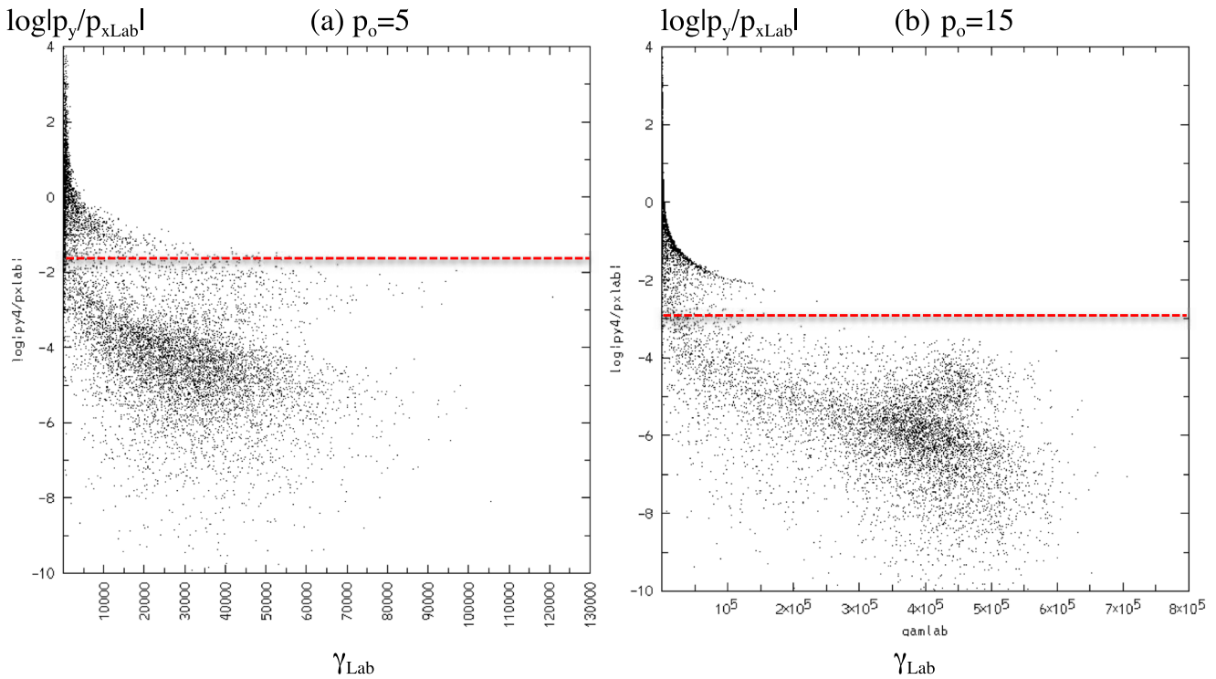
Figure 8. Distribution of the tangent of the “beam angle” ( =|p_y/p_{xLab}| ) of spine electrons vs. Lorentz factor \gamma_{Lab} in the “laboratory frame” at t\omega_c = 8000 for (a) p_o = 5 and (b) p_o = 15 . We see that in both cases all of the high-energy spine electrons (i.e., those that did not cross over to the sheath and get decelerated) have beam angles much smaller than 1/\Gamma (red dashed lines). In both cases, there exists an exponential anti-correlation between beam angle and electron energy, which may be tested with future observations.
