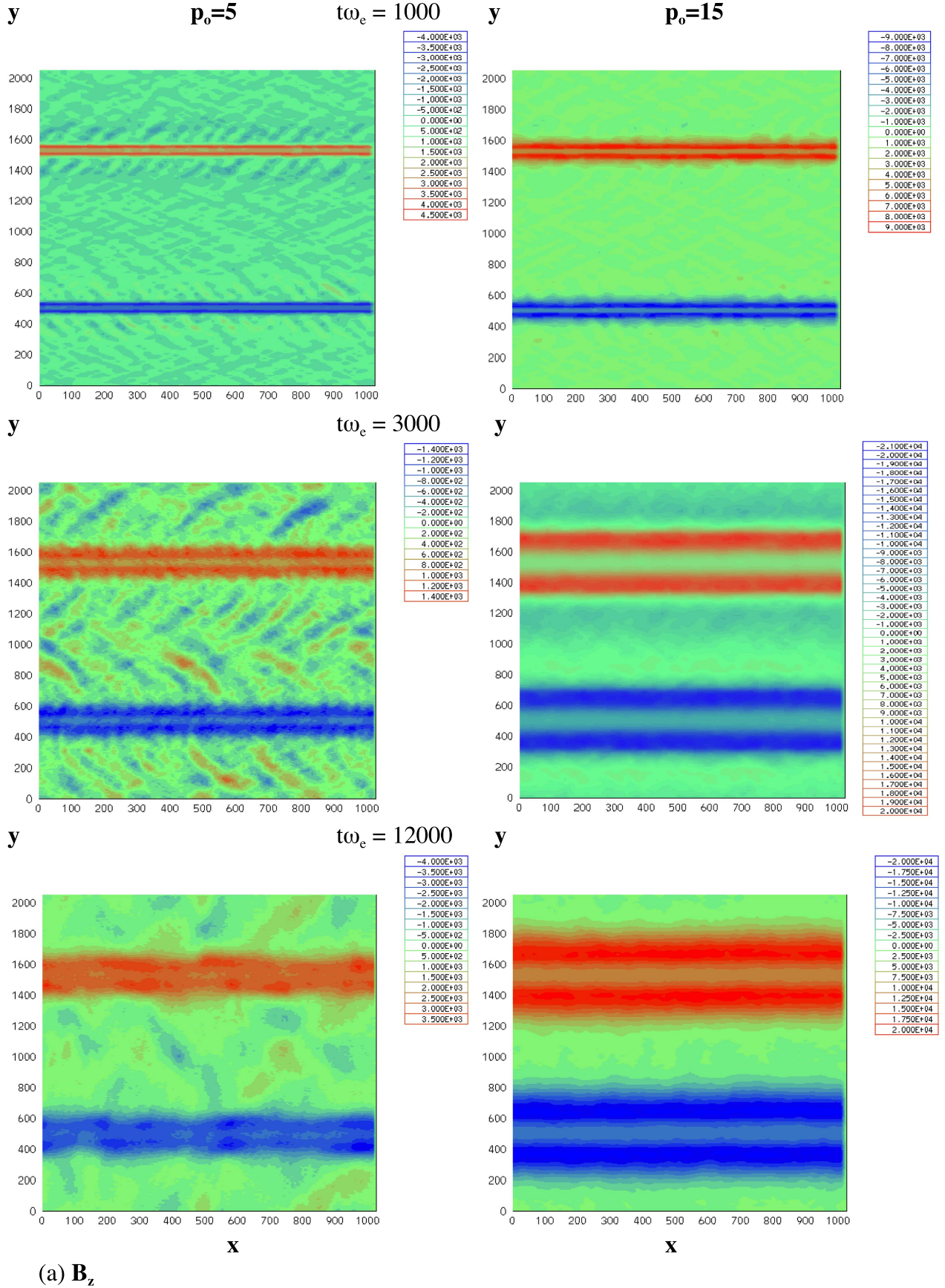
Figure 3. Comparison of spatial profiles of (a) B_z , (b) E_y , (c) E_x , (d) j_x , (e) \rho = \text{net charge} = (n_i - n_e) , between p_0 = 5 (left columns) and p_0 = 15 (right columns) cases at three different times: t\omega_e = 1000 (top), 3000 (middle), 12,000 (bottom). We note that the average shear boundary layer thickness of the p_0 = 5 case is \sim 1/3 that of the p_0 = 15 case, scaling roughly as \sim p_0 . The maximum B_z , E_y fields at t\omega_e = 12000 of the p_0 = 5 case is lower than those of the p_0 = 15 case, scaling roughly as p_0^{3/2} .
