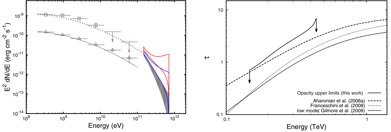
Fig. 4. HE and VHE spectra of PKS 1510–089 measured with Fermi -LAT and H.E.S.S., and upper limits on the EBL induced opacity. Left: the filled butterfly shows the H.E.S.S. spectrum as a 1\sigma confidence band; the blue and red butterflies shows the spectrum corrected for EBL absorption, using the low model for the EBL from Gilmore et al. (2009) and the upper-limit EBL model from Aharonian et al. (2006a) respectively. The triangles show the long-term average Fermi -LAT spectrum, with error bars denoting 1\sigma statistical errors; the solid curve is the log-parabola model obtained from a binned likelihood analysis of these data (see text for details). The open squares show the Fermi -LAT spectrum derived from the integration period between MJD 54 914.8 and MJD 54 917.5 (error bars illustrate 1\sigma statistical errors). Arrows denote upper limits on the flux for those bins where insufficient statistics prohibits a flux measurement. The dashed curve is obtained by re-normalizing the long-term average Fermi -LAT spectrum to the level of the high-flux state. Right: upper limits on the EBL opacity derived from spectral measurements of PKS 1510–089 compared to published models. The solid line with arrows at both ends shows the maximum optical depth, corresponding to upper limits on the EBL. For comparison the opacity corresponding to the previously published H.E.S.S. upper-limit EBL model Aharonian et al. (2006a), the Franceschini et al. (2008) model and the low model from Gilmore et al. (2009) are shown.
