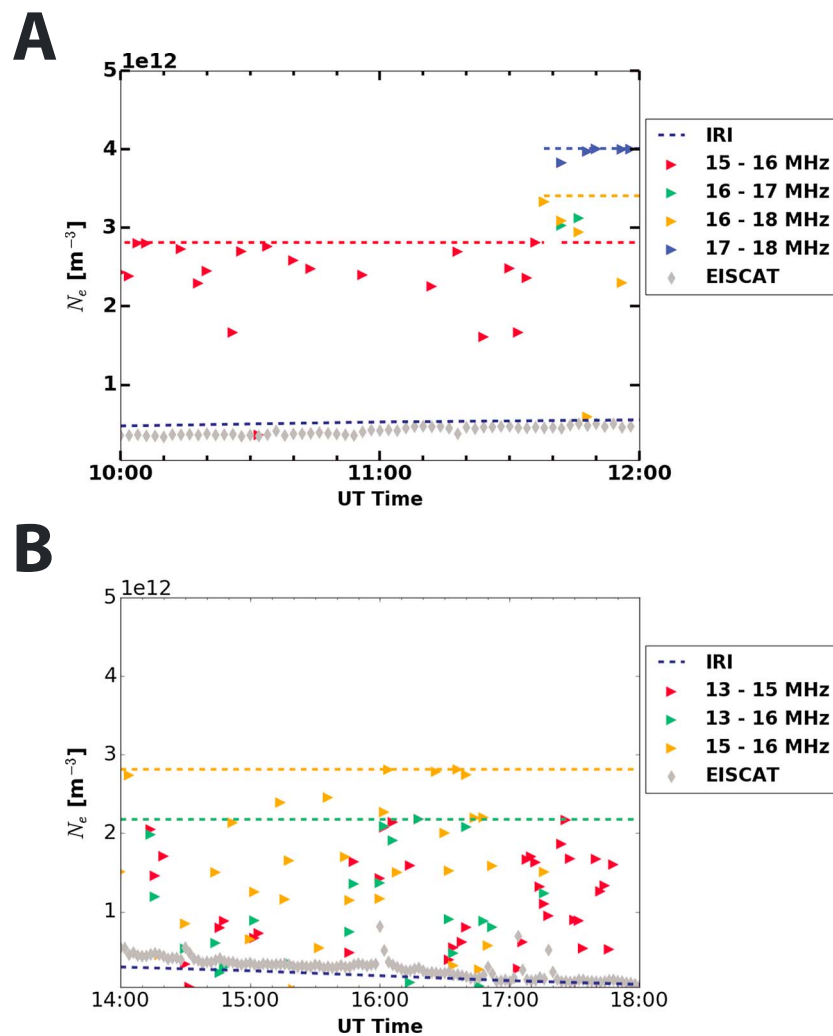
Figure 5. The colored triangles are the calculated N_e from the Hankasalmi STEREO observations for (a) 12 March 2015 from 10:00 to 12:00 UT and (b) 3 March 2016 from 14:00 to 18:00 UT. The shaded diamonds are the EISCAT N_e at 240 km for Figure 5a and 220 km for Figure 5b. The navy blue dotted line is IRI N_e at 240 km for Figure 5a and 220 km for Figure 5b. The dashed lines are the maximum electron number density possible in regard to plasma frequency. The color of the triangles and dashed lines indicate what frequency pairs were used to calculate N_e . In Figure 5a the green line is under the yellow one and in Figure 5b the red line is under the green one.
