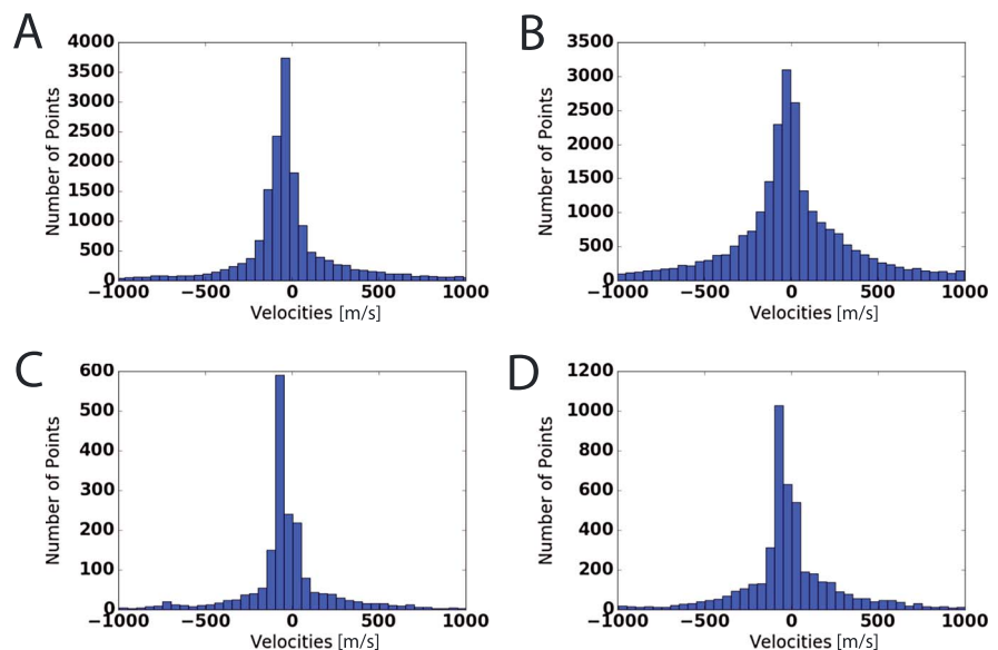
Figure 2. Velocity distributions of each of the major frequency bands from the Hankasalmi radar. (a) 15 MHz, (b) 16 MHz, (c) 17 MHz, and (d) 18 MHz for the campaign on 12 March 2015 from 10:00 to 12:00 UT.
