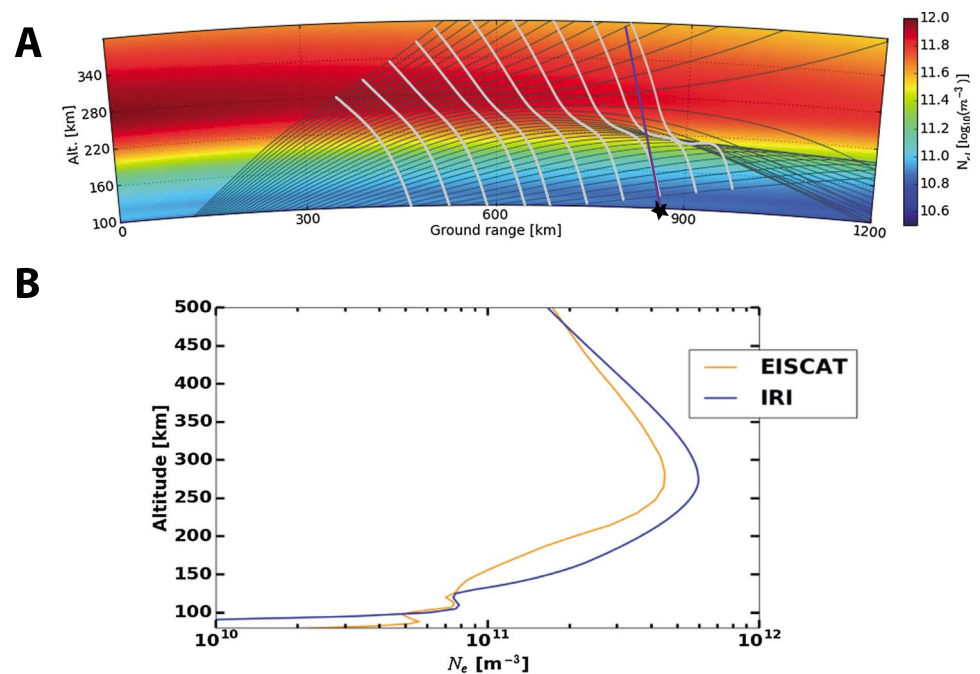
Figure 3. (a) The SuperDARN ray tracing model output for our experiment at 16 MHz for beam 5 on 12 March 2015. The radar-beam elevation angle ranges between 5 and 40°, with 2° increments represented by the black lines. The silver lines are every fourth range gate (approximately 60 km) starting at 480 km (range gate 0). The background is N_e from the IRI model. The black star represents the approximate distance to the EISCAT Tromsø site. The purple line represents the magnetic field line at Tromsø, indicating the look direction of the EISCAT heater. (b) The IRI (blue) and EISCAT (orange) N_e profiles averaged between 10:00 and 12:00 UT on 12 March 2015.
