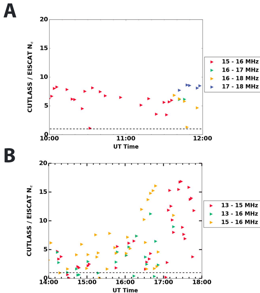
Figure 6. The ratio of N_e calculated from the Hankasalmi and EISCAT radars. The colored triangles are the calculated N_e from the Hankasalmi STEREO method resampled into 2 min periods for (a) 12 March 2015 from 10:00 to 12:00 UT and (b) 13 March 2016 from 14:00 to 18:00 UT and divided by the EISCAT N_e at 240 km for Figure 6a and 220 km for Figure 6b at the same times. The black dotted line is where the Hankasalmi N_e equals the EISCAT N_e . The color of the triangle indicates what frequency pairs were used to calculate N_e . In Figure 6a the green line is under the yellow one and in Figure 6b the red line is under the green one.
