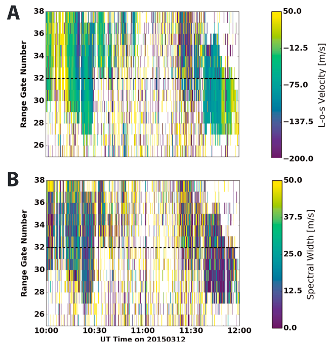
Figure 1. (a) The line-of-sight velocities from the Hankasalmi radar at frequencies of 15 MHz–18 MHz on 12 March 2015 from 10:00 UT to 12:00 UT at range gates of 25 to 38. The range gates start at 480 km and have 15 km spacing from there. EISCAT is located at approximately range gate 32, where we have placed a black dotted line. (b) The spectral widths over the same frequencies and same time period.
