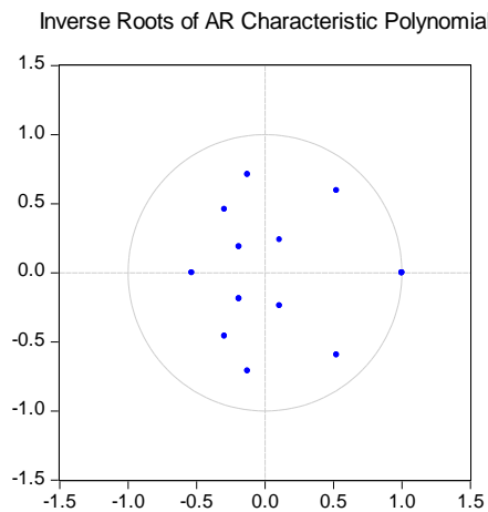
Figure 5.3 Stability test for Equation 4.4
