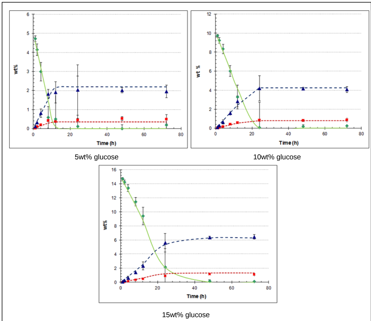
Figure I.1 Comparison of experimental fermentation data without substrate inhibition with substrate-limiting model using different starting sugar concentration and 10g/L yeast ( \diamond Experimental glucose, \blacktriangle Experimental ethanol, \blacksquare Experimental glycerol, — glucose model, --- ethanol model, ... glycerol model)
