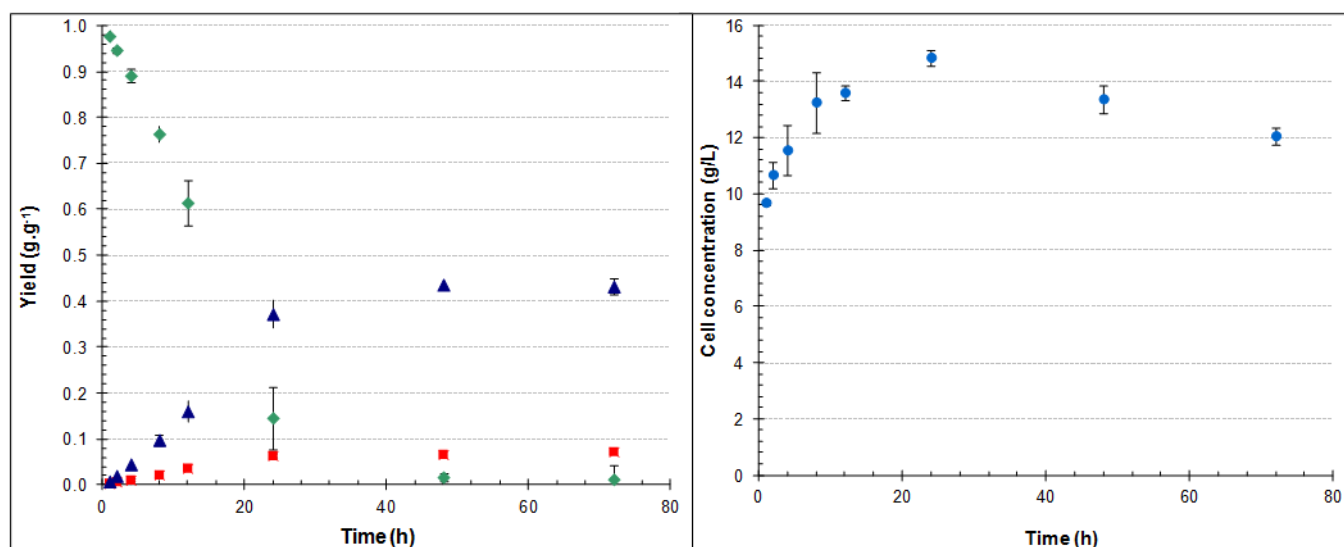
Figure C.16 Fermentation at a pH of 4.5
