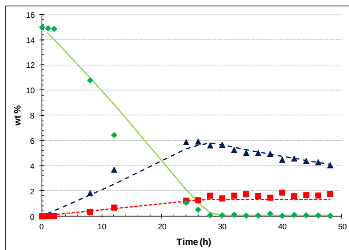
Figure I.8 Comparison of the membrane-reactor system model with experimental data (♦ Experimental glucose, ▲ Experimental ethanol, ■ Experimental glycerol, — glucose model, --- ethanol model, ... glycerol model)
