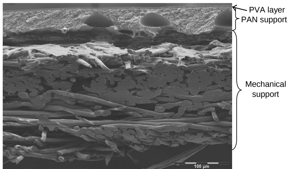
Figure 3.10 SEM image of the PERVAP4101® membrane
