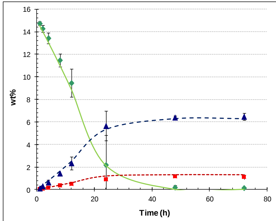
Figure 2.12 Comparison of experimental fermentation with the substrate-limiting model using 15wt% starting glucose and 10g/L starting yeast
