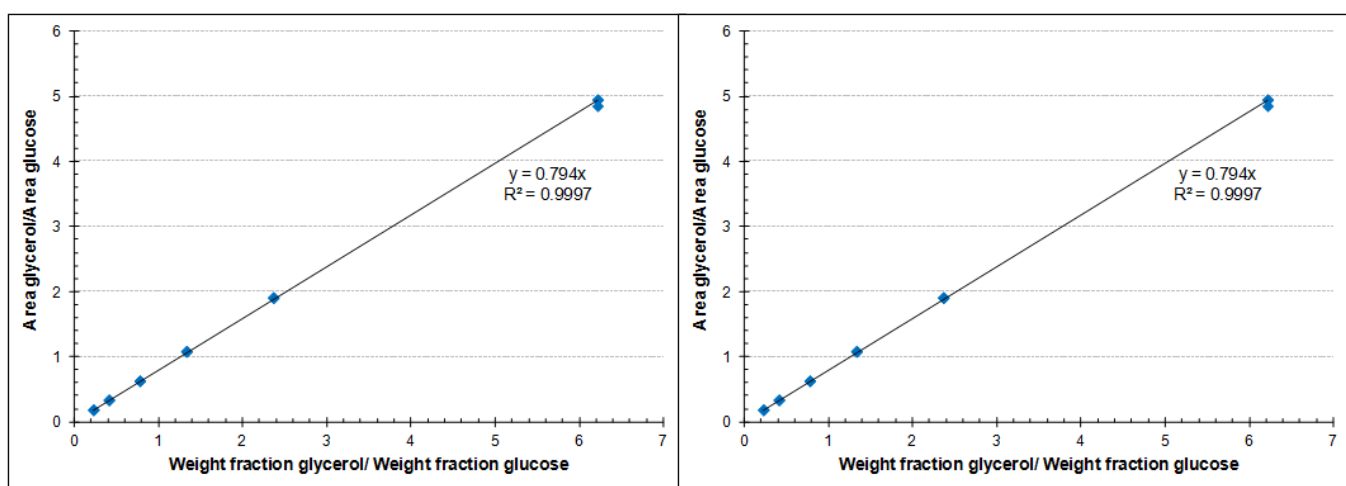
Figure B.4 Glycerol/Glucose calibration curve
