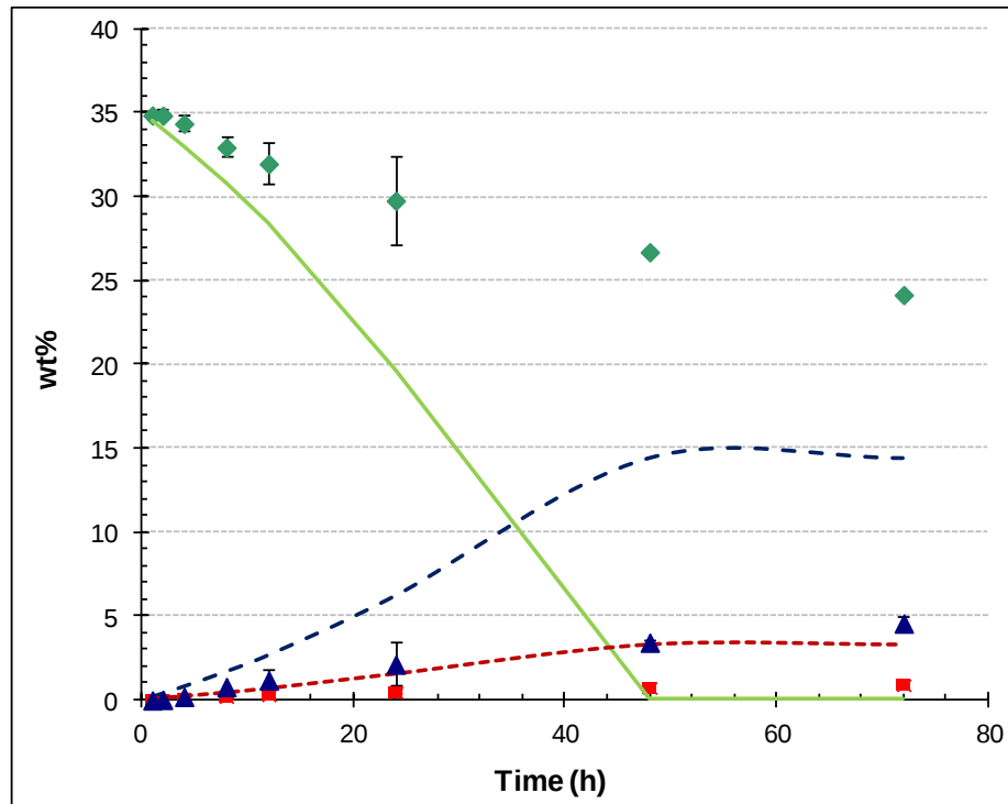
Figure 2.13 Comparison of experimental fermentation with the substrate-limiting model using 35wt% starting glucose and 10g/L starting yeast
