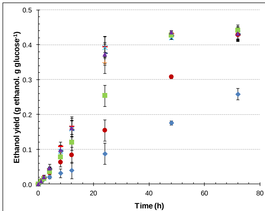
Figure 2.9 Effect of pH on ethanol yield (♦ 2.5, • 3, ■ 3.5, × 4, ▲ 4.5, + 5, − 5.5, X 6)
