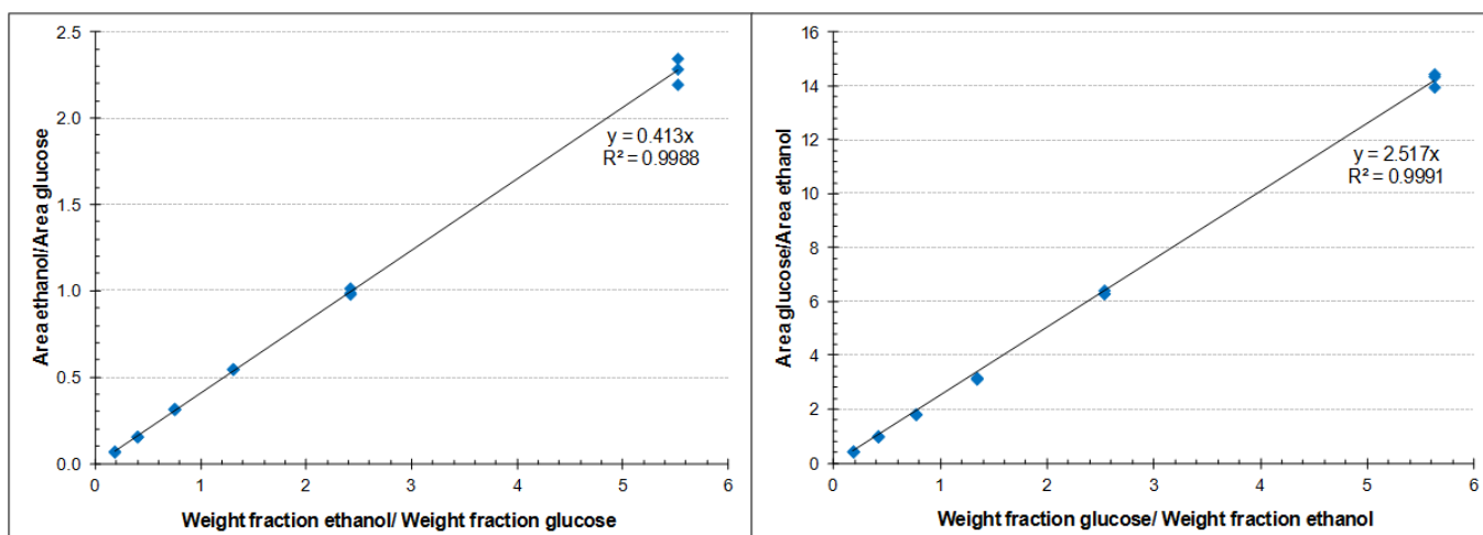
Figure B.3 Ethanol/Glucose calibration curve
