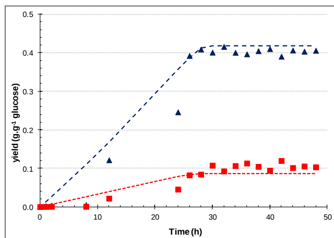
Figure I.9 Comparison of the membrane-reactor system model yields with experimental yields (▲ Experimental ethanol yield, ■ Experimental glycerol yield, --- ethanol yield model, ... glycerol yield model)
