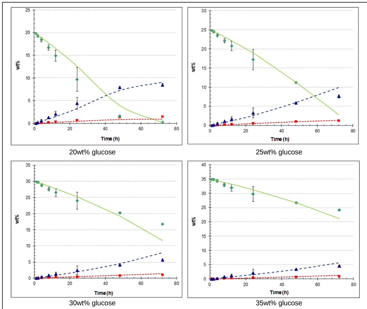
Figure I.5 Comparison of experimental fermentation data with substrate inhibition with substrate inhibition model using different starting sugar concentration and 10g/L yeast (♦ Experimental glucose, ▲ Experimental ethanol, ■ Experimental glycerol, — glucose model, --- ethanol model, ... glycerol model)
