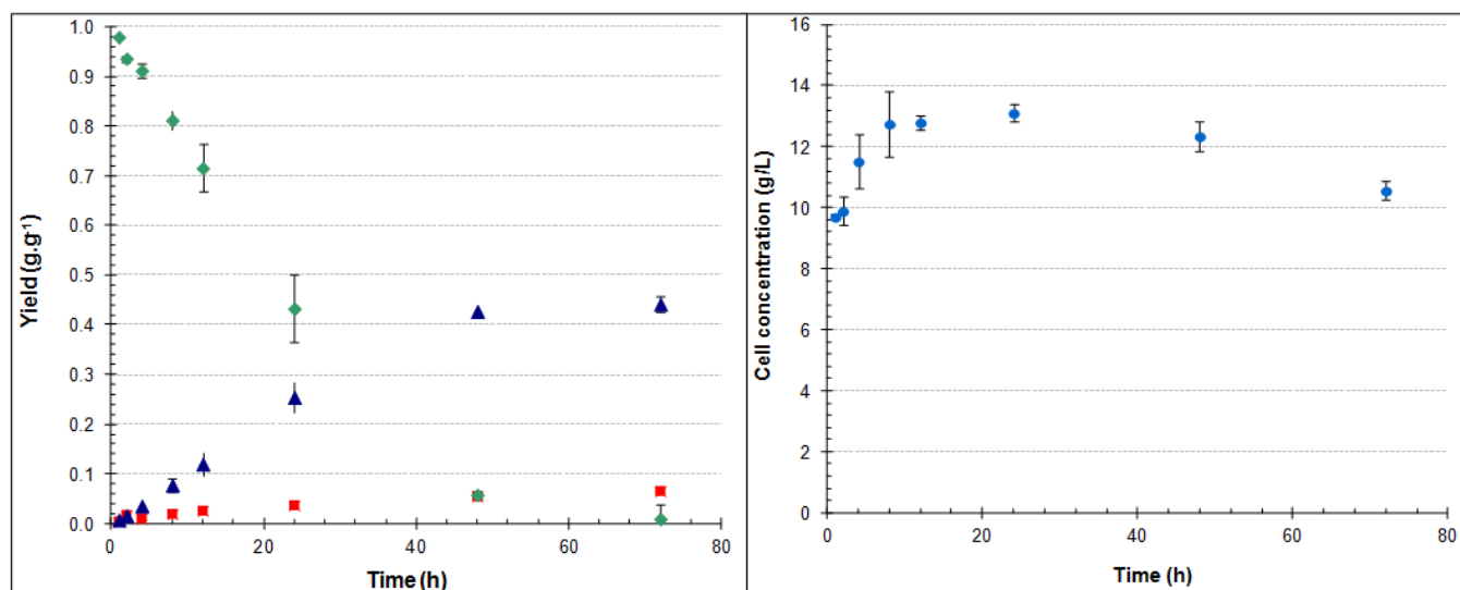
Figure C.15 Fermentation at a pH of 3.5
