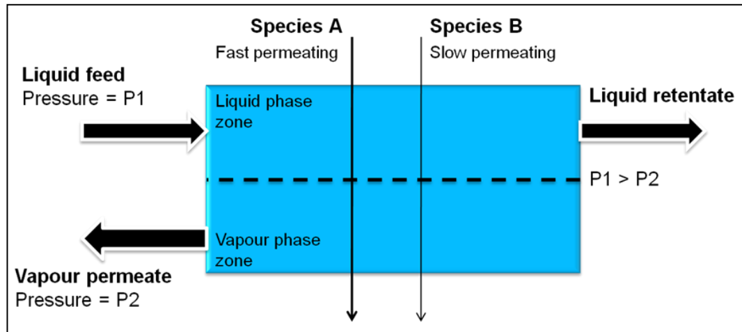
Figure 3.3 Pervaporation
