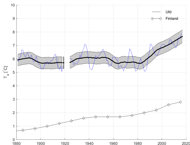
Figure 2. Average annual air temperatures at Utö during 1881–2016. The solid line represents temperatures calculated with DLM, and the gray area shows the 95 % confidence range calculated using bootstrap method. The blue line over the DLM curve is a 5-year running mean of atmospheric temperature at Utö. The thin black line with diamonds shows the decadal average temperatures calculated for all of Finland (Mikkonen et al., 2015).
