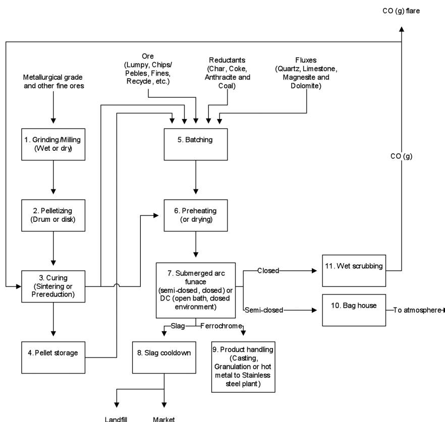
Figure 1—A flow diagram adapted from Riekkola-Vanhanen 7 , indicating most common process steps utilized for FeCr production in SA
