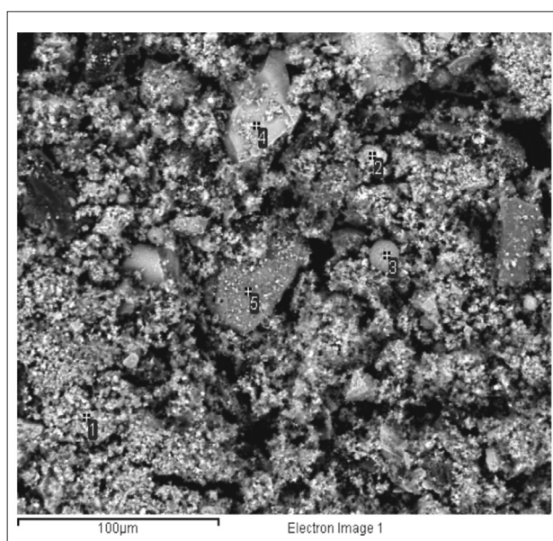
Figure 2—SEM photo of a bag filter dust sample originating from an open FeCr furnace in SA
