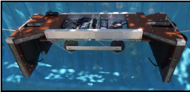
Fig. 4 Inspection robot balancing on transmission line.
