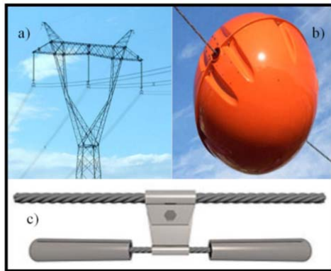
Fig. 3 (a) Tower structure; (b) visibility marker; (c) damper.
