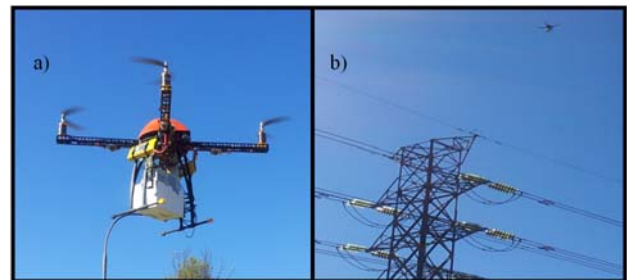
Fig. 6 (a) Quad-copter used for communication test; (b) quad-copter flying over transmission line.
