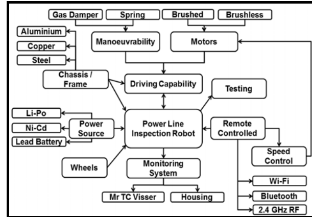
Fig. 2 Conceptual design of the line inspection robot.
