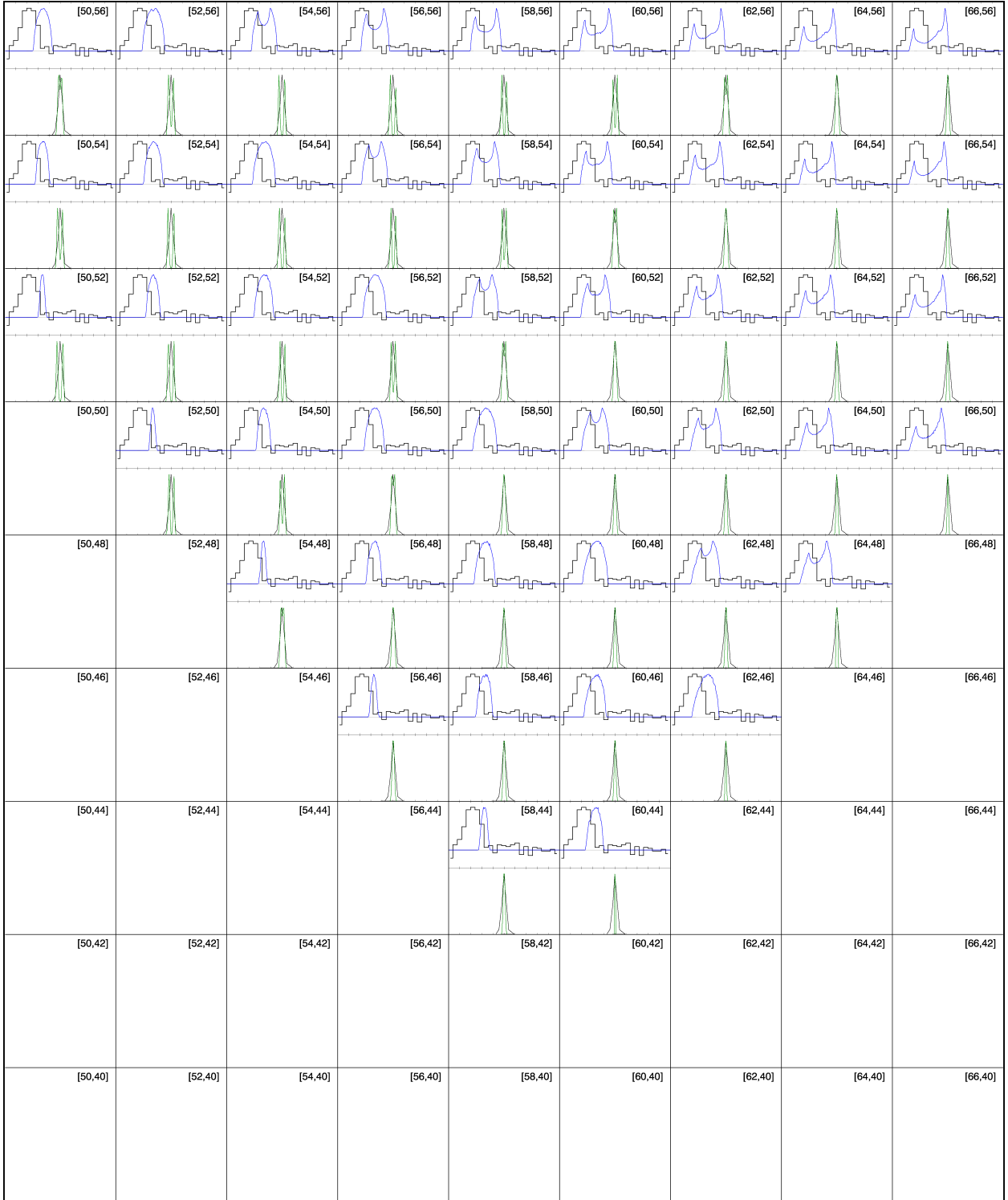
Figure A.5: OG atlas for PSR J0659+1414 with a 2^\circ resolution.
