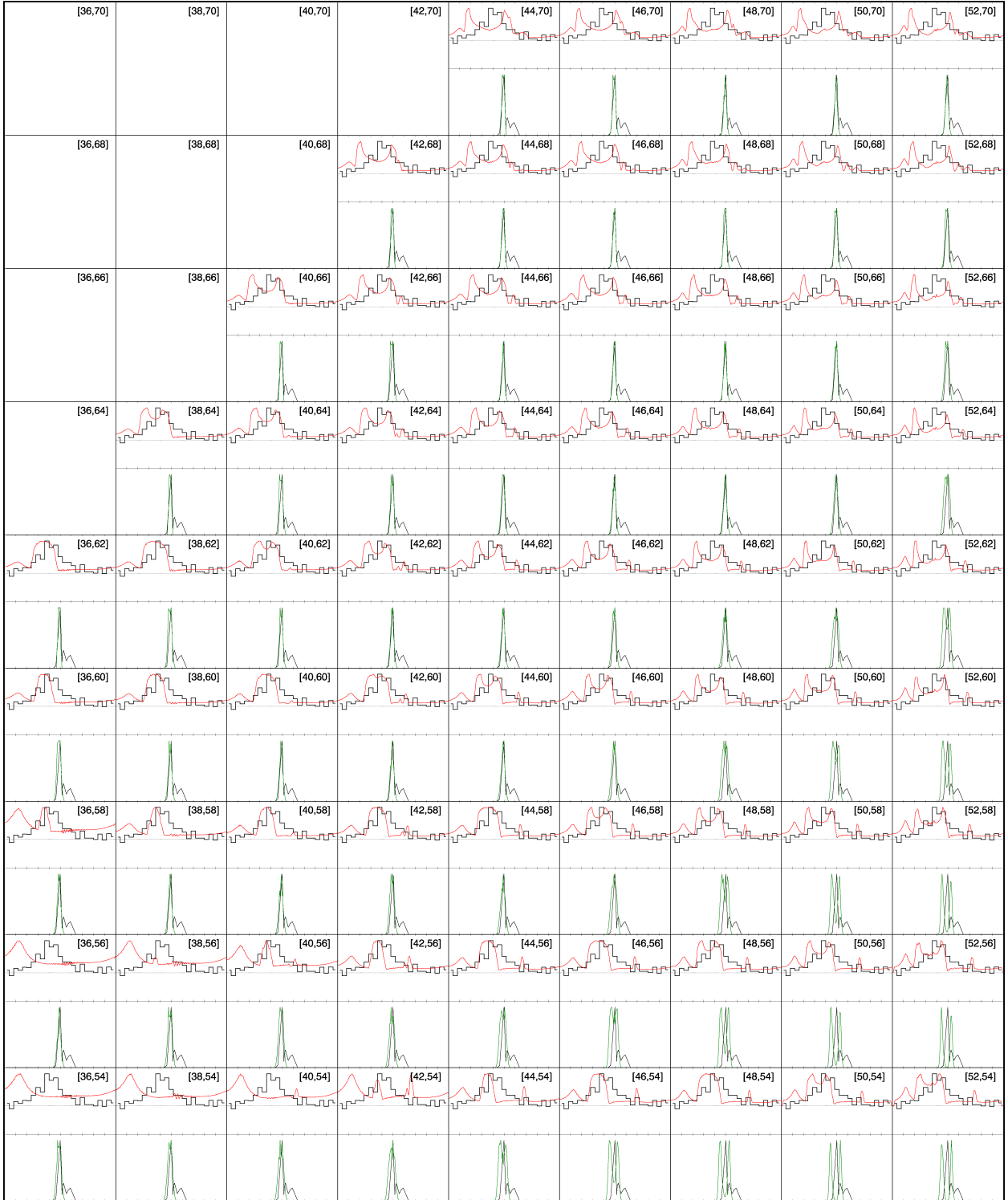
Figure A.15: AltTPC atlas for PSR J1718–3825 with a 2^\circ resolution.
