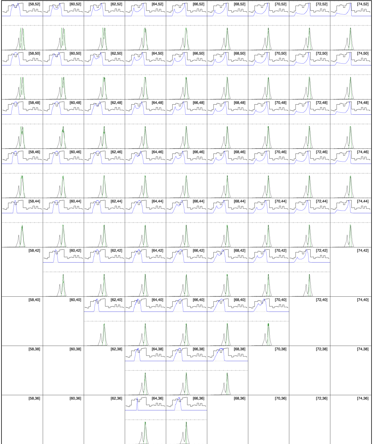
Figure A.11: OG atlas for PSR J1420–6048 with a 2^\circ resolution.
