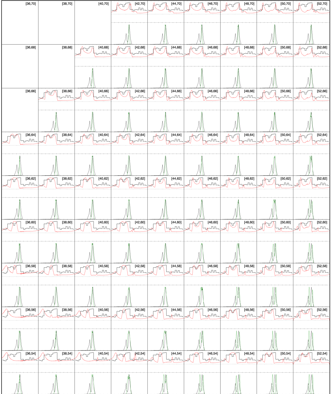
Figure A.10: AltTPC atlas for PSR J1420–6048 with a 2^\circ resolution.
