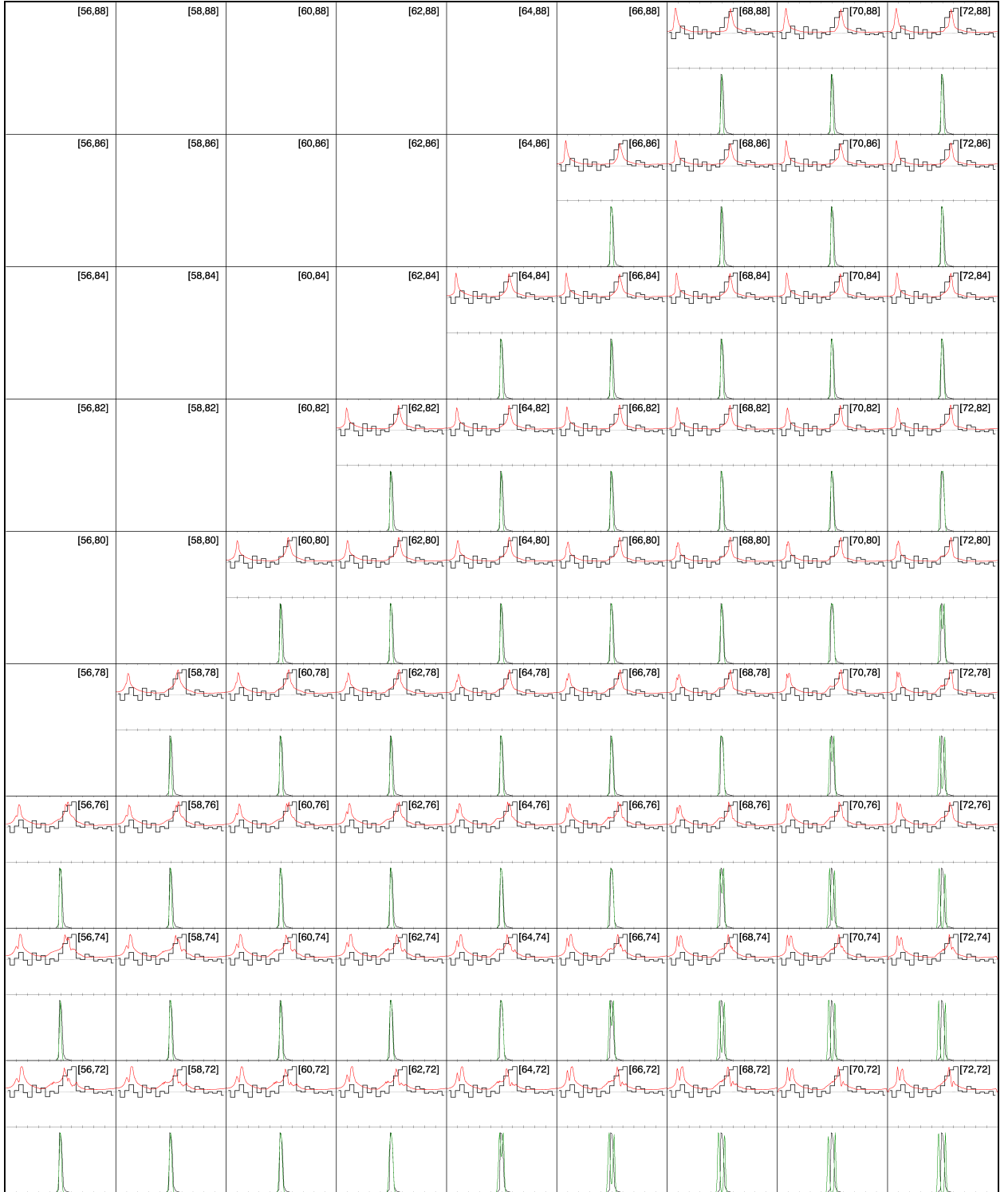
Figure A.6: TPC atlas for PSR J0742–2822 with a 2^\circ resolution.
