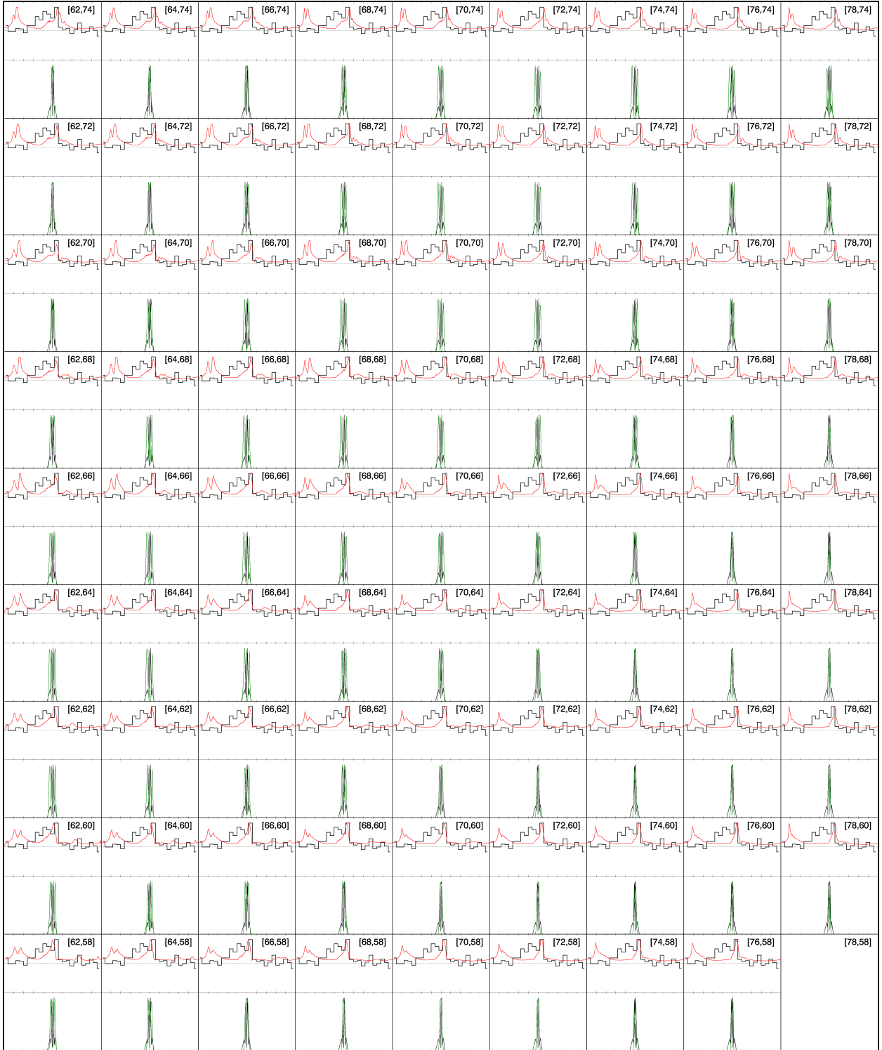
Figure A.1: TPC atlas for PSR J0631+1036 with a 2^\circ resolution.
