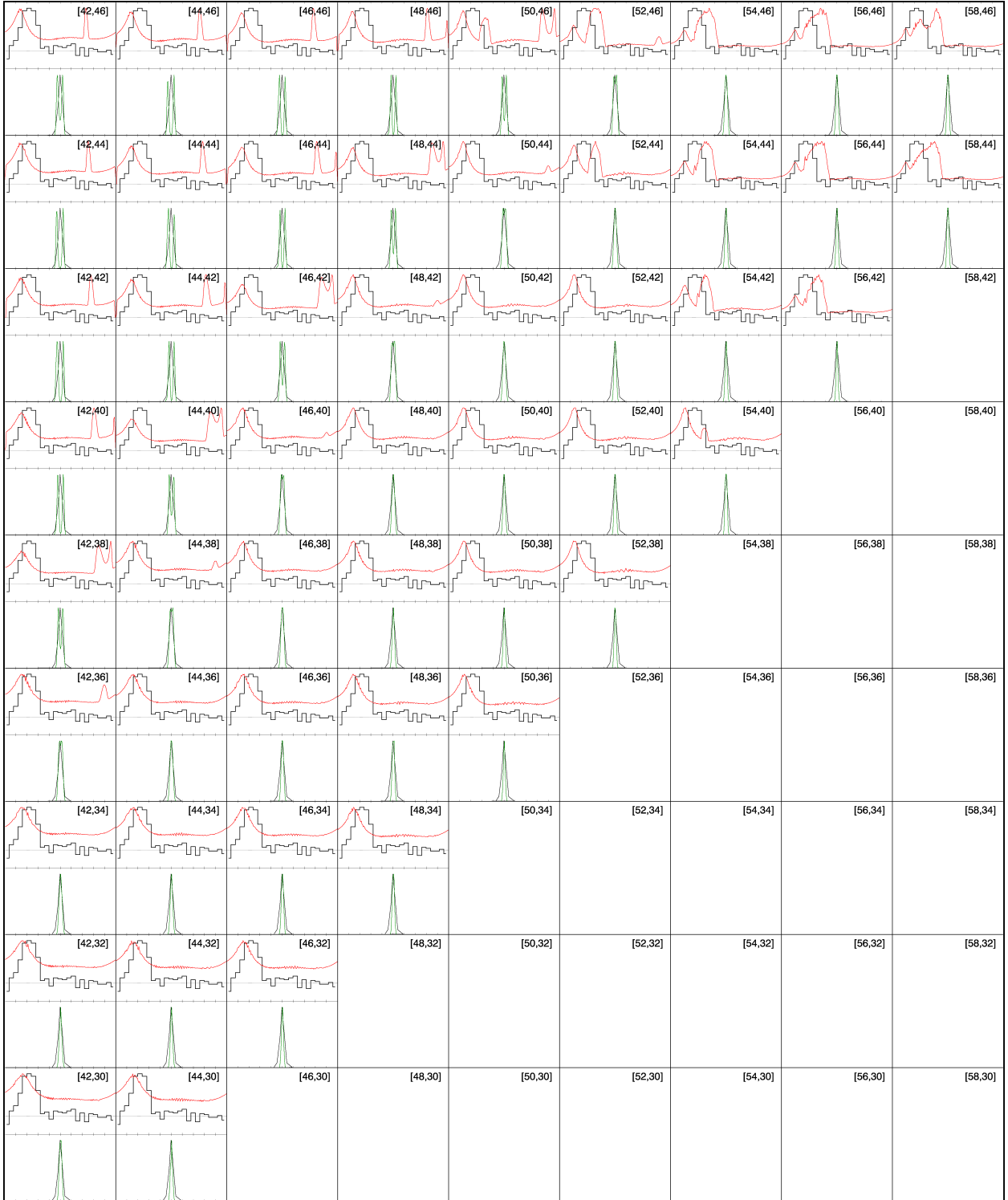
Figure A.3: TPC atlas for PSR J0659+1414 with a 2^\circ resolution.
