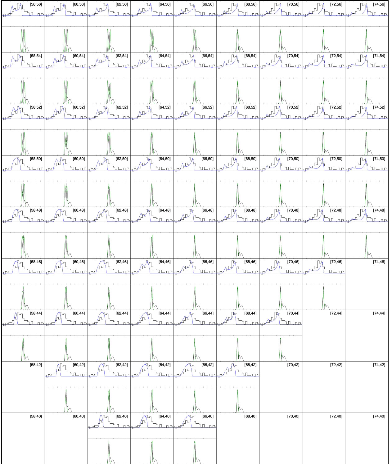
Figure A.16: OG atlas for PSR J1718–3825 with a 2^\circ resolution.
