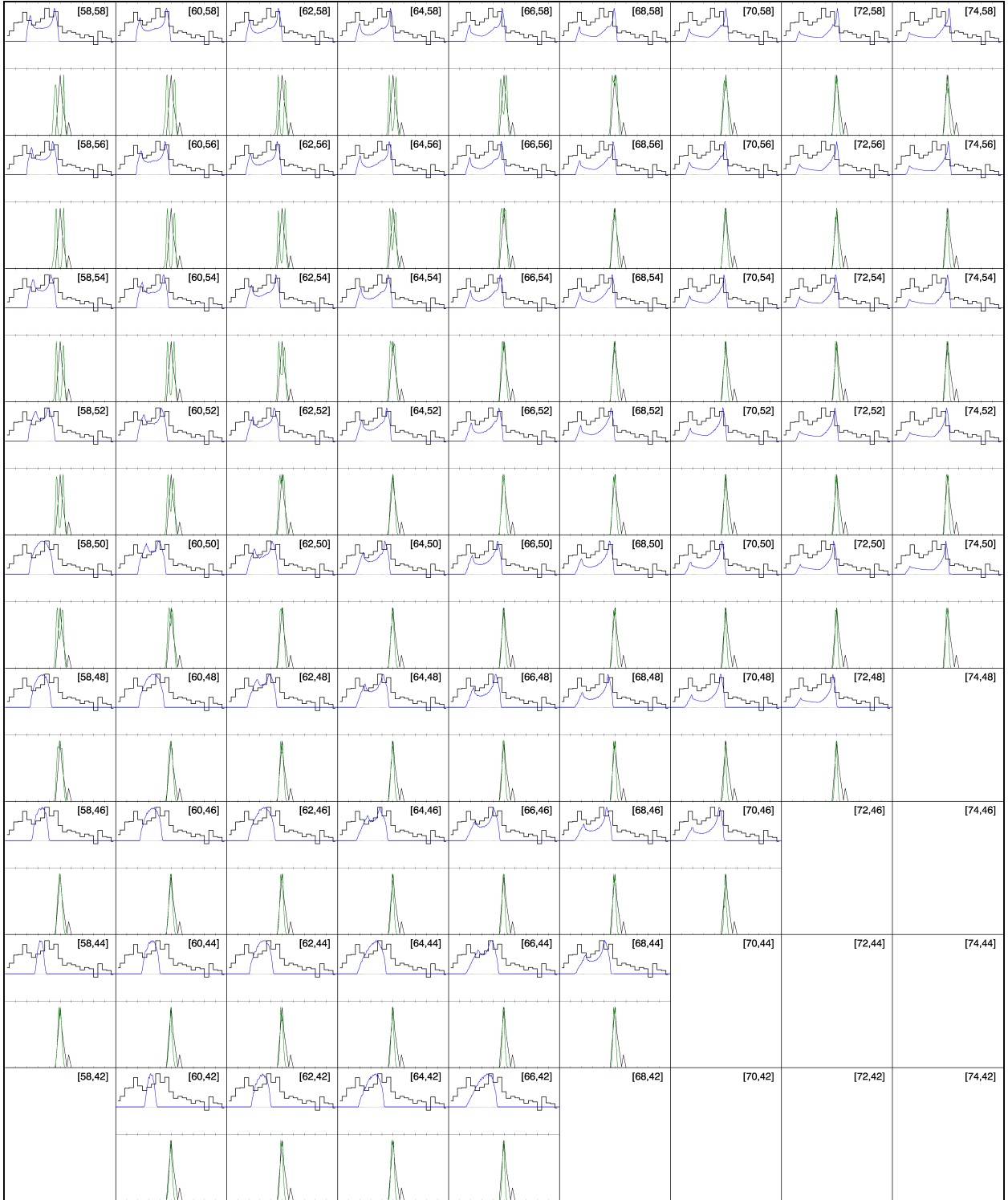
Figure A.13: OG atlas for PSR J1509–5850 with a 2^\circ resolution.
