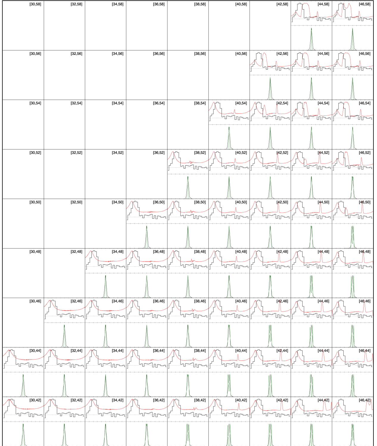
Figure A.4: AltTPC atlas for PSR J0659+1414 with a 2^\circ resolution.
