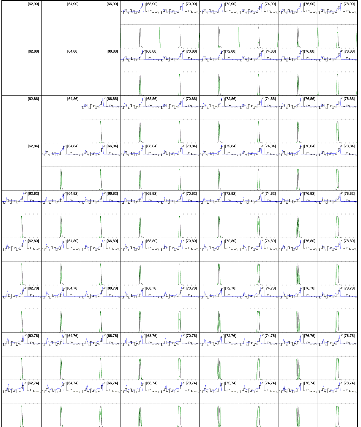
Figure A.8: AltOG atlas for PSR J0742–2822 with a 2^\circ resolution.
