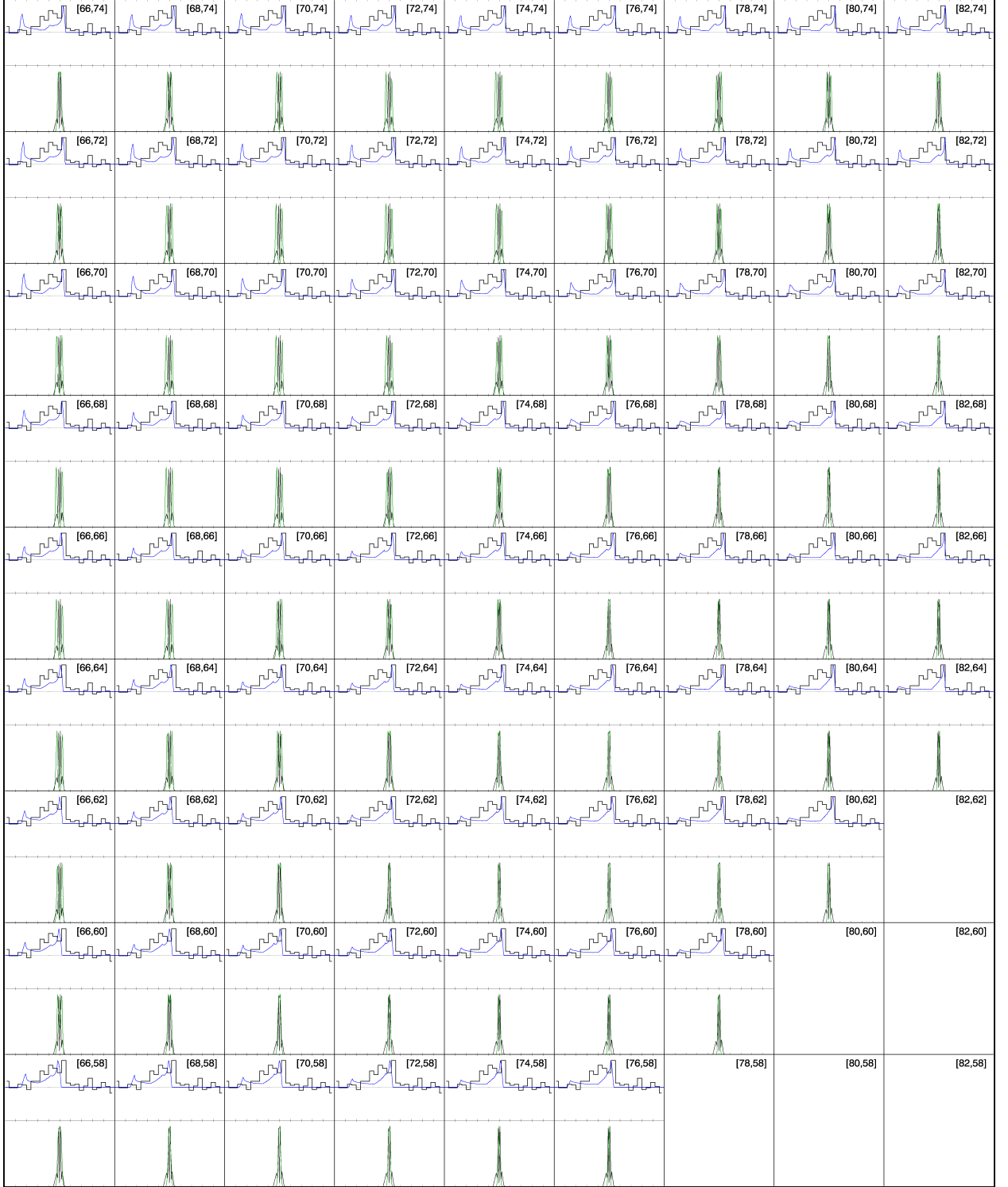
Figure A.2: OG atlas for PSR J0631+1036 with a 2^\circ resolution.
