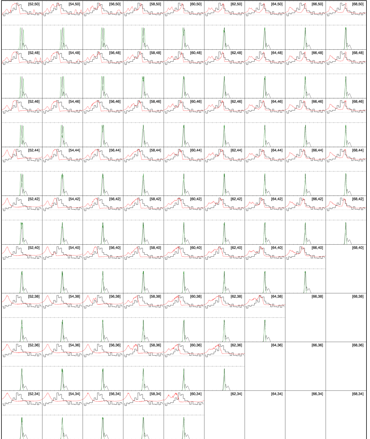
Figure A.14: TPC atlas for PSR J1718-3825 with a 2^\circ resolution.
