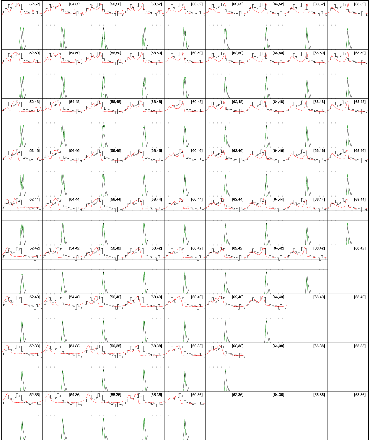
Figure A.12: TPC atlas for PSR J1509–5850 with a 2^\circ resolution.
