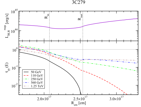
Figure 2. Results for 3C279. Lower panel: \gamma\gamma absorption optical depth as a function of location of the emission region, R_{\text{em}} , for a fixed value of u_{\text{BLR}} as encountered by the emission region at the respective location (see the text), for several \gamma -ray photon energies. Upper panel: required luminosity of the BLR, according to the re-normalization of the local BLR emissivity (Equation (8)).
