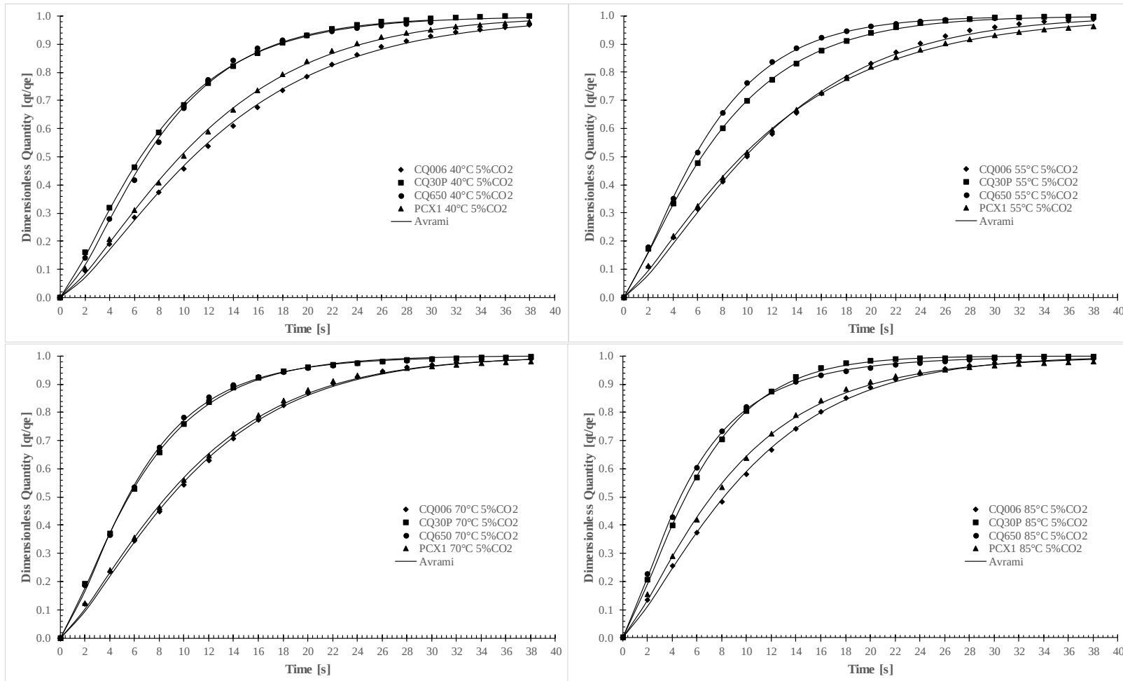
Figure C- 4: Comparing the experimental adsorption rate data of CQ006, CQ30P, CQ650 and PCX1 at 40, 55, 70 and 85 °C for at a fixed inlet CO 2 concentration of 5 vol%, modelled with the Avrami adsorption rate model.
