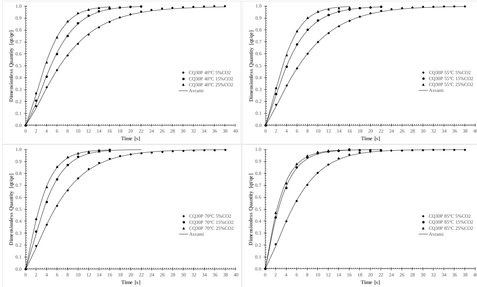
Figure C- 2: Experimental adsorption rate data at 40, 55, 70 and 85 °C for CQ30P at different inlet CO 2 concentration of 5, 15 and 25 vol%, modelled with the Avrami adsorption rate model.
