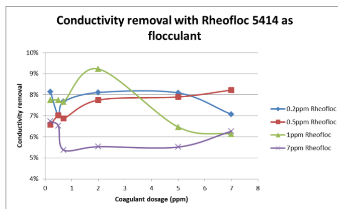
Fig 2: Conductivity removal @ 40°C
