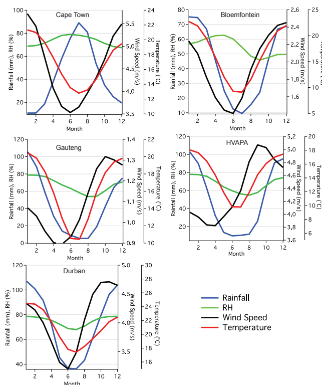
Figure 4. Monthly averaged values of RH, accumulated rainfall, wind speed, and temperature for sites in each satellite study area for the period 1 January 2000 to 31 December 2009. Note different y scales for each site.
