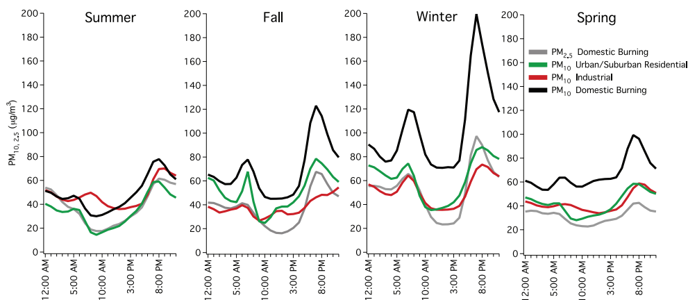
Figure 13. Average diurnal \text{PM}_{10} and \text{PM}_{2.5} for each site type.
