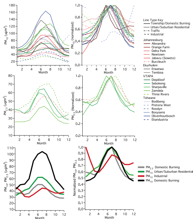
Figure 10. Monthly averaged \text{PM}_{10} , \text{PM}_{2.5} (absolute magnitude and normalized by maximum monthly average) and \text{PM}_{2.5}/\text{PM}_{10} for ground monitoring sites. Solid lines represent sites with domestic burning influence, fine dashed lines represent urban/suburban residential areas, and coarse dashed lines represent industrial sites.
