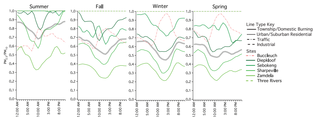
Figure 12. Season-averaged diurnal \text{PM}_{2.5}/\text{PM}_{10} , indicating the diurnal variability in the ratio of fine to coarse particles. Solid lines represent sites with domestic burning influence, fine dashed lines represent urban/suburban residential areas, and coarse dashed lines represent industrial sites.
