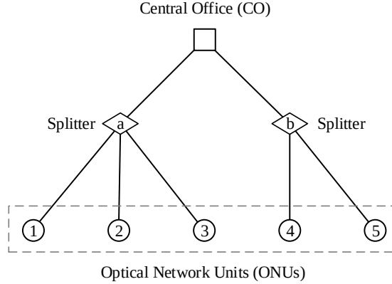
Figure 1: A schematic layout of the PON topology.
