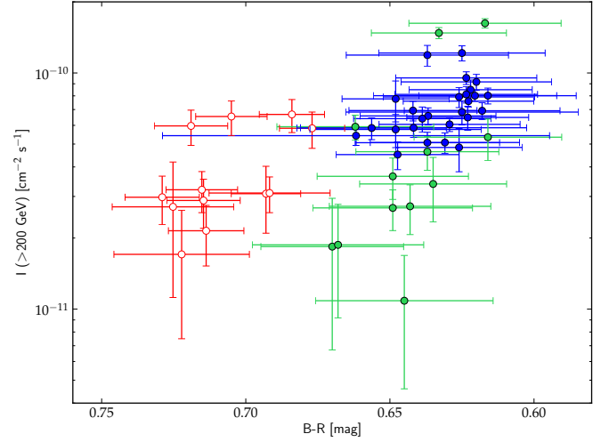
Fig. 4. VHE \gamma -ray photon flux I_{>200\text{GeV}} vs. B - R colour for PKS 2155–304 during the 2007–2009 period. The applied colour coding is the same as in Figs. 1 and 2.
