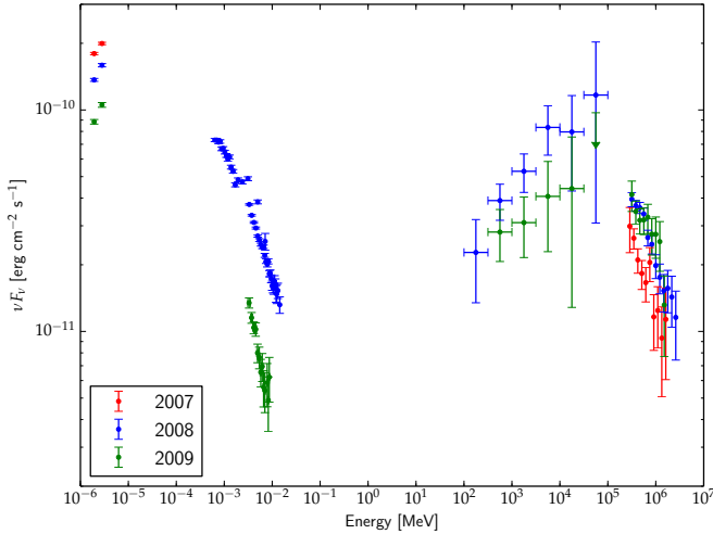
Fig. 5. Average broadband SEDs of PKS 2155–304 for the years 2007, 2008, and 2009 (red, blue and green symbols, respectively), constructed using quasi-simultaneous data collected with ATOM, RXTE, Swift , Fermi -LAT, and H.E.S.S.
