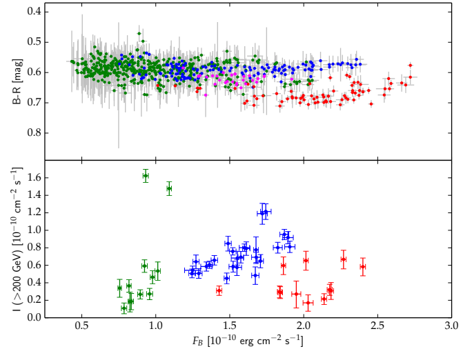
Fig. 2. Upper panel: B - R colour vs. the B -band energy flux for PKS 2155–304 during the analysed period 2007–2009. Lower panel: corresponding VHE \gamma -ray photon flux of the source also as a function of the B -band energy flux. The applied colour coding is the same as in Fig. 1. We note two distinct optical spectral states appearing at high flux levels in the upper panel , and the correspondingly distinct optical–VHE correlation pattern emerging in the lower panel (green and blue points), for details see Sect. 3.4. The colour uncertainties are calculated as rms.
