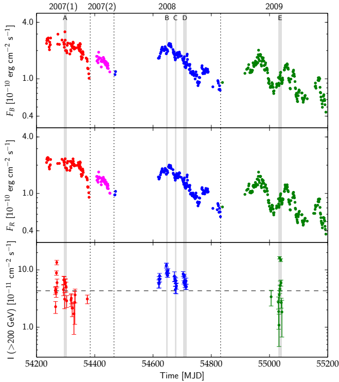
Fig. 1. Optical (ATOM; B and R bands) and VHE \gamma -ray (H.E.S.S.) lightcurves of PKS 2155–304 during the period 2007–2009 ( upper , middle , and bottom panels , respectively). The observations performed in 2007 until MJD 54 385 are denoted by red symbols, in 2007 after MJD 54 385 by magenta symbols, in 2008 by blue symbols, and in 2009 by green symbols; these epochs are also separated by the dotted vertical lines. For the two upper panels the error bars are within the size of the points. The optical and VHE lightcurves are binned in one-night intervals. We note uneven sampling of the lightcurves at optical and VHE frequencies, as well as different integration times between the optical and VHE exposures. The horizontal line in the lower panel indicates the quiescent state of the source, defined in Abramowski et al. (2010). The vertical grey lines indicate the A–E intervals defined in Sect. 3.4.
