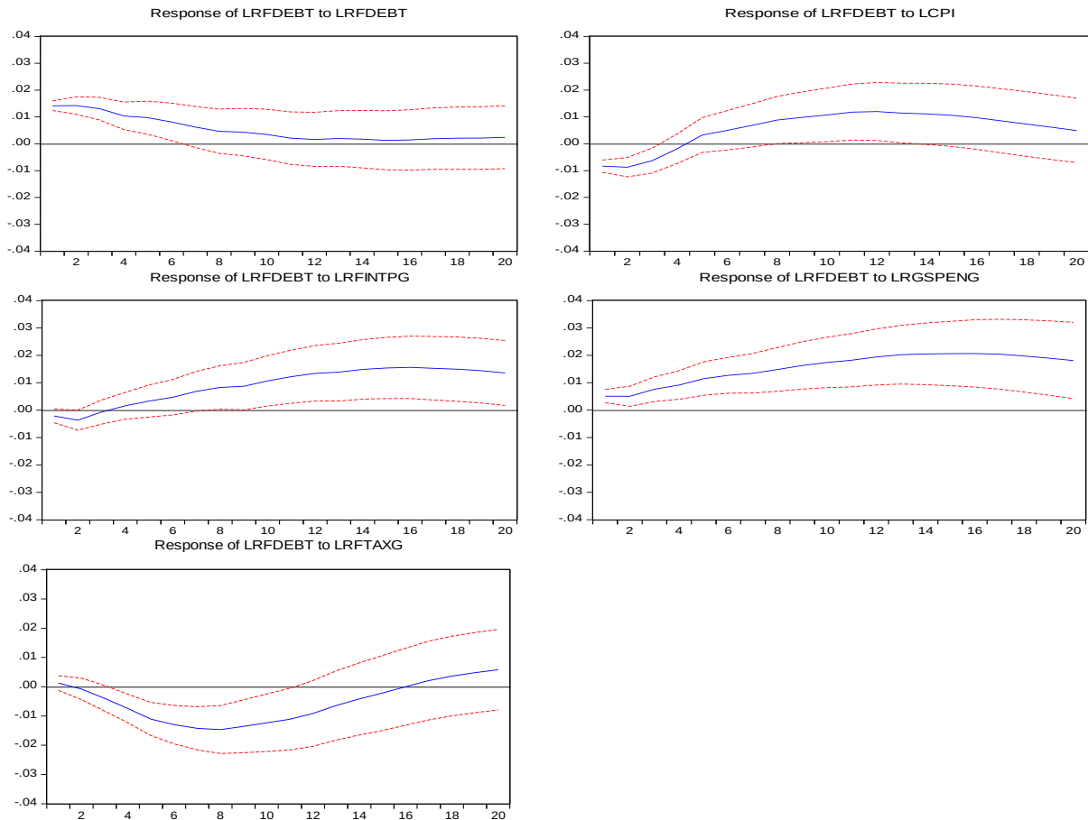
Figure 3. Response of LRFDEBT to independent variables
