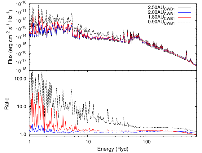
Figure 6. Top panel: results from the calculation of the SED from the shocked gas for adiabatic and radiative cooling gas. Bottom panel: the ratio of each SED relative to the SED for 2.5 au (black line). This shows that radiative cooling gas results in SEDs with increased flux of lower energy ionizing photons.
