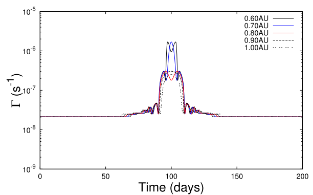
Figure 8. The interpolated time-dependent ionization rates obtained from the equilibrium states of the IF of the H II region. This is an example for a 200-d period for a fixed constant neutral hydrogen density and mass-loss rate combination, for several periastron distances.
