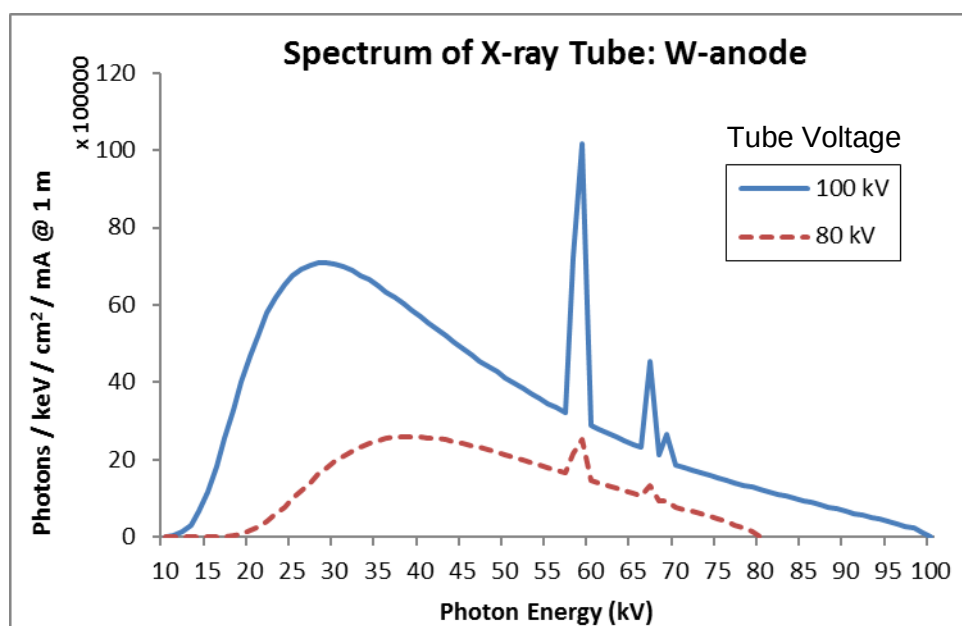
Figure 2.4: Spectrum of an X-ray tube with a tungsten anode for 2 different tube voltages calculated with SPEKCALC.
