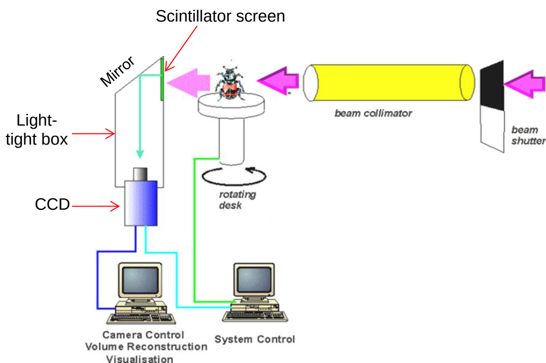
Figure 2.10: Scintillator screen and detector geometry of the radiation detection layout for digital neutron and X-ray radiography and tomography. (Courtesy: PSI).
