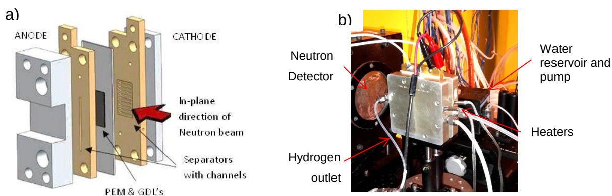
Fig. 2. a) Schematic illustration of the experimental setup and in-plane direction of the neutron beam [1]. b) Experimental set up of the electrolyzer fuel cell in the NI chamber at NIST.
