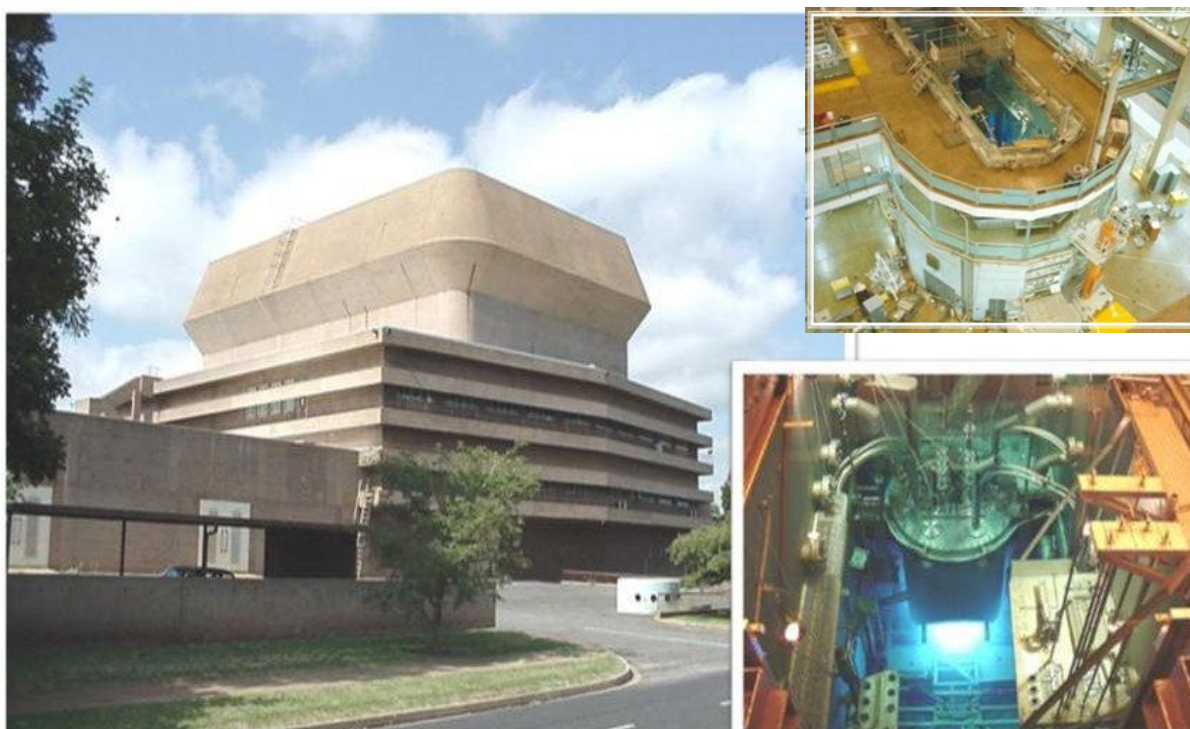
Figure 2.23: Necsa's SAFARI-1 nuclear research reactor at Pelindaba. (Courtesy: Necsa).
