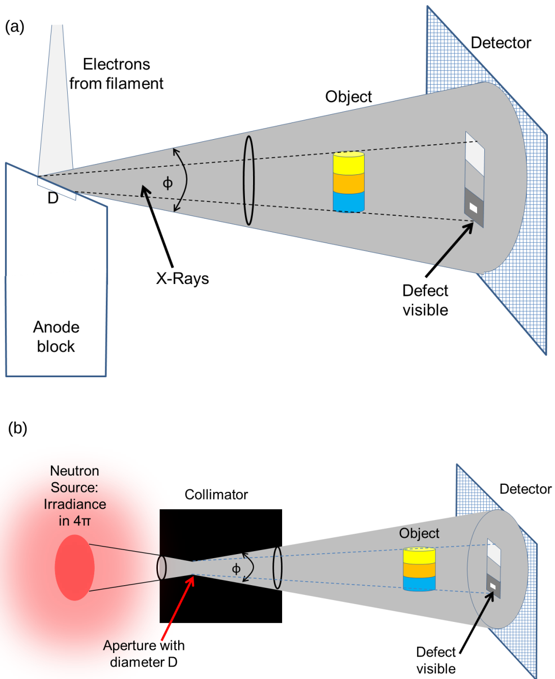
Figure 2.2: Schematic diagram of the classical principle and setup for (a) X-Ray and (b) neutron radiography each with a sample rotation capability for tomography application. (After: Halmshaw, 1988) (After: Domanus, 1987).
