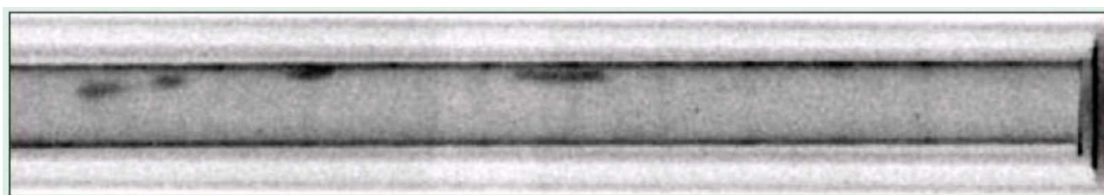
Figure 15 - Neutron radiograph of nuclear fuel and cladding material showing (black spots) hydrogen accumulation within the Zr TM -tubing (Frajtag, n.d.).
