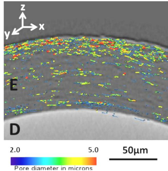
Figure 22 – Xradia VersaXRM orthoslice showing the SiC (D) and OPyC (E) layers with the pore volumes superimposed. Pore diameter is colourcoded to identify large pore clustering (Lowe et al, 2015)
