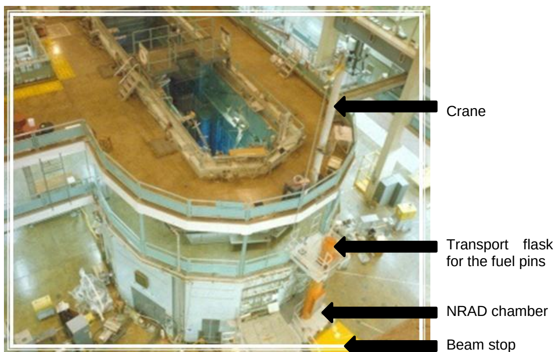
Figure 3.1: Neutron radiography set-up at beam tube 4 on the beam port floor of the SAFARI-1 nuclear research reactor for PIE of LTA fuel pins.
