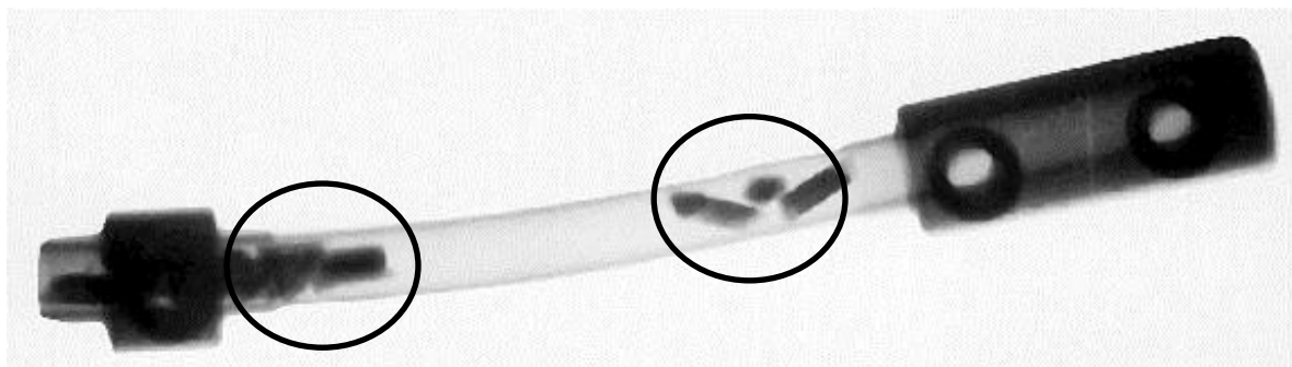
Figure 2.27: Film neutron radiograph of the blockage (encircled) of aircraft fluid flow components. (Photo: Courtesy of Mr. Don Uytenbogaard).
