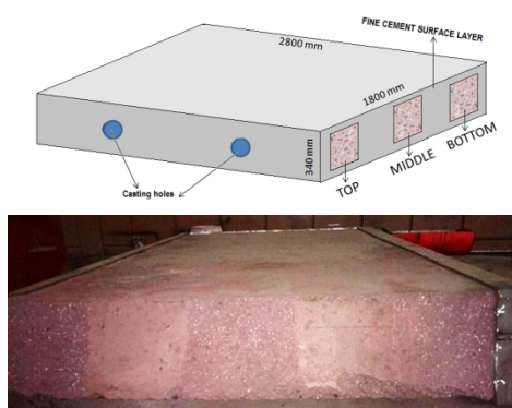
Fig. 7. TOP: Schematic of a shield block with exposed top, middle and bottom windows. BOTTOM: Photograph of the three exposed areas, showing uniform general aggregate consistency in all three exposed windows (top window is on the left)
