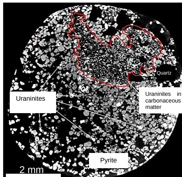
Figure 2.2: Demonstration of the performance of the PerkinElmer Amorphous Silicon X-ray flat panel detector. Large geometric magnification resulted in high pixel resolution in the 2D slice of a \mu XCT tomogram showing small uraninite grains, quartz-pyrite matrix and carbonaceous matter but with sharp defined edges. (Courtesy: Necsa).
