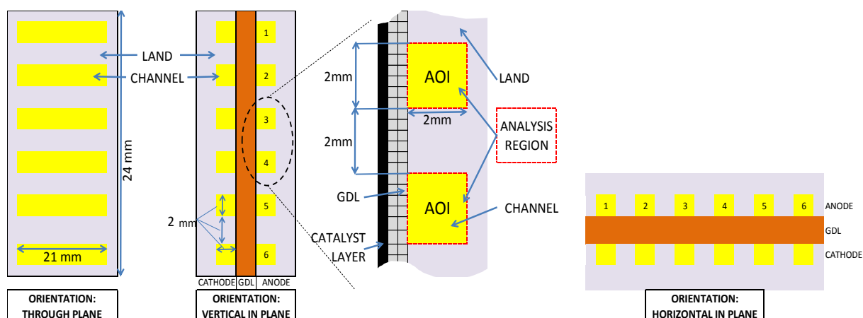
Fig. 4. Schematic diagram of the detail of the dimensions of the PEM electrolyzer fuel cell. Experiments were performed only in both the in-plane orientations (vertical & horizontal) with the channels (yellow) as main areas-of-interest.
