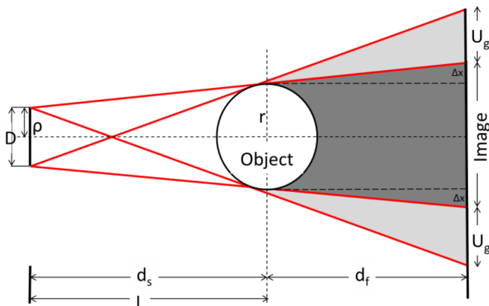
Figure 2.3: Schematic diagram of a radiography geometry setup. (Courtesy: Necsa).
