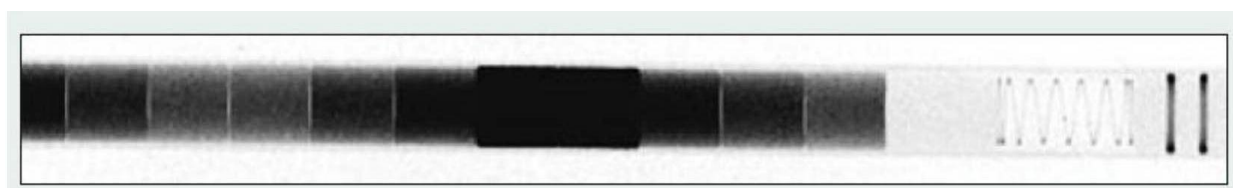
Figure 8 - Neutron radiograph (film) of fresh fuel pellets in a fuel pin with varying degrees of isotopic U-235 enrichment. Pellets loaded with higher enrichment appear darker (Frajtag, n.d.)
