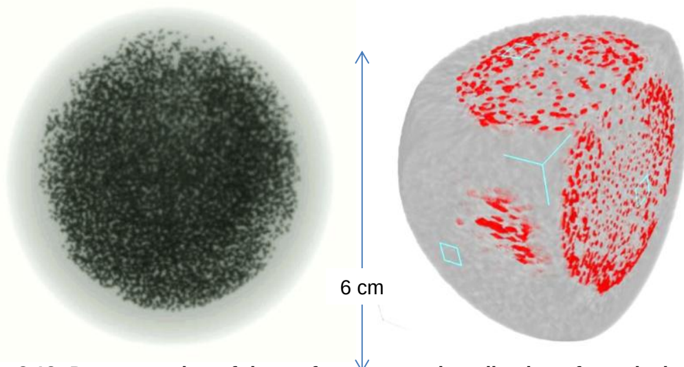
Figure 2.12: Demonstration of the performance and application of a typical scintillator - CCD-camera based digital setup with a 1 mm X-ray focal spot on a PBMR fuel sphere: LEFT: Low quality X-ray radiograph with low definition of the TRISO particles, but ability to visualise the fuel containing core and fuel free zone. RIGHT: Corresponding low quality sliced X-ray tomogram. (Courtesy: Necsa).
