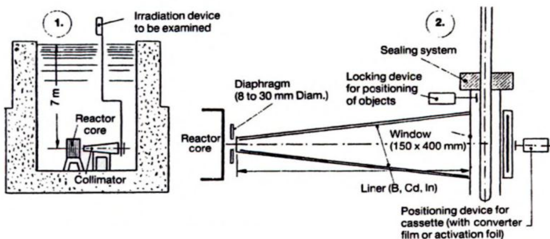
Figure 2.26: In-pool collimator set-up for neutron radiography.(Domanus, 1987).
