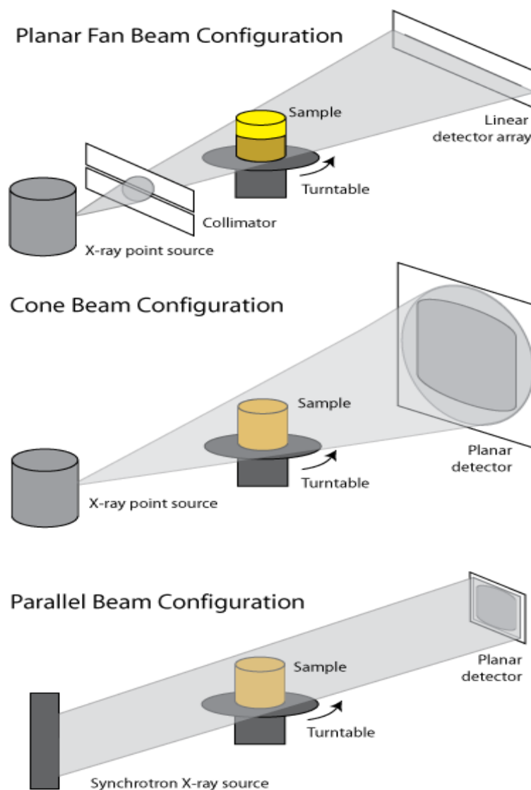
Figure 2.17: Tomography beam geometries.
