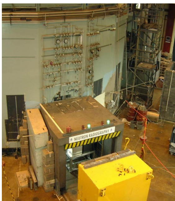
Figure 3.3: Relocation of the neutron radiography facility at beam port no. 2 of the SAFARI-1 reactor.
