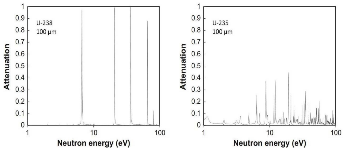
Figure 9 - Neutron attenuation of 100 micron thick U-235 and U-238 isotopes calculated from the tabulated data on the total cross sections as a function of neutron energy (Tremisn et al , 2013)
