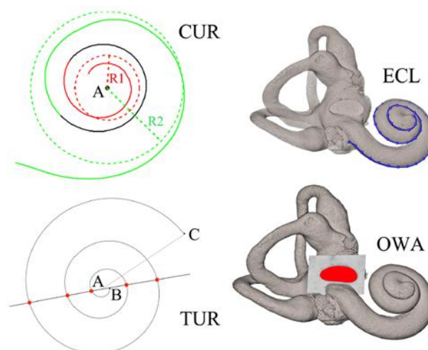
Fig. 7.4. Illustrations of the five cochlear features expressed as continuous variables. The external cochlear length (ECL, in mm), number of turns (TUR, expressed as the sum of full circle rotations and the angle between lines “AB”—center to apex—and “AC”—center to base), and relative length (RECL = ECL/TUR, in mm), the curvature gradient (CUR, expressed as a dimensionless ratio between the radii of the larger first—noted “R2”—and the smaller last spiral turns—noted “R1”), and the oval window area (OWA in mm 2 ) Courtesy: (Braga et al, 2013).
