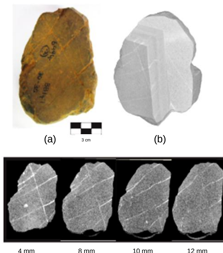
Fig. 7.22. Slab BB147 from Excavation 6. (a) A photograph showing a grid of lines visible on the surface. (b) A cutaway midway through the slab, showing that the lines continue as fissures (visible as white lines) through the slab. (c) Slices at 4, 8, 10 and 12 mm from the surface, showing the persistence of the grid pattern through the slab ( Courtesy: Jacobson et al, 2013 ).
