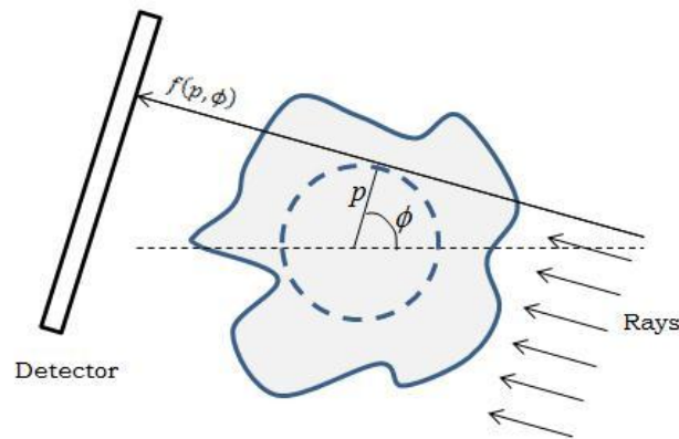
Figure 2.19: Reconstruction geometry for a general 2D density distribution. (Courtesy: Necsa).
