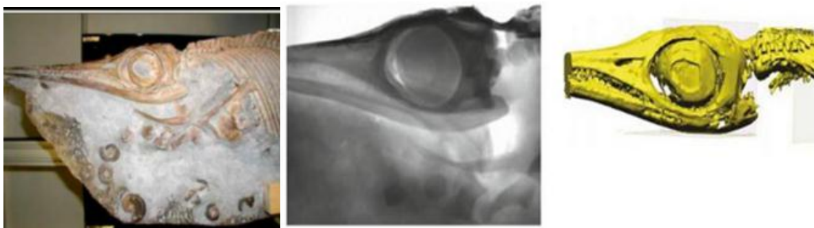
Fig. 7.12. : Left: Photo of the head section; Middle: Transmission neutron radiograph; Right: 3D printed model based on neutron tomography data of the head section ( Courtesy: PSI and Liang et al, 2008).
