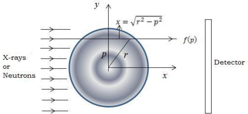
Figure 2.18: Reconstruction of a cylindrically symmetric object slice. (Courtesy: Necsa).
