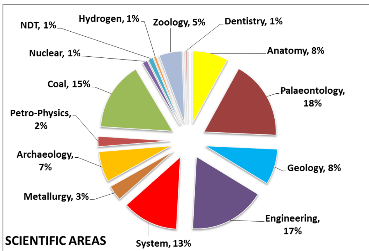
Figure 3.20: Miscellaneous scientific areas covered in the total output generated at the Necsa's radiography and tomography facilities to date.
