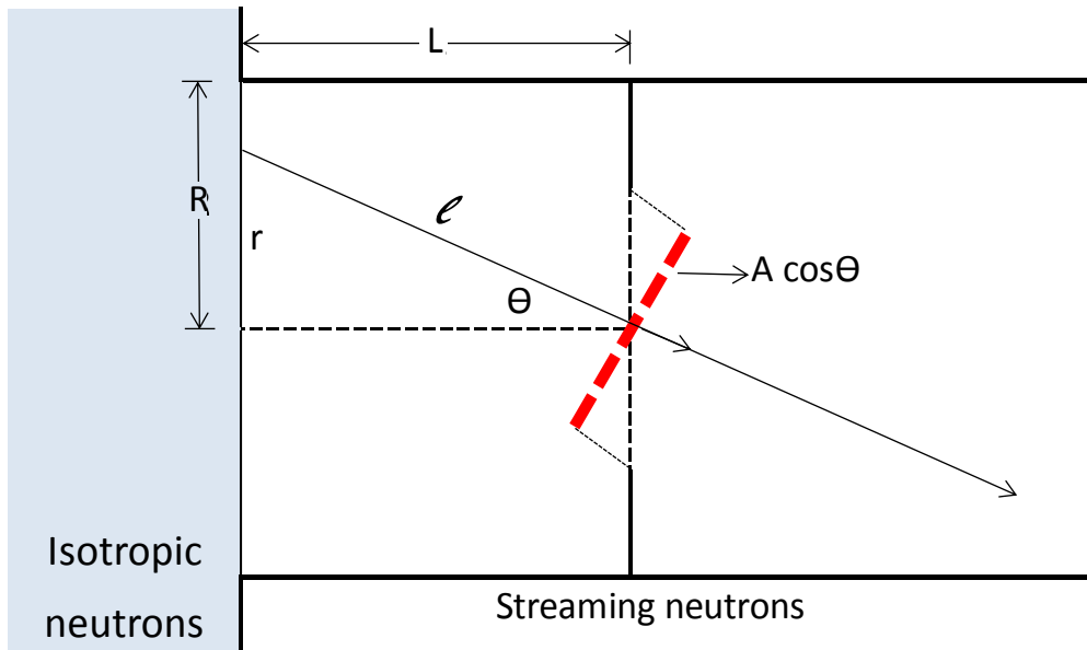
Figure 2.5: Thermal neutrons streaming down a reactor flight tube. (Courtesy: Necsa).
