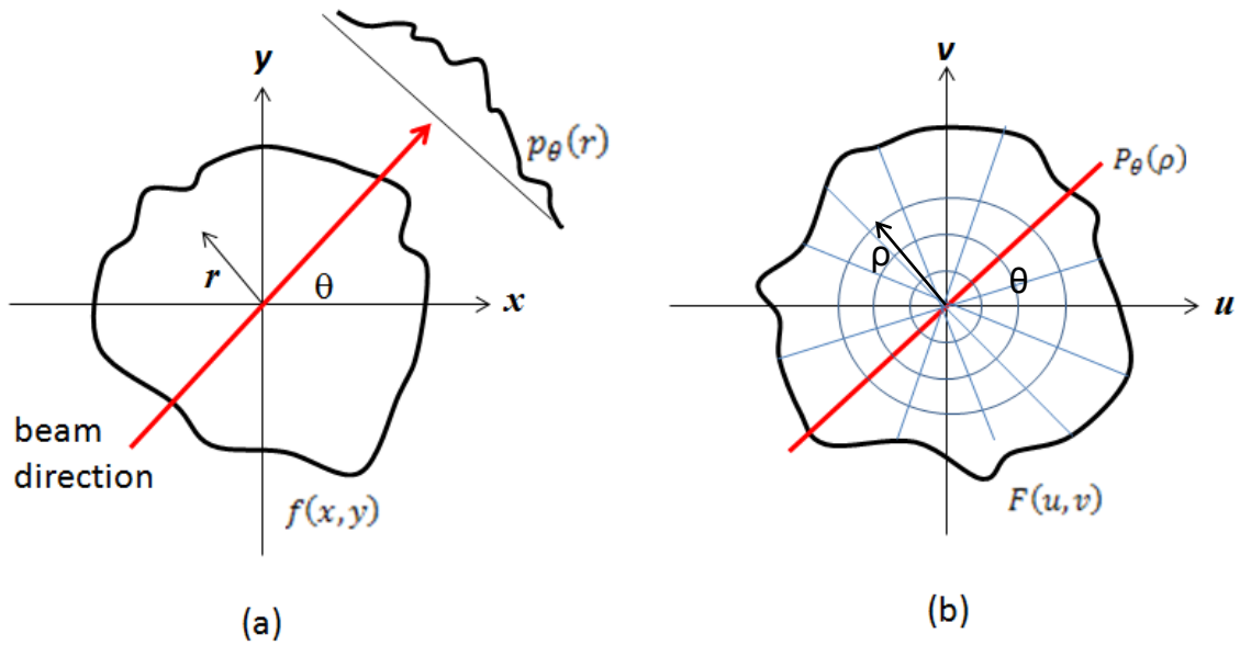
Figure 2.20: (a) Graphical representation of a 2-dimensional slice f(x,y) in the Cartesian plane. (b) Fourier transform of f(x,y) in the spatial frequency space (u,v) . (Courtesy: Necsa).
