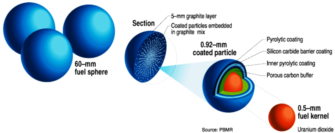
Figure 17 - Composition of PBMR-fuel (Weil, 2001)
