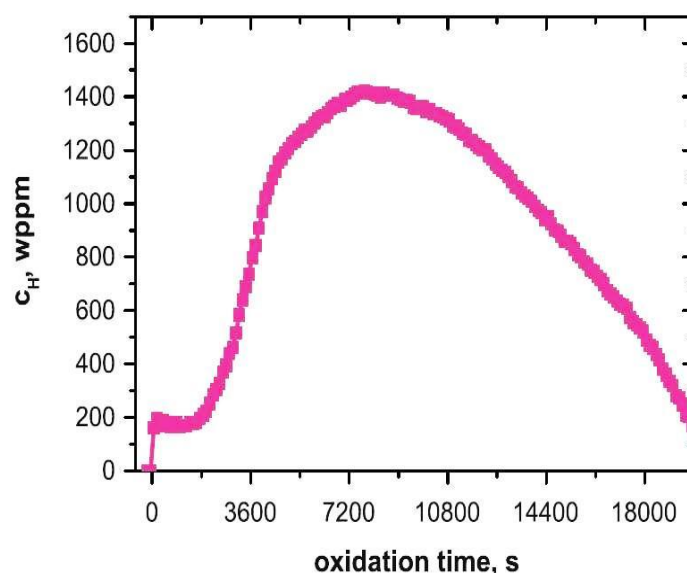
Figure 16 - Neutron radiography (Nrad) investigation: kinetics of hydrogen uptake and release during steam oxidation (Frajtag, n.d.)
