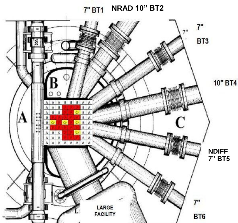
Figure 2.24: Radiation beam lines from the reactor core towards the beam port hall. Beam Tube 5 (BT5) and BT2 currently host the Neutron Diffraction (NDIFF) and Neutron Radiography (NRAD) facilities respectively. (Courtesy: Necsa).
