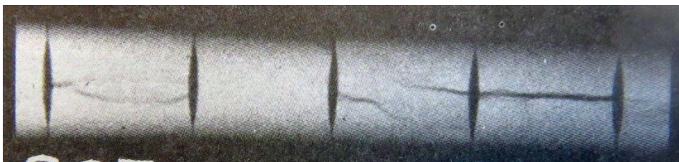
Figure 2.9: Demonstration of the application of the track-etch technique in neutron radiography using B-10 converter screens and nitro-cellulose film. A radiograph of post irradiation nuclear fuel pellets (10 mm long) inside a 10 mm diameter Zirconium-rod reveals shrinkage and crack formation. (Domanus 1987).
