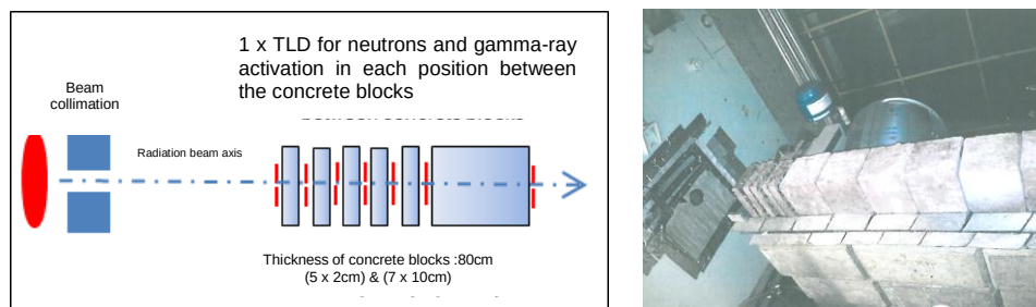
Fig. 9. Schematic- and physical layout of the experiments with the dose meters inside the NRAD experimental chamber
