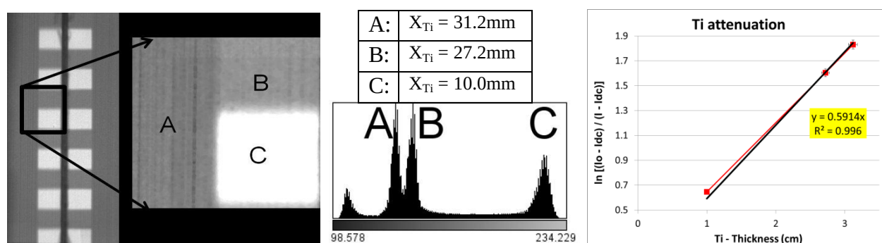
Fig. 6. Determination of the Ti neutron attenuation: LEFT: Neutron radiograph with system at dry state showing zoomed in view with the areas A,B and C. MIDDLE: Histogram with pixel values for 3 individual regions. RIGHT: Utilization of eq-4 in a graph to determine the \Sigma_{Ti} .
