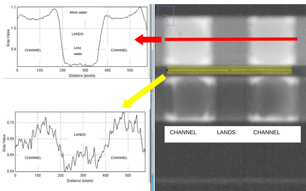
Fig. 7. TOP LEFT: A line profile at the position of the channels and land at the anode within the Ti-body of the electrolyzer. BOTTOM LEFT: A line profile at the position of the GDL spanning across the channels and land. RIGHT: Neutron radiograph at the horizontal orientation of the electrolyzer of 2 channels and 1 land indicating the positions of the line profiles.
