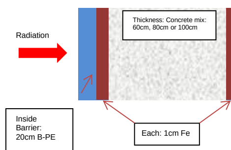
Fig. 5. Cross section of the radiation shielding barrier of the SANRAD facility
