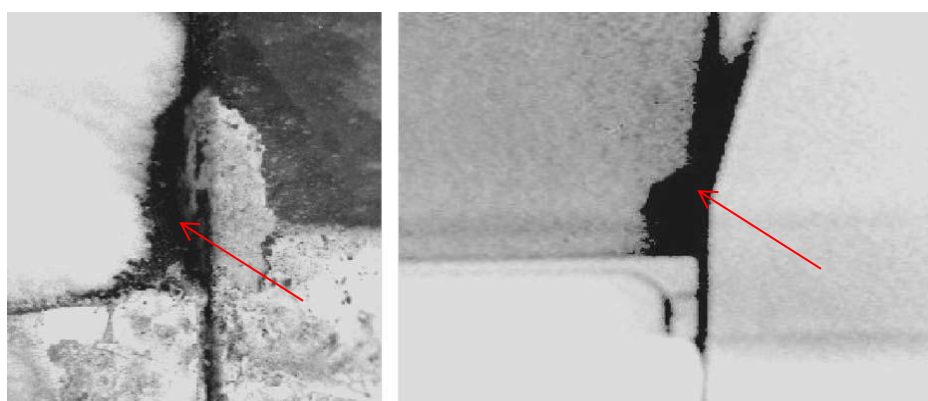
Figure 2.7: Demonstration of the successful application of the direct technique in neutron radiography using Gd-metal foil and D4 X-ray film to reveal water ingress into the structure of a helicopter main rotor blade. Arrows indicate areas of water ingress. (Courtesy: Necsa).
