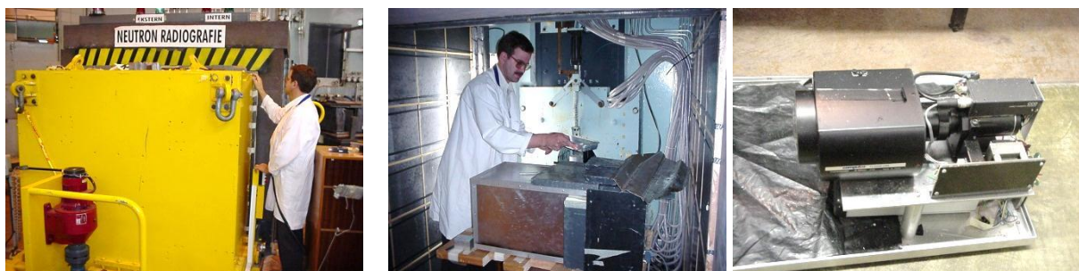
Figure 3.2: LEFT: First neutron radiography facility at beam port 4. MIDDLE: Electronic camera box partially covered with borated wax and B 4 C materials as radiation shield. RIGHT: First electronic neutron radiography camera system.
