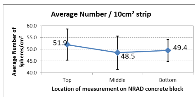
Fig. 8. Average number of steel shot balls counted at the top, middle and bottom positions of the exposed surfaces on the test concrete block in 10 cm² strips within each position
