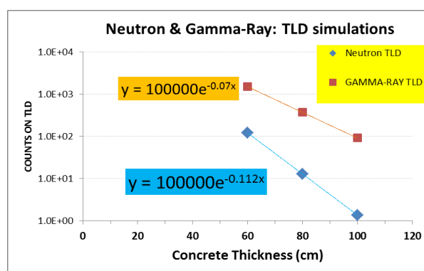
Fig. 10. Trend of attenuation of neutron- and gamma-ray radiation in laboratory concrete samples through TLD exposure and analysis
