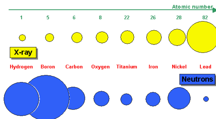
Figure 2.14: Graphical comparison of neutron and X-ray attenuation for some elements. (Courtesy: PSI).
