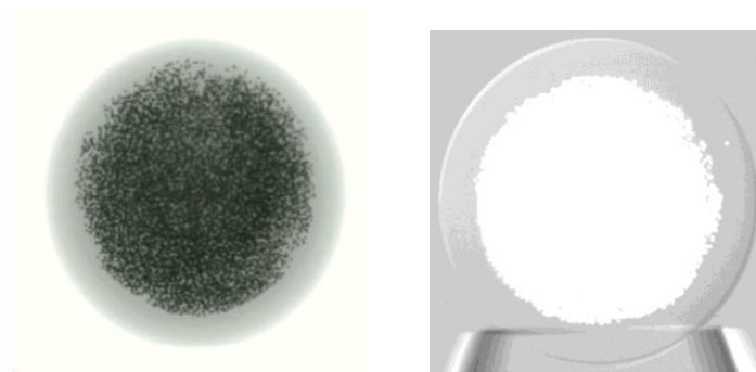
Figure 18 - X-ray tomography of a PBMR fuel pebble. Left: the non-centralized fuel sphere within the carbon matrix. Right: Location and identification of a TRISO particle inside the fuel-free zone (Necsa, 2006)
