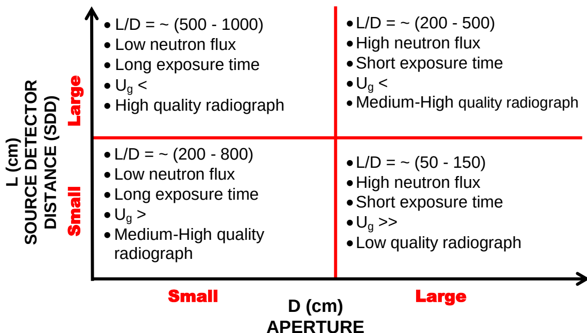
Figure 2.6: L/D characteristics and their consequences for neutron radiographic setups. (After: Domanus, 1987)
