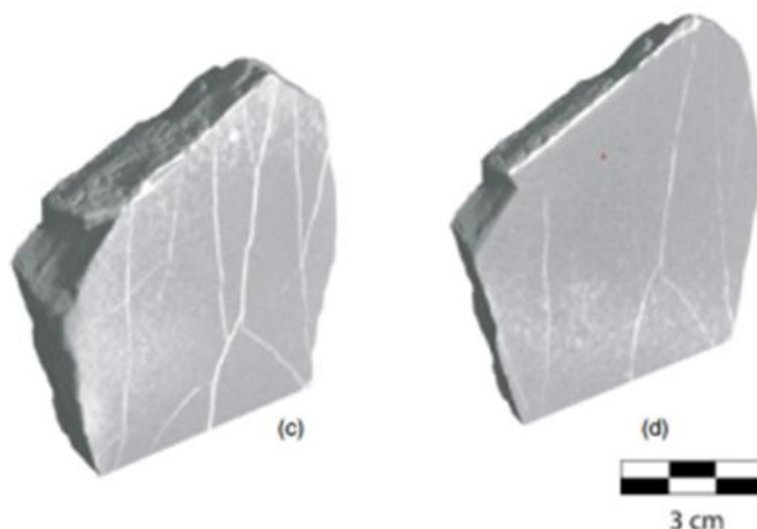
Fig. 7.21. (c) A slice of #23 at a depth of ~5 mm, showing a dense network of fissures visible as white lines. (d) A slice at a depth of ~10 mm, showing a decrease in the number of fissure lines with depth from the surface ( Courtesy: Jacobson et al, 2013).
