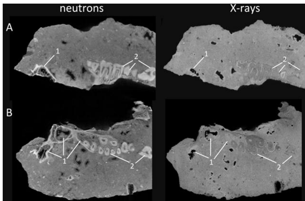
Fig. 7.5. Comparison of sagittal (A) and traverse (B) sections of the breccia block embedding STS 1039 obtained by neutron-based and X-Ray acquisitions performed at a similar resolution. While traditional X-Ray microtomography fails to fully discriminate bone from matrix (1) and dental tissues from matrix (2), the neutron-based microtomography successfully separates the biological and mineral materials.
