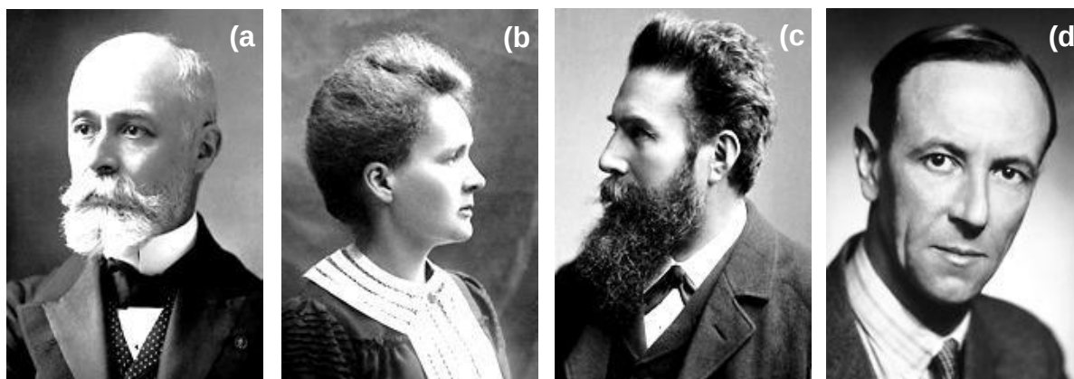
Figure App 1.1: Pioneers in radiation sciences: (a) Becquerel, (b) Curie, (c) Röntgen and (d) Chadwick.
