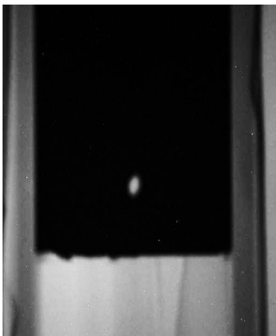
Figure 2.11: Demonstration of the successful application of a digital neutron radiography / tomography detection system using a LiF/ZnS(Ag) neutron sensitive scintillator and digital CCD camera: Quantitative quality inspection of a SAFARI-1 nuclear reactor control rod containing Cadmium (Black) could be achieved. (Courtesy: Necsa).
