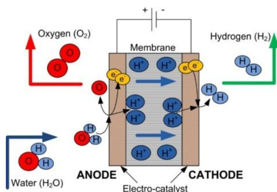
[Fig. 1. Schematic of a PEM electrolyser setup [1].
