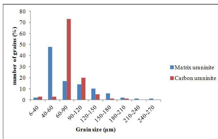
Figure 7 – Grain size distribution of uraninite in the matrix and the carbonaceous matter (Sebola, 2014)
