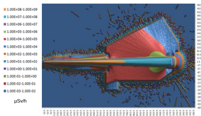
Fig.6. MCNP-X simulations showing the shielding capability for the upgraded SANRAD facility for whole neutron spectrum of SAFARI-1
