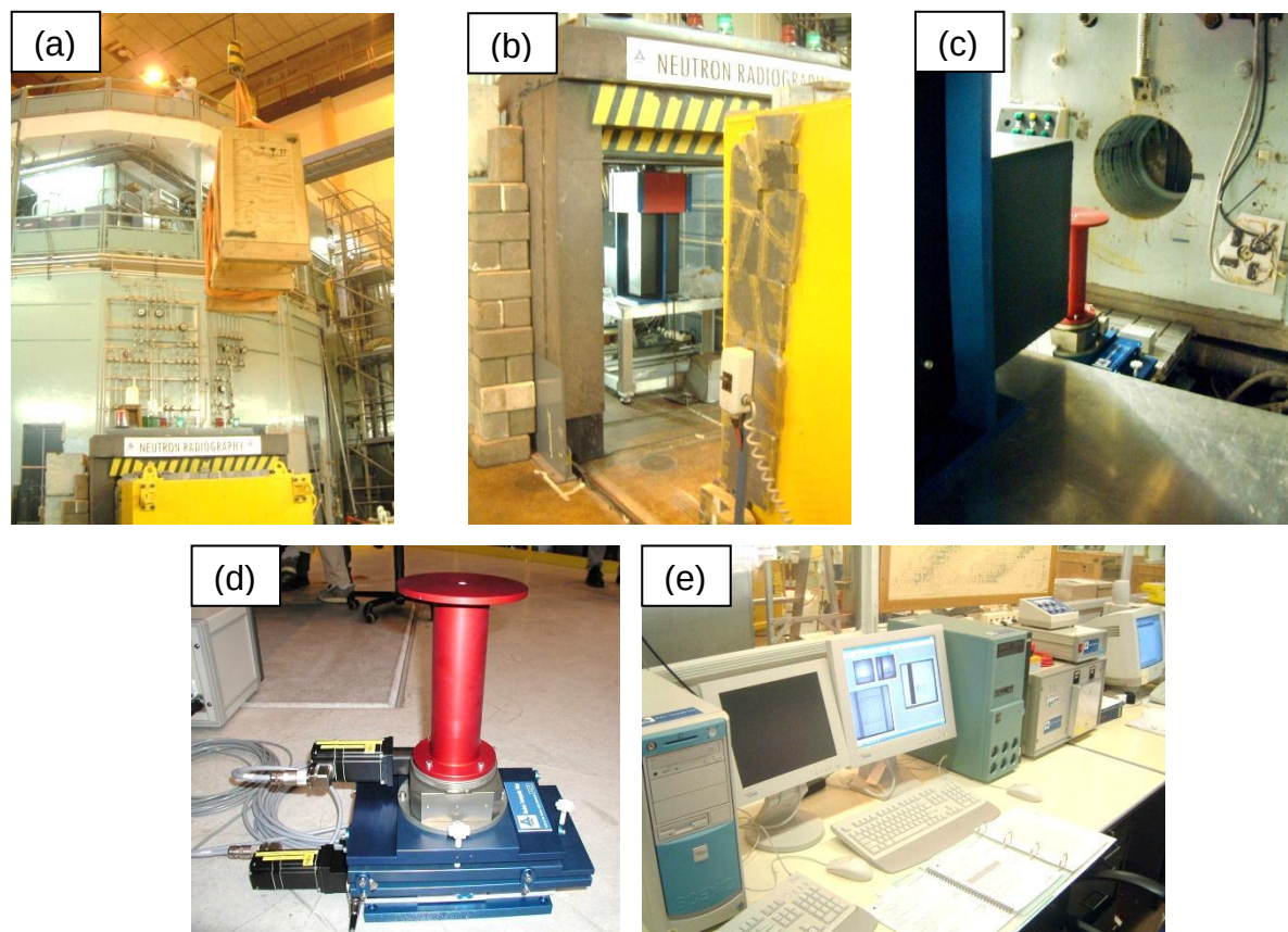
Figure 3.4: (a) Delivery of the neutron CT system from PSI in January 2003. (b) Outside view: CT system installed inside the NRAD bunker at beam port 2. (c) Inside view: Camera box – translation table – radiation beam port alignment. (d) Translation-rotation table, a key CT component required for acquisition of the projections at high angular resolution. (e) Computer infrastructure supporting CT acquisition and capturing of 2D projections at specific angular increments.
