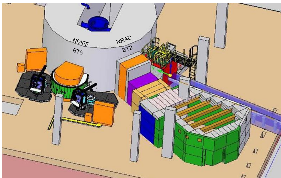
Figure 3.7: Monte Carlo model of the upgraded SANRAD facility at beam tube-2 in relation to the NDIFF (BT-5) and SANS (BT-1) facilities.
