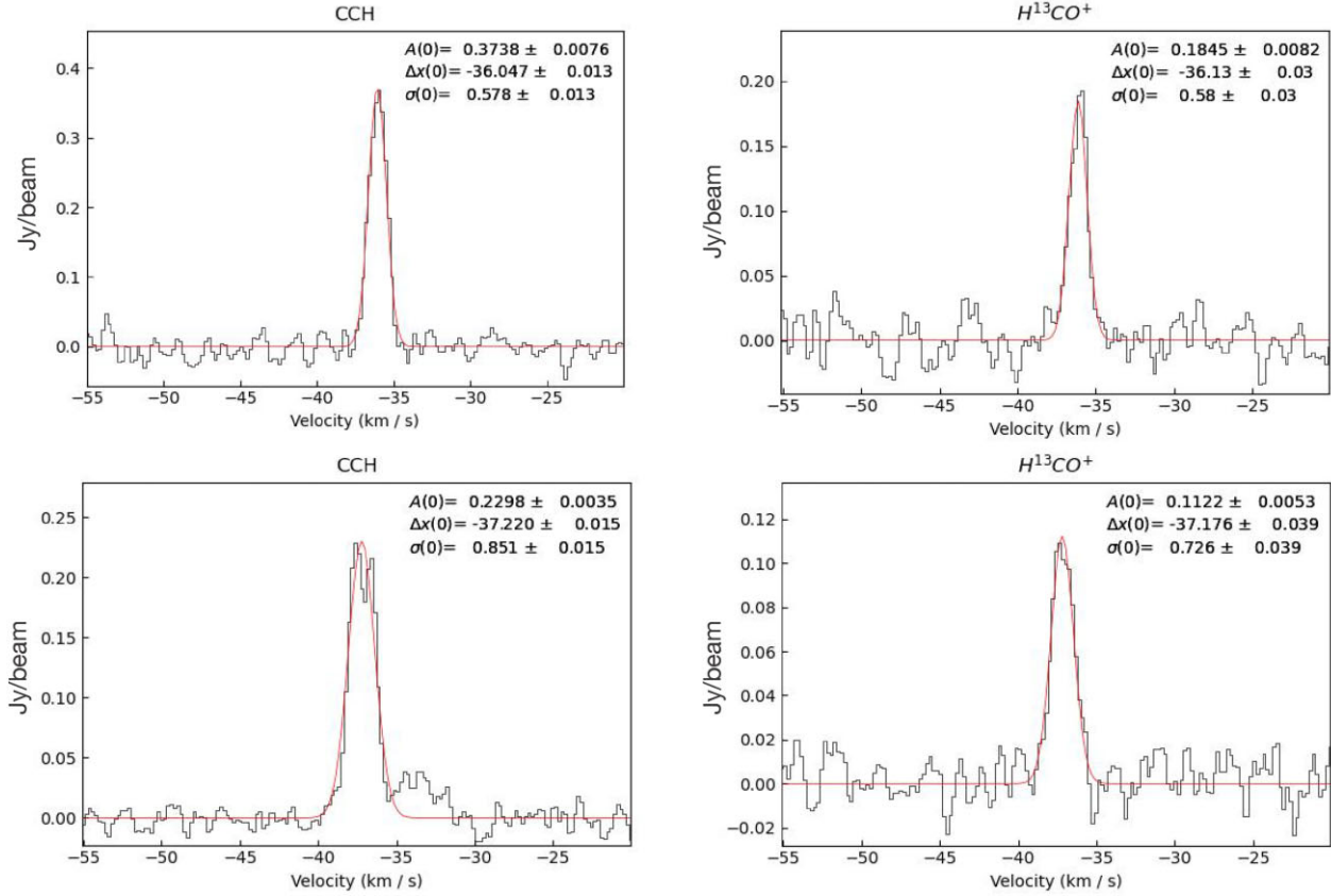
Figure 5. The spectrum of an exemplar source I18461-0113. Left and right panels show the CCH and H^{13}CO^+ , respectively. The data are shown in black, the Gaussian fits in red. The value and error of Gaussian fits parameters show in the upper right in each panel.
