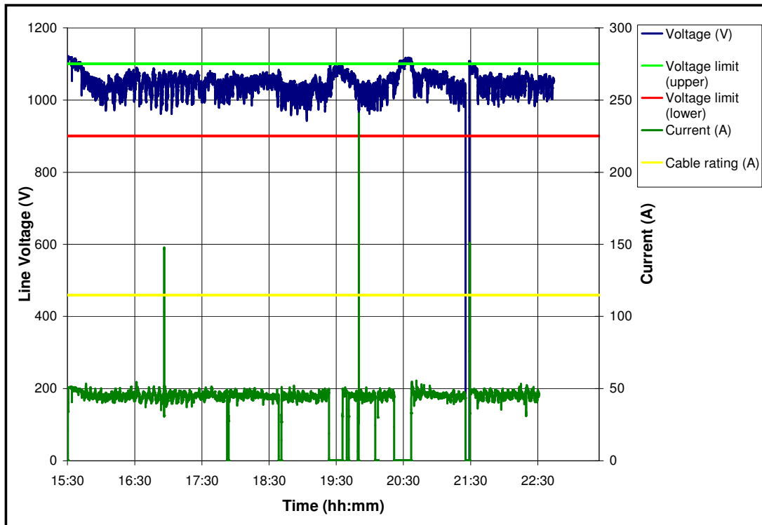
Figure G.1-11: Load current and voltage for a FB – 19 May 2005.
