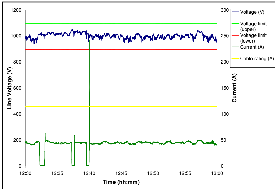
Figure G.1-18: Load current and voltage for a FB – 25 May 2005 (30 minute period).
