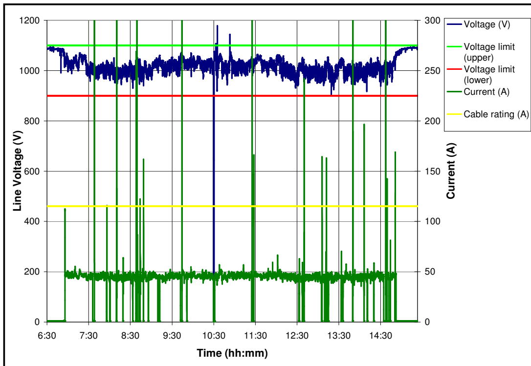
Figure G.1-17: Load current and voltage for a FB – 25 May 2005.
