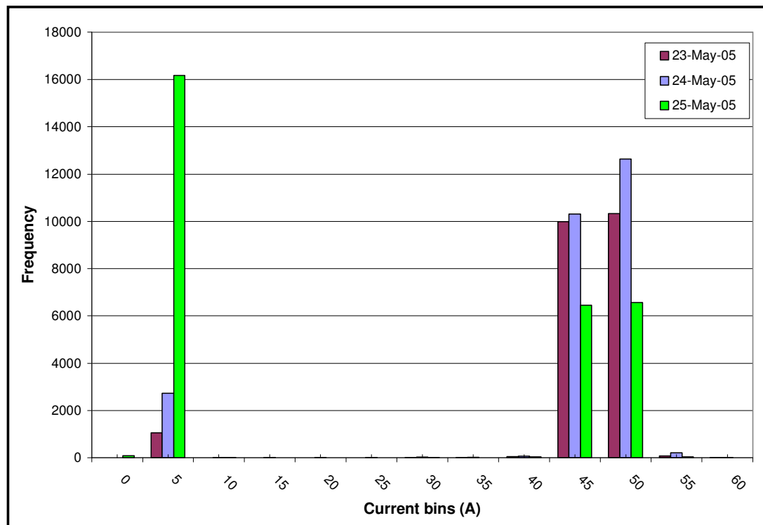
Figure G.2-4: Histogram for current consumed by a FB.
