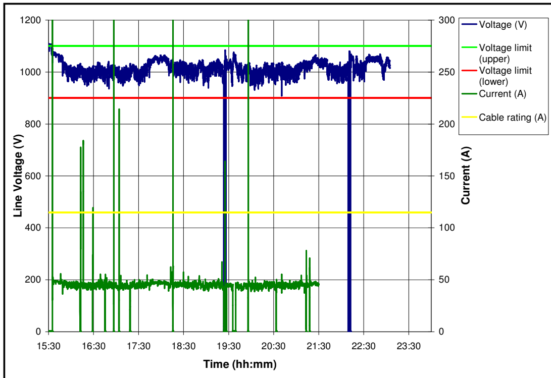
Figure G.1-19: Load current and voltage for a FB – 23 May 2005.
