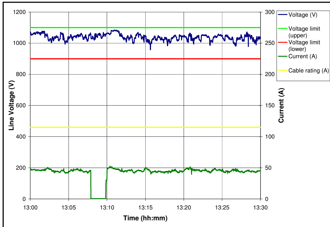
Figure G.1-6: Load current and voltage for a FB – 19 May 2005 (30 minute period).
