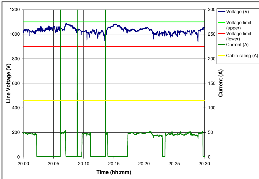
Figure G.1-22: Load current and voltage for a FB – 24 May 2005 (30 minute period).
