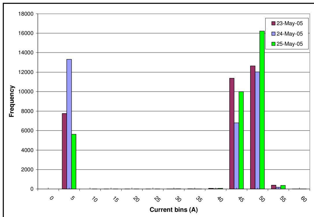
Figure G.2-3: Histogram for current consumed by a FB.
