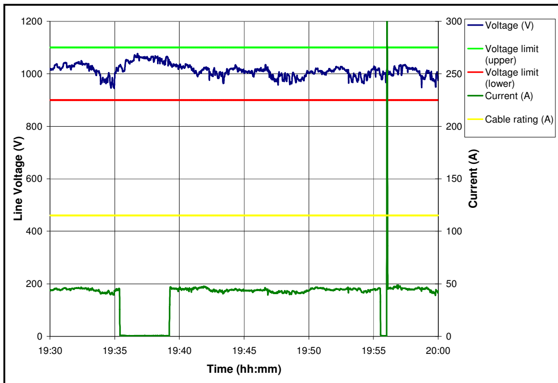
Figure G.1-20: Load current and voltage for a FB – 23 May 2005 (30 minute period).
