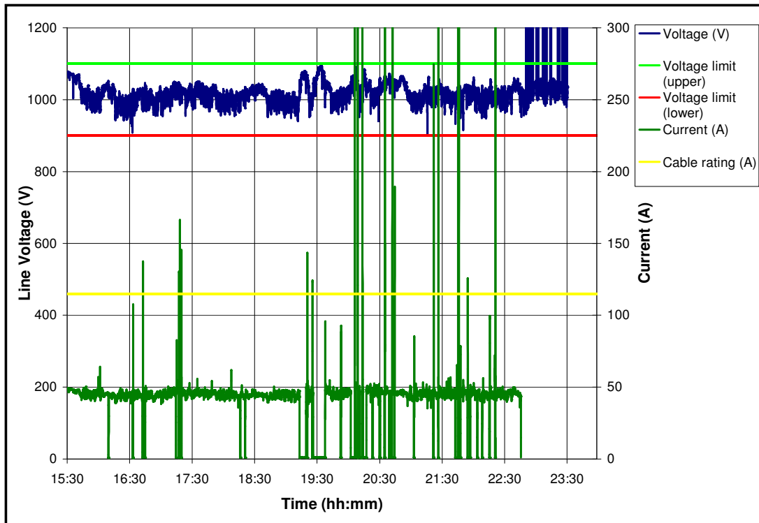
Figure G.1-21: Load current and voltage for a FB – 24 May 2005
