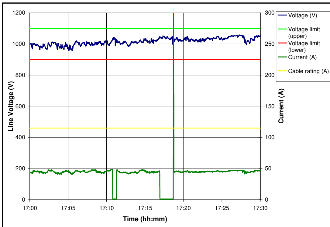
Figure G.1-24: Load current and voltage for a FB – 25 May 2005 (30 minute period).
