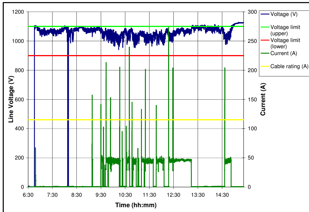
Figure G.1-1: Load current and voltage for a FB – 17 May 2005.
