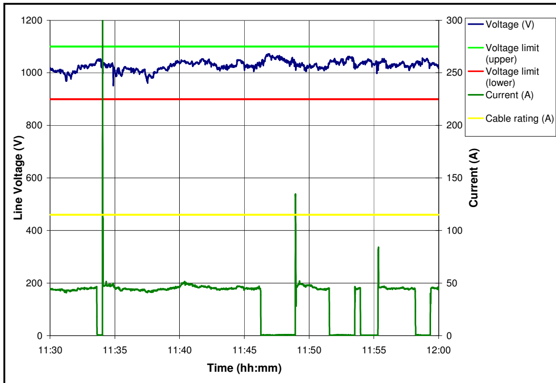
Figure G.1-14: Load current and voltage for a FB – 23 May 2005 (30 minute period).
