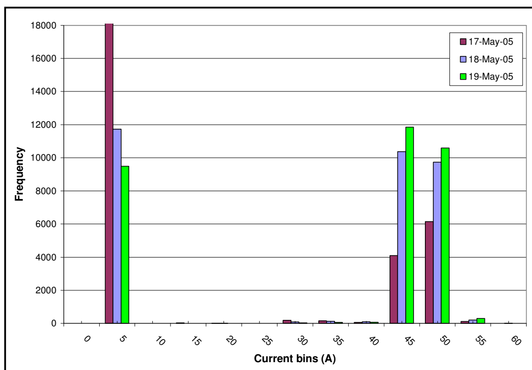
Figure G.2-1: Histogram for current consumed by a FB.
