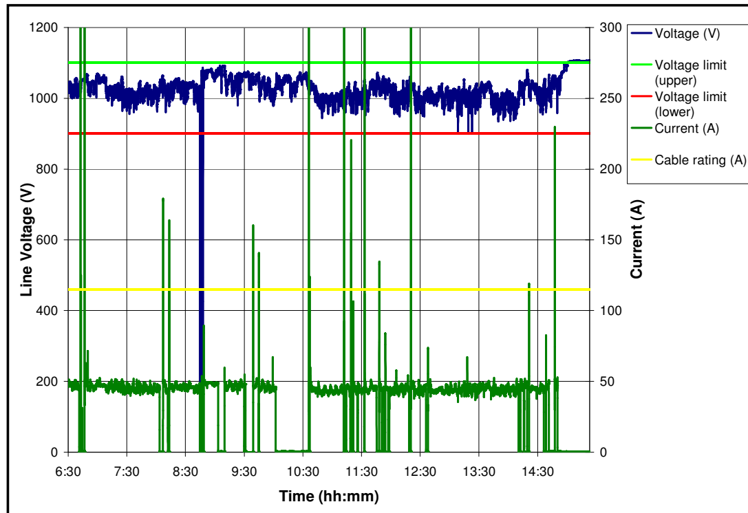
Figure G.1-13: Load current and voltage for a FB – 23 May 2005.
