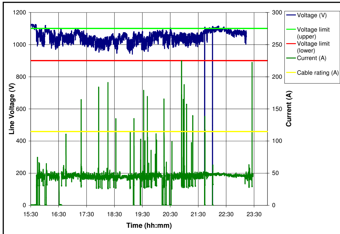
Figure G.1-7: Load current and voltage for a FB – 17 May 2005.
