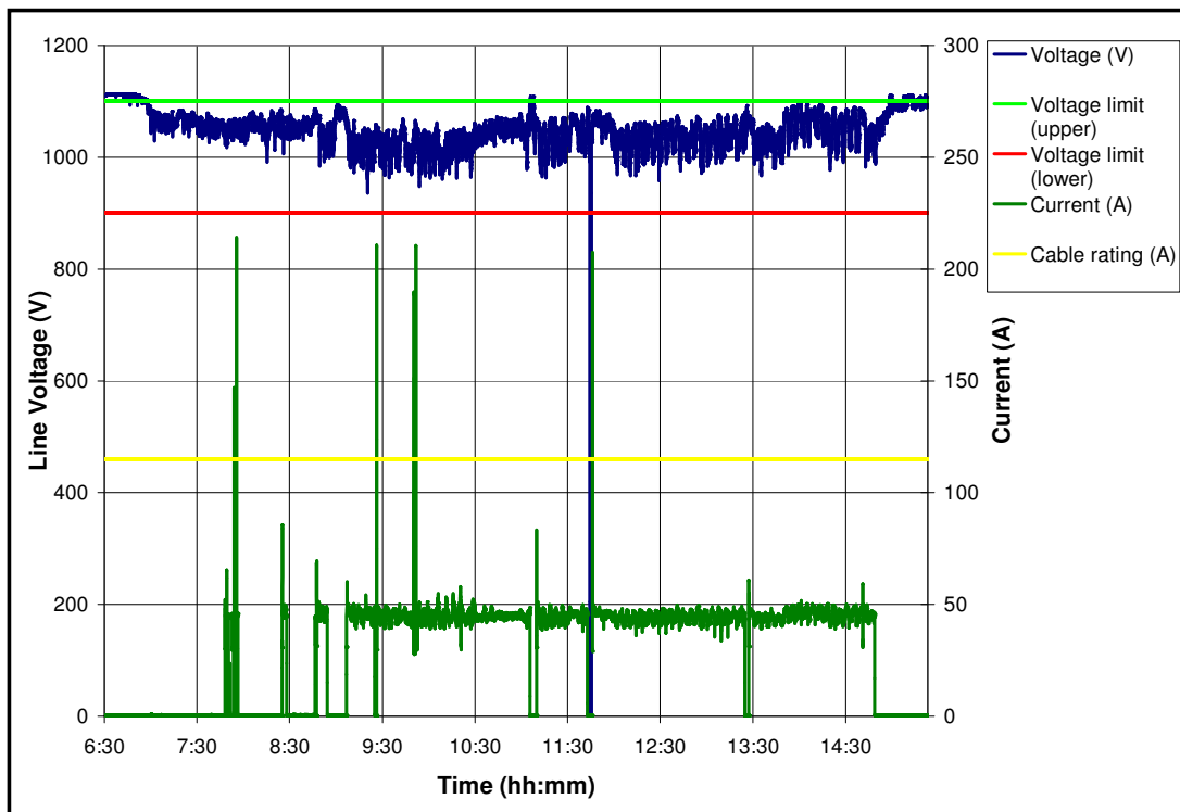
Figure G.1-3: Load current and voltage for a FB – 18 May 2005.
