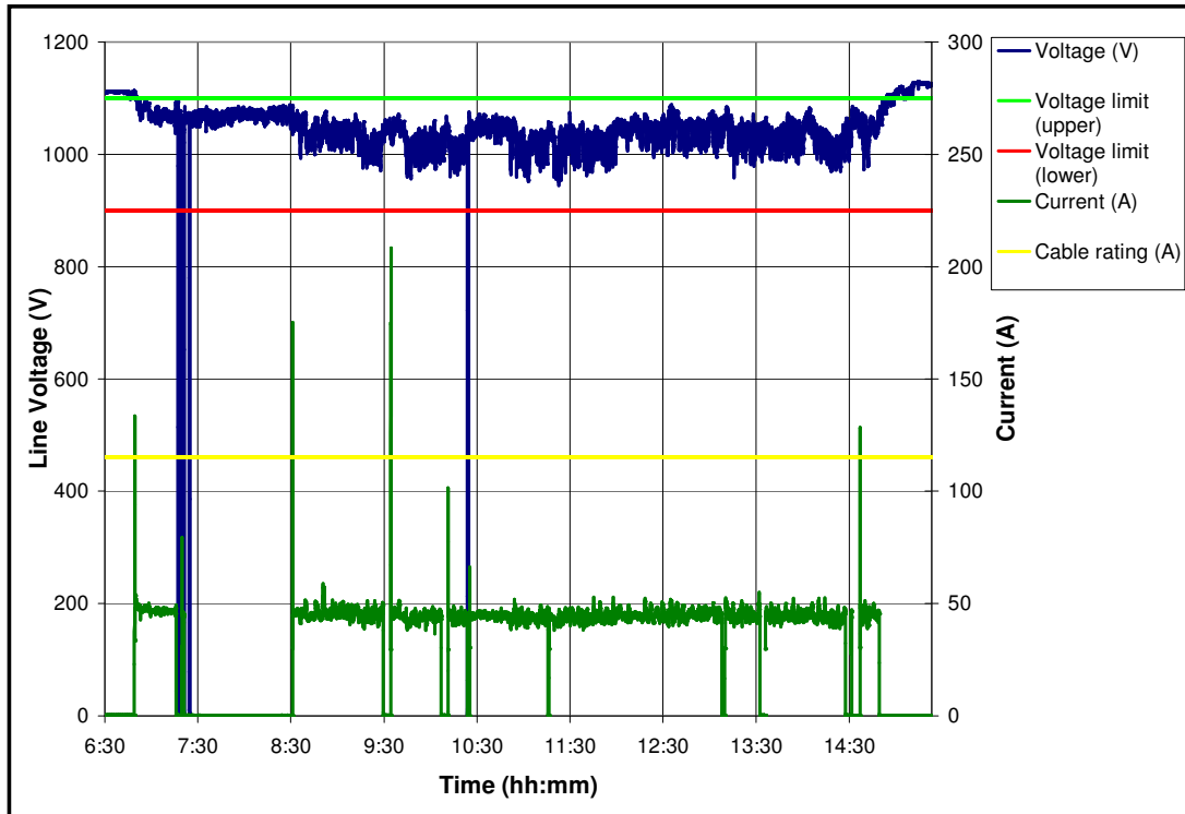
Figure G.1-5: Load current and voltage for a FB – 19 May 2005.
