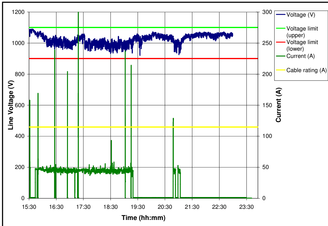
Figure G.1-23: Load current and voltage for a FB – 25 May 2005.
