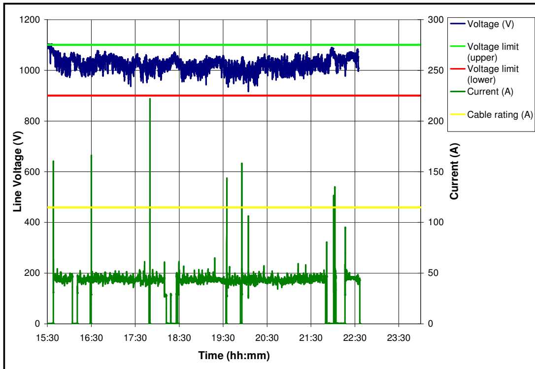
Figure G.1-9: Load current and voltage for a FB – 18 May 2005.
