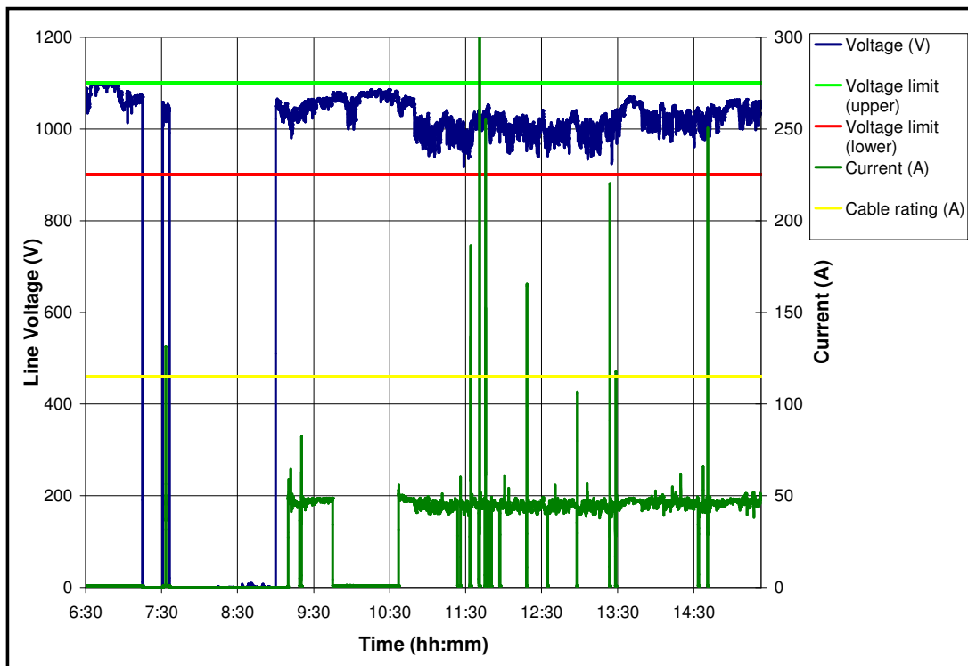
Figure G.1-15: Load current and voltage for a FB – 24 May 2005.
