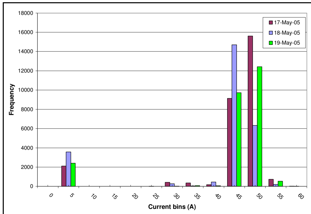
Figure G.2-2: Histogram for current consumed by a FB.
