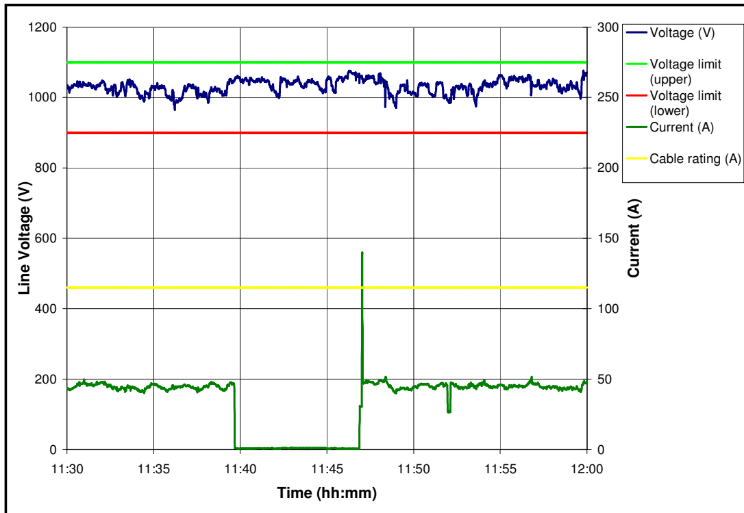
Figure G.1-2: Load current and voltage for a FB – 17 May 2005 (30 minute period).
