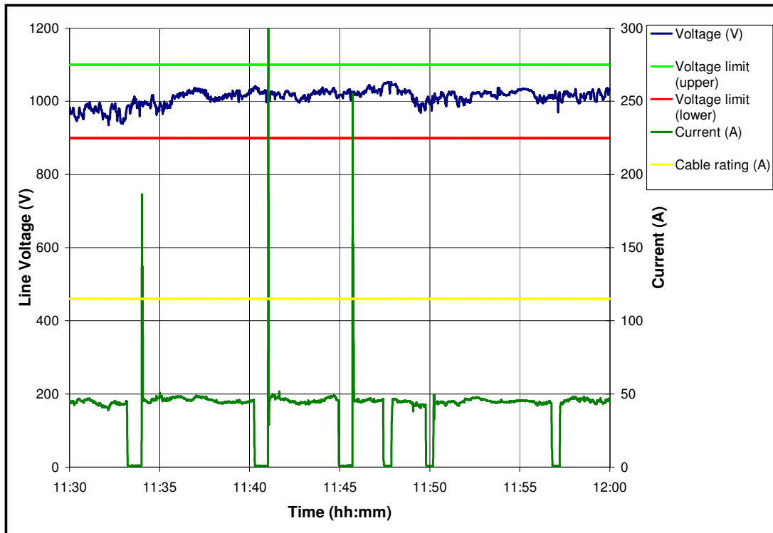
Figure G.1-16: Load current and voltage for a FB – 24 May 2005 (30 minute period).
