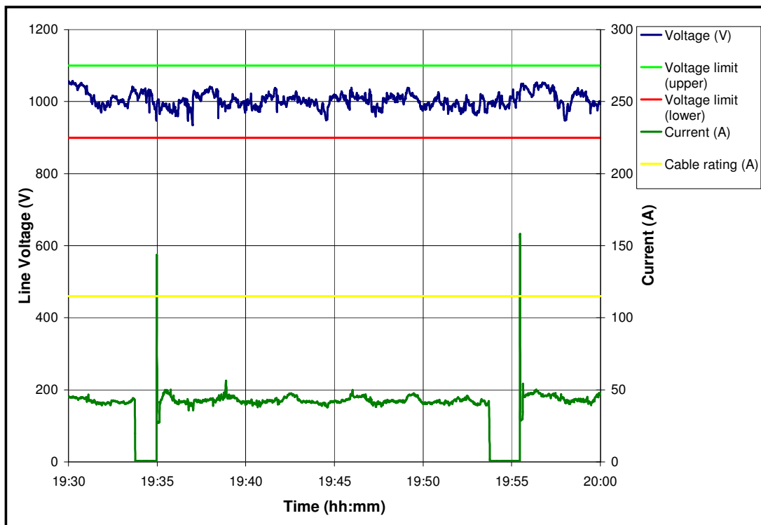
Figure G.1-10: Load current and voltage for a FB – 18 May 2005 (30 minute period).
