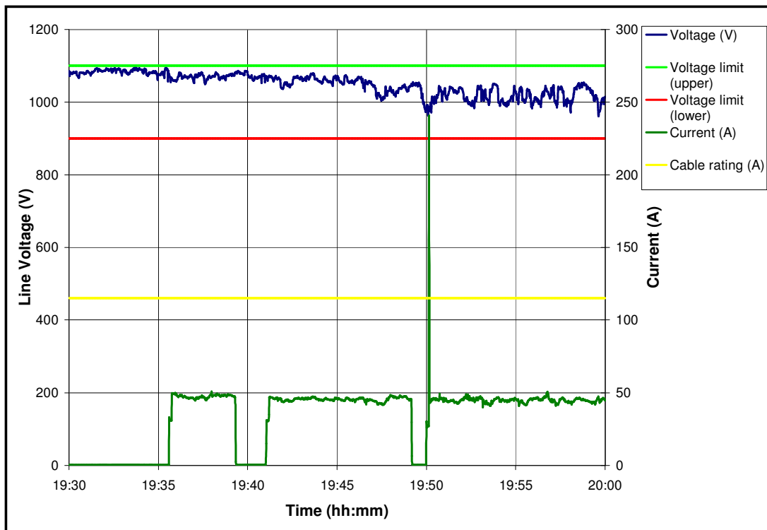
Figure G.1-12: Load current and voltage for a FB – 19 May 2005 (30 minute period).
