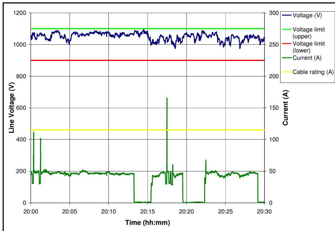
Figure G.1-8: Load current and voltage for a FB – 17 May 2005 (30 minute period).
