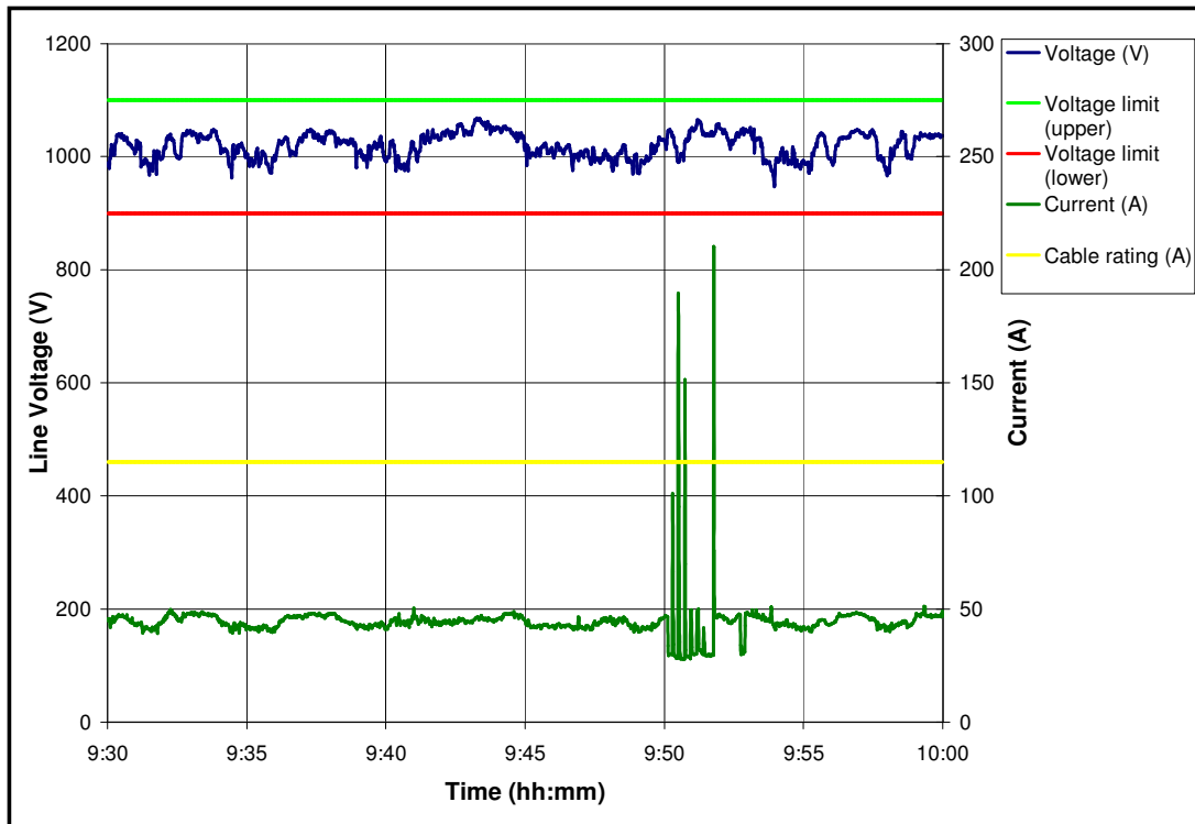
Figure G.1-4: Load current and voltage for a FB – 18 May 2005 (30 minute period).
