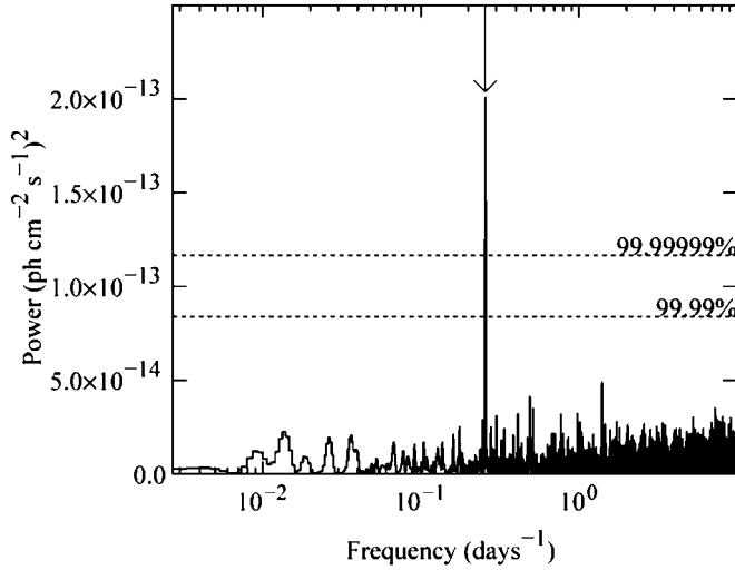
Figure 2. Power spectrum of the light curve. The arrow indicates the known orbital period of 3.90603 days (Casares et al. 2005). The dashed lines show the 99.99% and 99.99999% significance levels.
