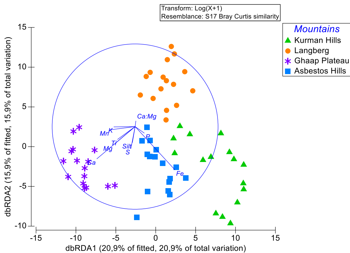
Figure C1. Distance based redundancy analysis (dbRDA) of ten soil parameters associated with compositional differences between mountain plant communities.
