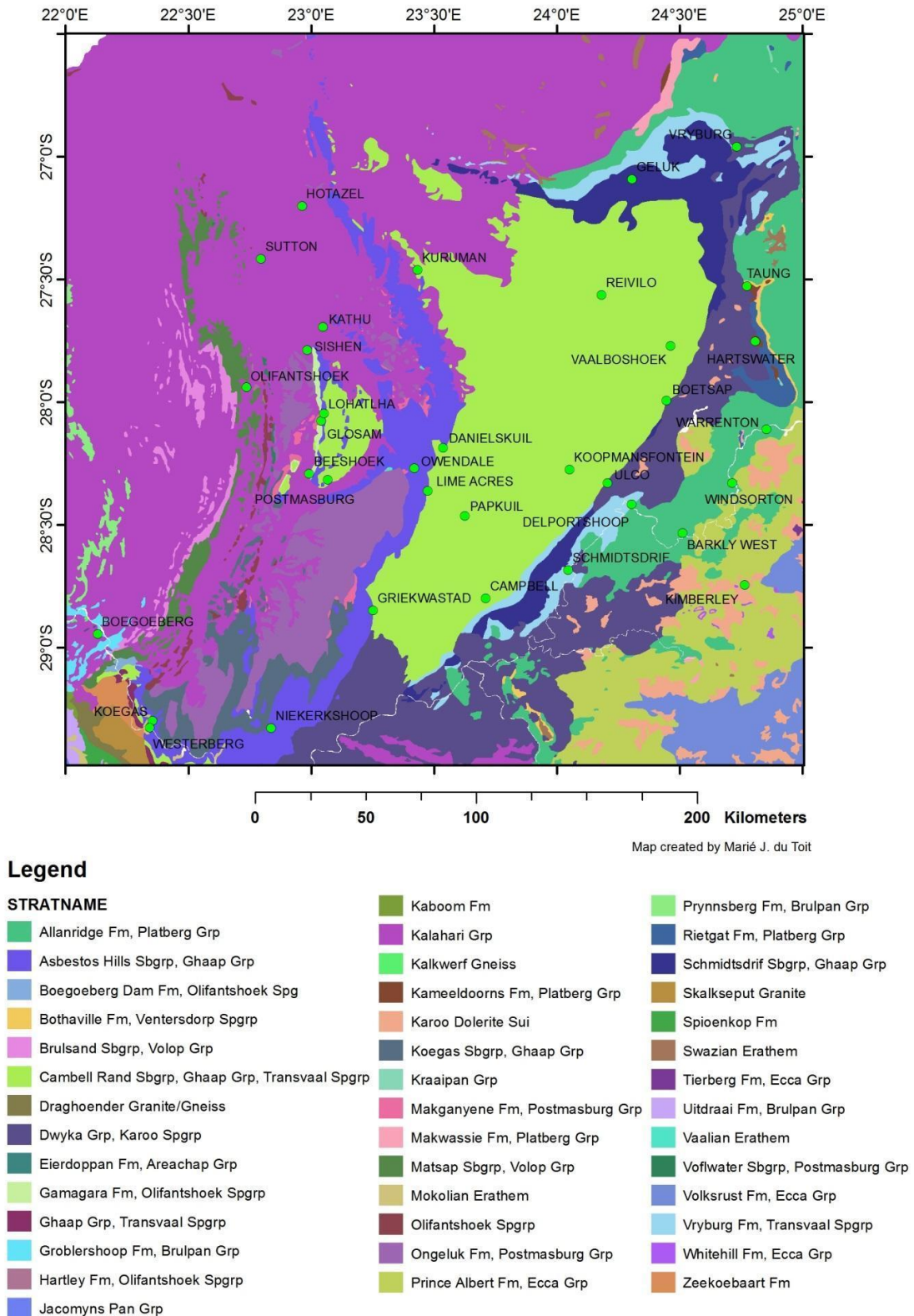
Figure 2.7. Geological map of the GW region (Council for Geosciences, 2008). Note that the Cambell Rand Subgroup as well as the Schmidtsdrif Subgroup, of the Ghaap Group, are within the Transvaal Supergroup. Grp, Group; Sbgrp, Subgroup; Spgrp, Supergroup.
