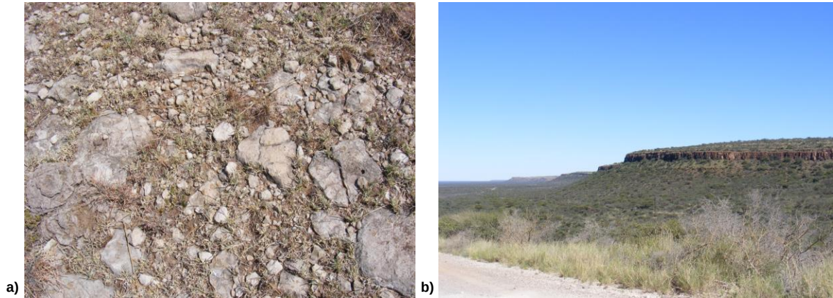
Figure 2.9. a) Exposed weathered dolomite of the Ghaap Plateau near Koopmansfontein and b) the escarpment slopes of the Ghaap Plateau beyond which a plateau develops. Photos: N. van Staden.
