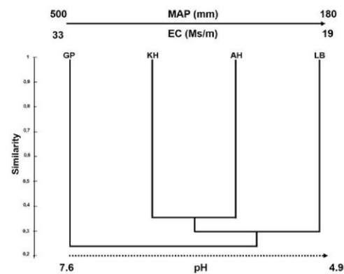
Figure 3. Dendrogram of Jaccard Similarity indicating the relatedness of each mountain ecosystem across the pH-, nutrient- and rainfall gradient. Clusters were based on presence and absence of sampled plant species.
