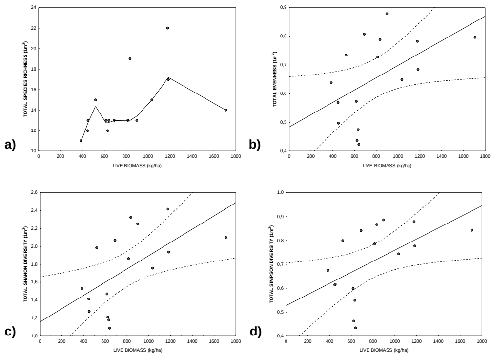
Figure D4. Local diversity-biomass relationships of total species diversity indices for the Ghaap Plateau, a) species richness, b) evenness, c) Shannon- and d) Simpson diversity.
