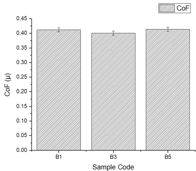
Fig. 8 Average CoF for Ti–Al–Nb alloys
