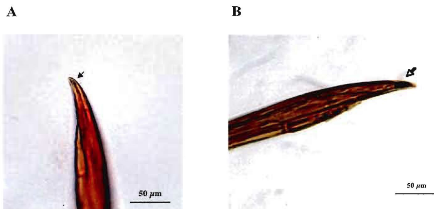
Figure 3.4. Unpaired (dorsal valve) of Cotesia sesamiae (A) and Cotesia flavipes (B) after silver staining. For each parasitoid species, the tip appeared silver stained (see arrow) due to numerous dome-shaped sensilla concentrated on it.
