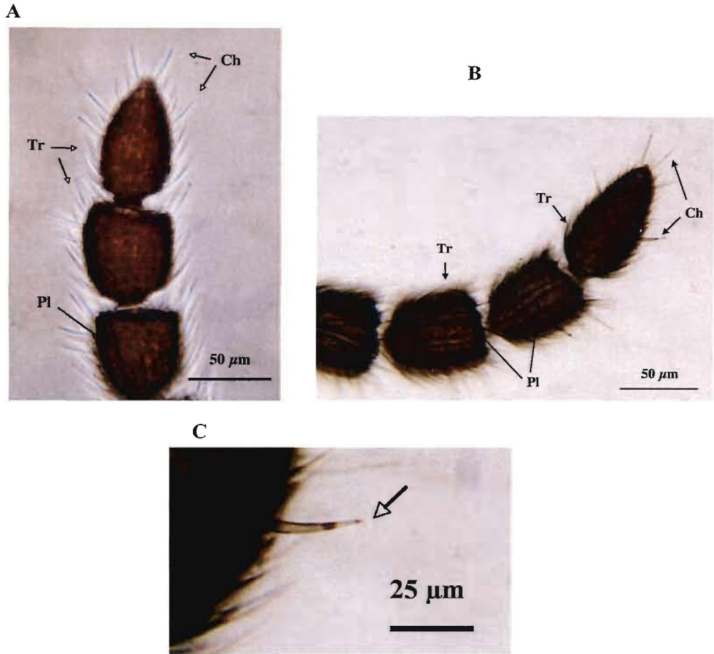
Figure 3.2. Distal antennomeres of adult females of Cotesia sesamiae (A) and Cotesia flavipes (B) observed by optic microscopy after silver staining procedure, showing the uniporous sensilla chaetica (Ch) and the sensilla placodea (Pl) along the longitudinal axis silver stained. Close-up of a long and curved sensillum chaeticum (C) located on the last antennomere of C. flavipes showing the silver nitrate which penetrated from the single pore on its tip (see arrow).
