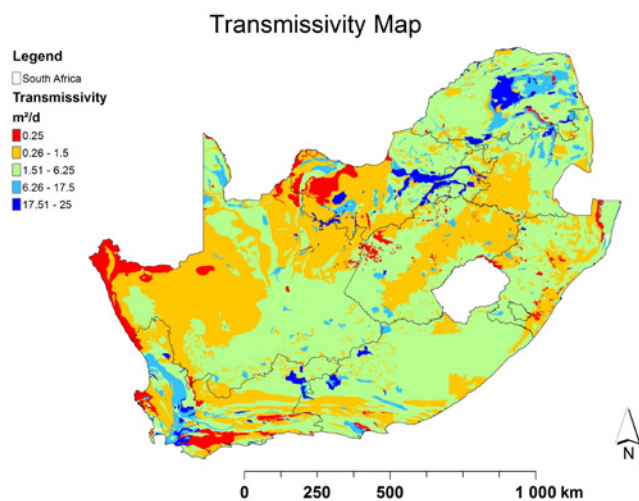
Figure 12 Transmissivity map
