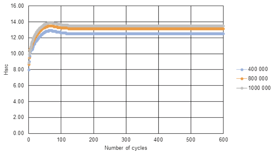
Figure 8: Full core model fission source convergence.
