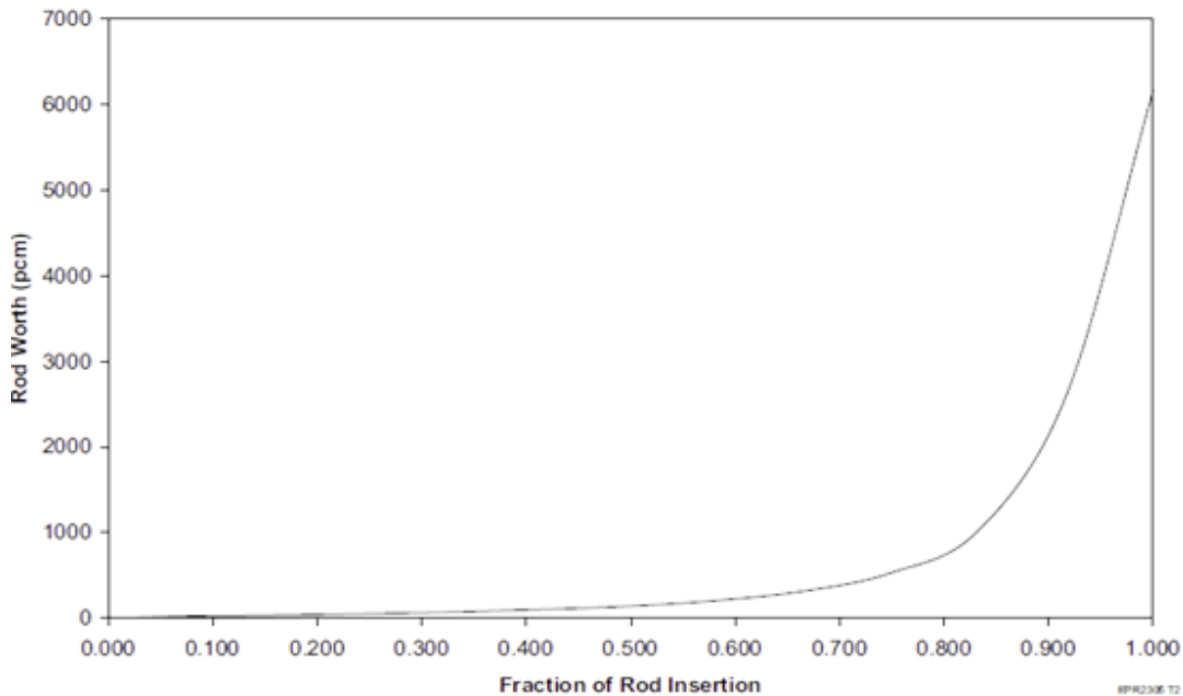
Figure 14: EPR's control rod worth (AREVA, 2012).
