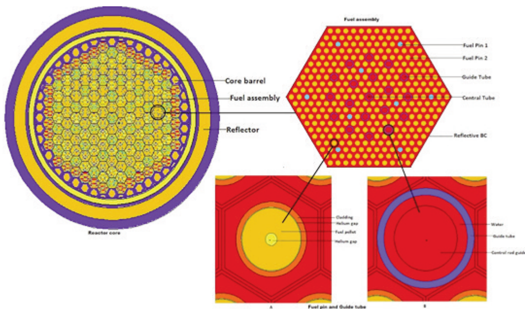
Figure 6: VVER-1000 core layout showing the positions of the fuel pins within the fuel assembly, and the position of the fuel assembly within the reactor core.
