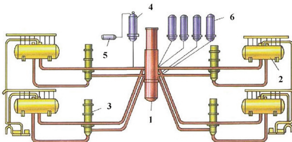
Figure 1: VVER schematic diagram. 1. Reactor, 2. Steam generator, 3. Main coolant pump, 4. Pressuriser, 5. Pressurizer relief tank, 6. Accumulator (Agrawal, et al, 2005).
