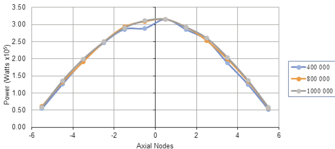
Figure 10: Axial power profile.
