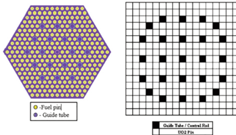
Figure 4: VVER-1000 (left) (Kostal, et al., 2013) and typical PWR (right) (Rahnema & Douglass, 2009) fuel assembly.
