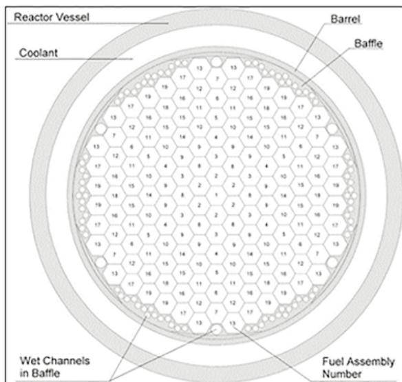
Figure 2: Reactor cores, (Mahlers, 2009).
