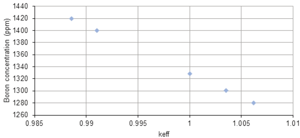
Figure 11: Calculation of the critical boron concentration.
