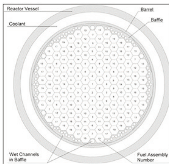
VVER-1000 Core
