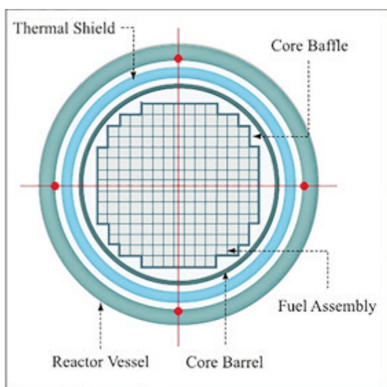
Westinghouse PWR- core
