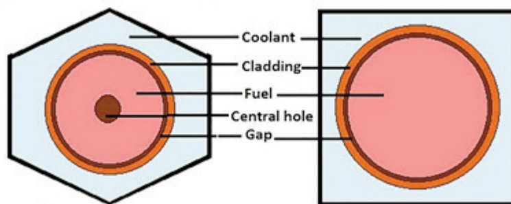
Figure 5: Fuel pellet (Mozafari & Faghihi, 2013).
