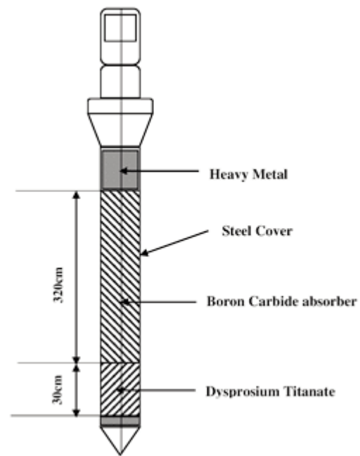
Figure 12: Control rod (Tikhonov, 2011).
