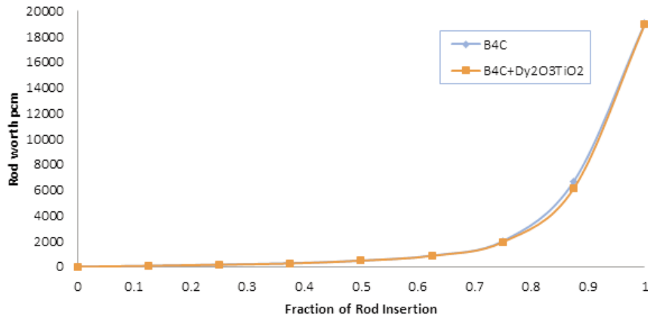
Figure 13: Rod worth.
