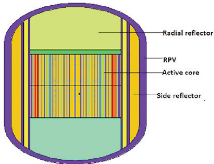
Figure 7: Reactor pressure vessel and internals showing the layout of the various components within the reactor pressure vessel.
