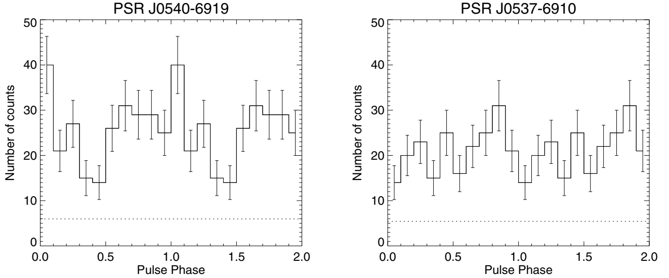
Fig. 7. Lightcurves obtained for PSR J0540–6919 (left) and PSR J0537–6910 (right) for the energy range 200 MeV–20 GeV using an event selection radius of 0.5^\circ around the nominal pulsar positions. The data are binned into 10 phase bins. The dotted lines indicate the sum of the expected contributions from extragalactic and Galactic diffuse emissions and residual instrumental background.
