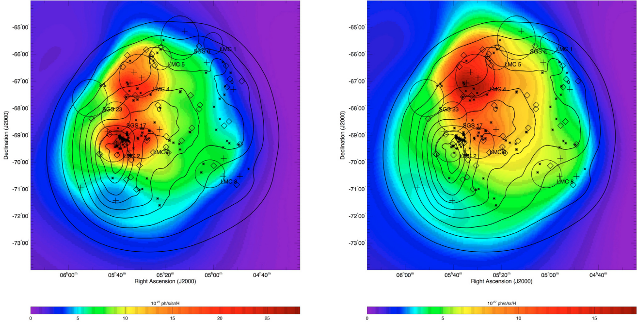
Fig. 10. Integrated >100 MeV emissivity maps of the LMC in units of 10^{-27} ph s ^{-1} sr ^{-1} H-atom ^{-1} for \mathcal{H}_1 (left panel) and \mathcal{H}_2 (right panel). An adaptive smoothing with a signal-to-noise ratio of 5 has been applied to reduce statistical fluctuations. Note that the colour scales are not the same for the two images. As contours we show N(H) column densities convolved with the LAT point spread function that are linearly spaced from 10%–90% of the maximum in steps of 10%. Symbols indicate the locations of pulsars (pluses) from ATNF catalogue version 1.36 (Manchester et al. 2005), supernova remnants (diamonds) from Rosa Williams web page http://www.astro.illinois.edu/projects/atlas/index.html , Wolf-Rayet stars (stars) from the fourth catalogue of Breysacher et al. (1999), and supergiant shells (circles) from Staveley-Smith et al. (2003).
