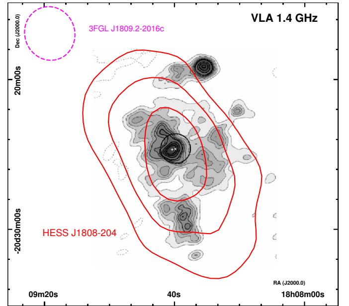
Fig. 5. VLA 1.4 GHz radio image of the radio nebula G10.0–0.3 (contour levels at -3, 2, 4, 6, 8, 10, 12, 14, 20, 25, 30 \times 1.56 \text{ mJy/beam} ; black circle indicating an ASCA X-ray source location) from Kulkarni et al. (1994) with red solid VHE \gamma -ray contours of HESS J1808–204 (as per Fig. 1). The 68% location error of 3FGL J1809.2–2016c is indicated by the magenta dashed ellipse, and locations of SGR 1806–20 (x) and LBV 1806–20 (+) are indicated.
