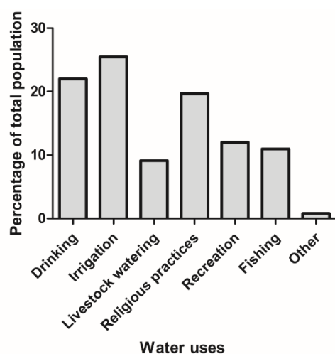
Figure 11. Future proposed uses of the Wonderfonteinspruit
