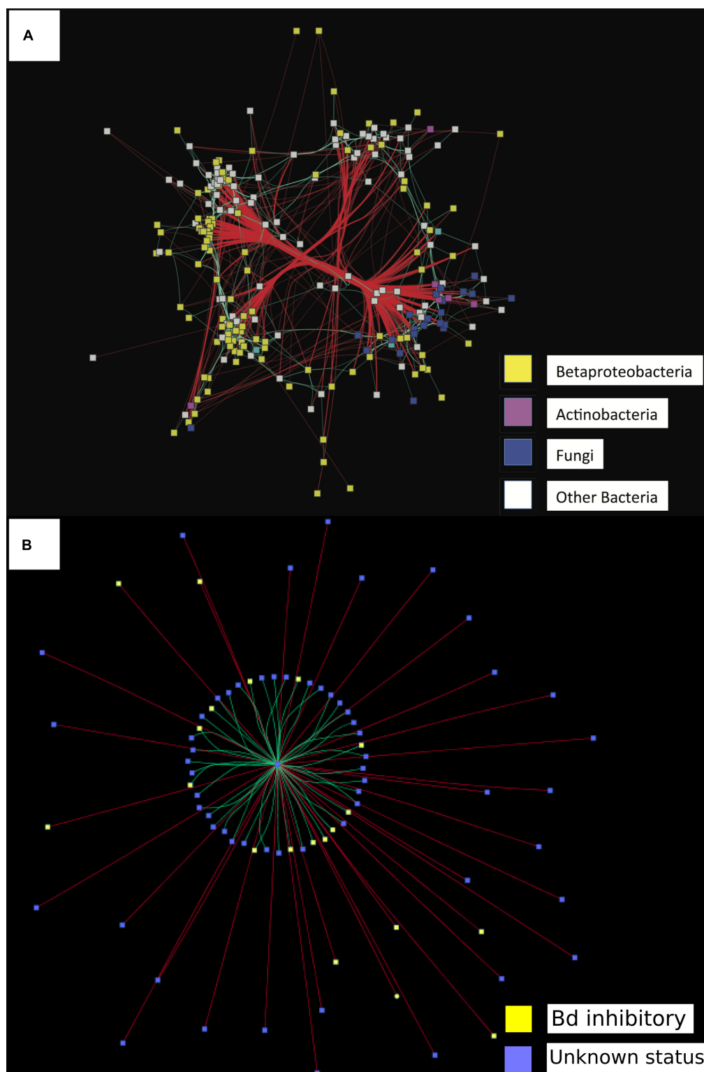
FIGURE 2 | Data showing proof of concept of a network analysis to identify correlations among bacterial and fungal operational taxonomic units (OTUs) on amphibian hosts. Network analyses depicting significantly correlated bacterial and fungal OTUs (SparCC r > 0.35 ). All square nodes represent OTUs (either bacteria or fungi). Red lines indicate negative correlations between two OTUs. Turquoise lines indicate positive correlations between two OTUs. (A) Assessing directionality of interactions found between all bacteria and fungal taxa. Figure adapted from Kueneman et al. (2015). Yellow = Betaproteobacteria, purple = Actinobacteria, blue = Fungi, white = other bacterial OTUs. (B) Assessing directionality of interactions found between all bacterial interactions and Pathogen Bd . Yellow = bacteria that inhibit Bd in co-culture, blue = Unknown interaction with Bd in co-culture. Center of network = fungal pathogen Bd .
