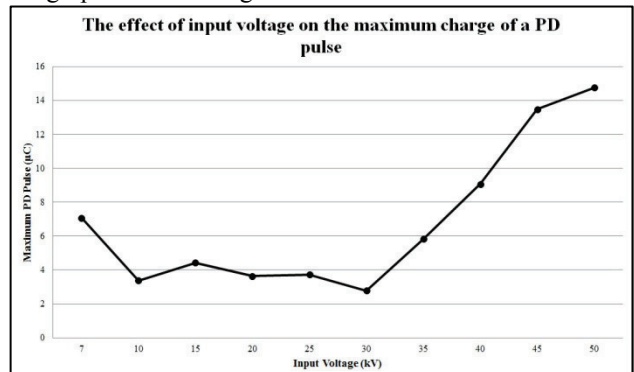
Figure 7: Effect of input voltage on the maximum PD amplitude
