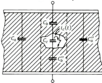
Figure 5: Capacitor configuration for basic model [12]
