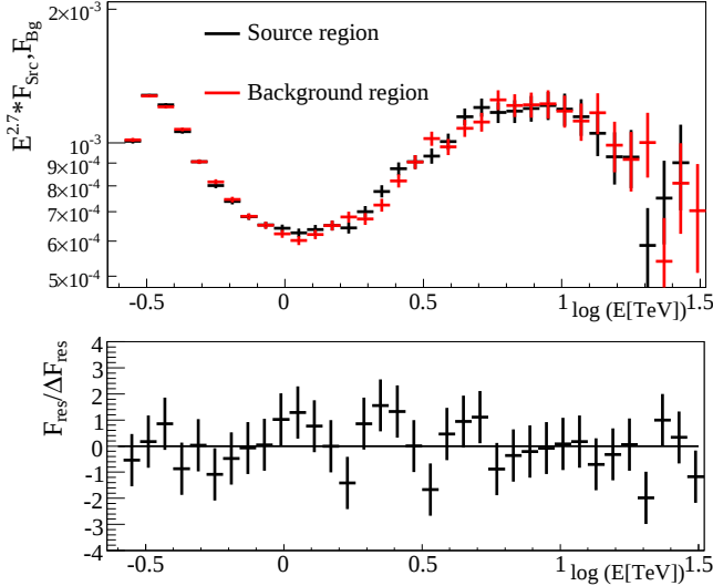
FIG. 3. Top panel: Reconstructed differential flux F_{\text{src}}/F_{\text{Bg}} , weighted with E^{2.7} for better visibility, obtained for the source and background regions as defined in the text. The units are \text{TeV}^{1.7} \text{ m}^{-2} \text{ s}^{-1} \text{ sr}^{-1} . Due to an energy-dependent selection efficiency and the use of effective areas obtained from \gamma -ray simulations, the reconstructed spectra are modified compared to the cosmic-ray power-law spectrum measured on Earth. Bottom panel: Flux residua F_{\text{res}}/\Delta F_{\text{res}} , where F_{\text{res}} = F_{\text{src}} - F_{\text{Bg}} and \Delta F_{\text{res}} is the statistical error on F_{\text{res}} . The residual flux is compatible with a null measurement. Comparable null residuals are obtained when varying the radius of the source region, subdividing the data set into different time periods or observation positions, or analyzing each half of the source region separately.
