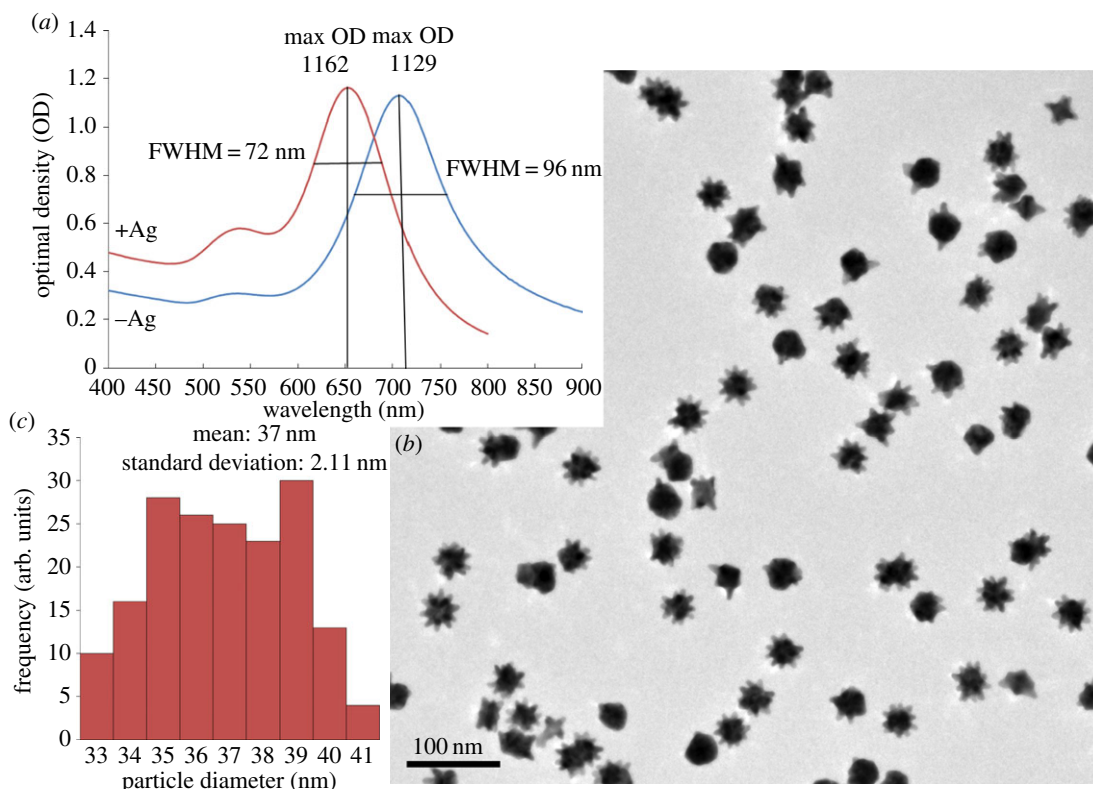
Figure 3. Particle size distribution and monodispersity analysis. (a) UV–Vis spectra indicating the full width at half maximum value for both –Ag and +Ag nanostars. (b) TEM image of +Ag nanostars. (c) Particle diameter distribution using TEM images.
