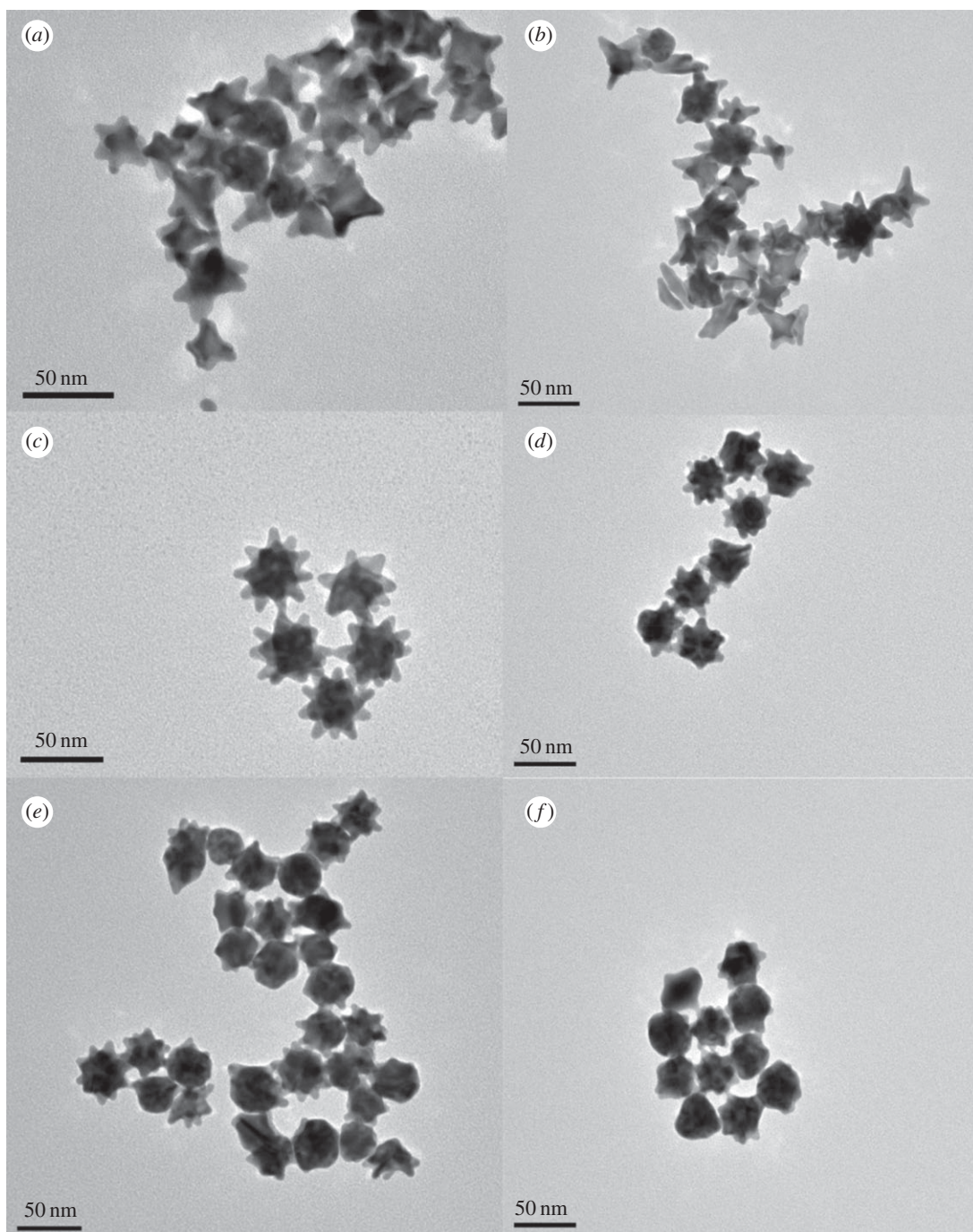
Figure 2. Representative HR-TEM images of the nanoparticle morphology. (a) 0 \mu\text{l} -Ag , (b) 2 \mu\text{l} +Ag , (c) 4 \mu\text{l} +Ag , (d) 6 \mu\text{l} +Ag , (e) 8 \mu\text{l} +Ag , and (f) 10 \mu\text{l} +Ag gold nanostars.
