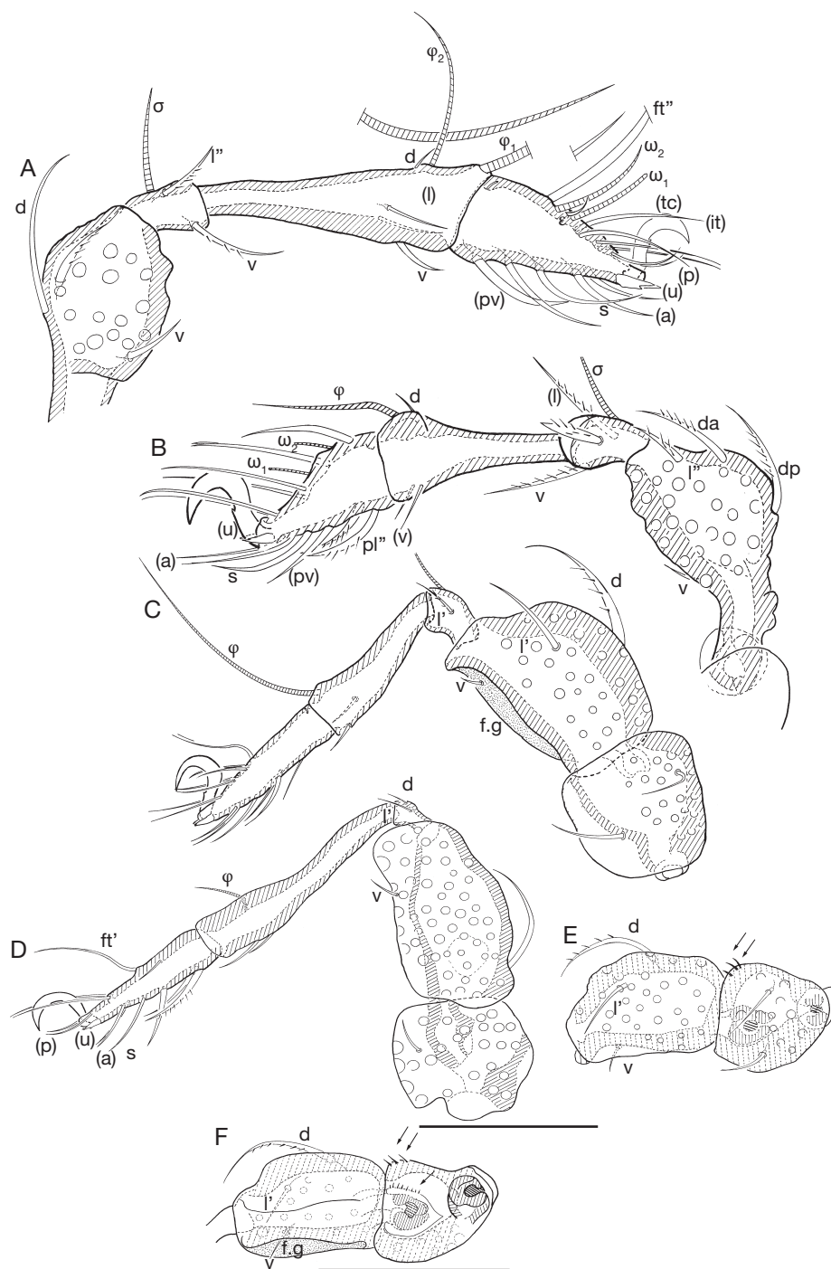
FIG. 18. — Congocephus extactesi n. sp. adult.: A , legs I, antiaxial; B , leg II, antiaxial; C , legs III, antiaxial; D , legs IV, antiaxial; E , trochanter-femur, leg III, antiaxial; F , trochanter-femur, leg III, paraxial. Abbreviations: see Material and methods. Scale bars: A-D, 50 \mu m; E, F, 70 \mu m.
