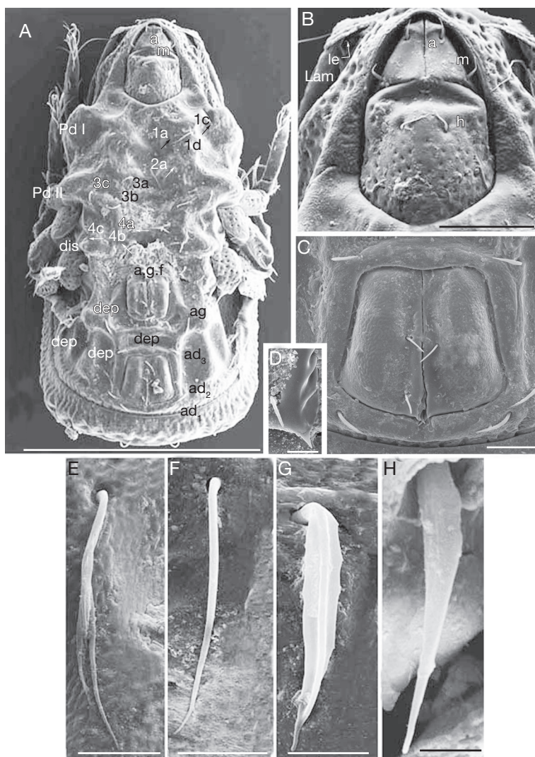
FIG. 14. — Congocepheus ektatesi n. sp. adult, scanning electron micrographs: A , ventral view; B , infracapitulum; C , anal zone; D , anal, sharp end; E , aggenital setae; F , epimeric setae; G , adanal setae; H , anal setae. Abbreviations: see Material and methods. Scale bars: A, 300 \mu m; B, 50 \mu m; C–E, 20 \mu m; F, 30 \mu m; G, 10 \mu m; H, 5 \mu m.
