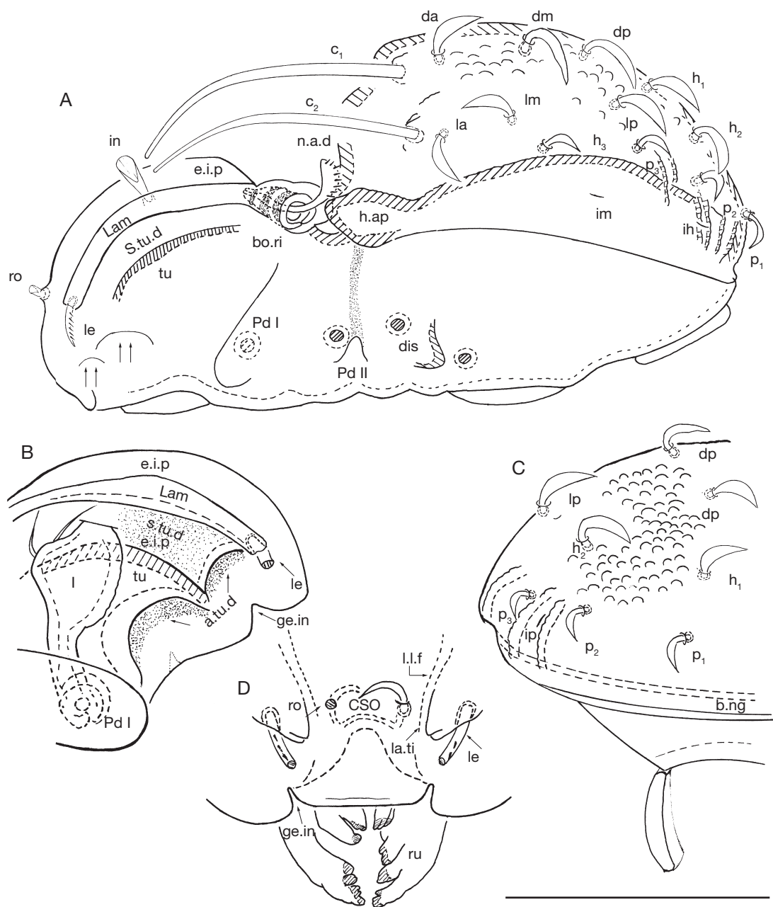
FIG. 4. — Congocephus involutus Mahunka, 1997 adult: A , lateral view; B , tutorial zone, lateral view; C , posterior view; D , frontal view. Abbreviations: see Material and methods. Scale bar: 100 \mu m.
