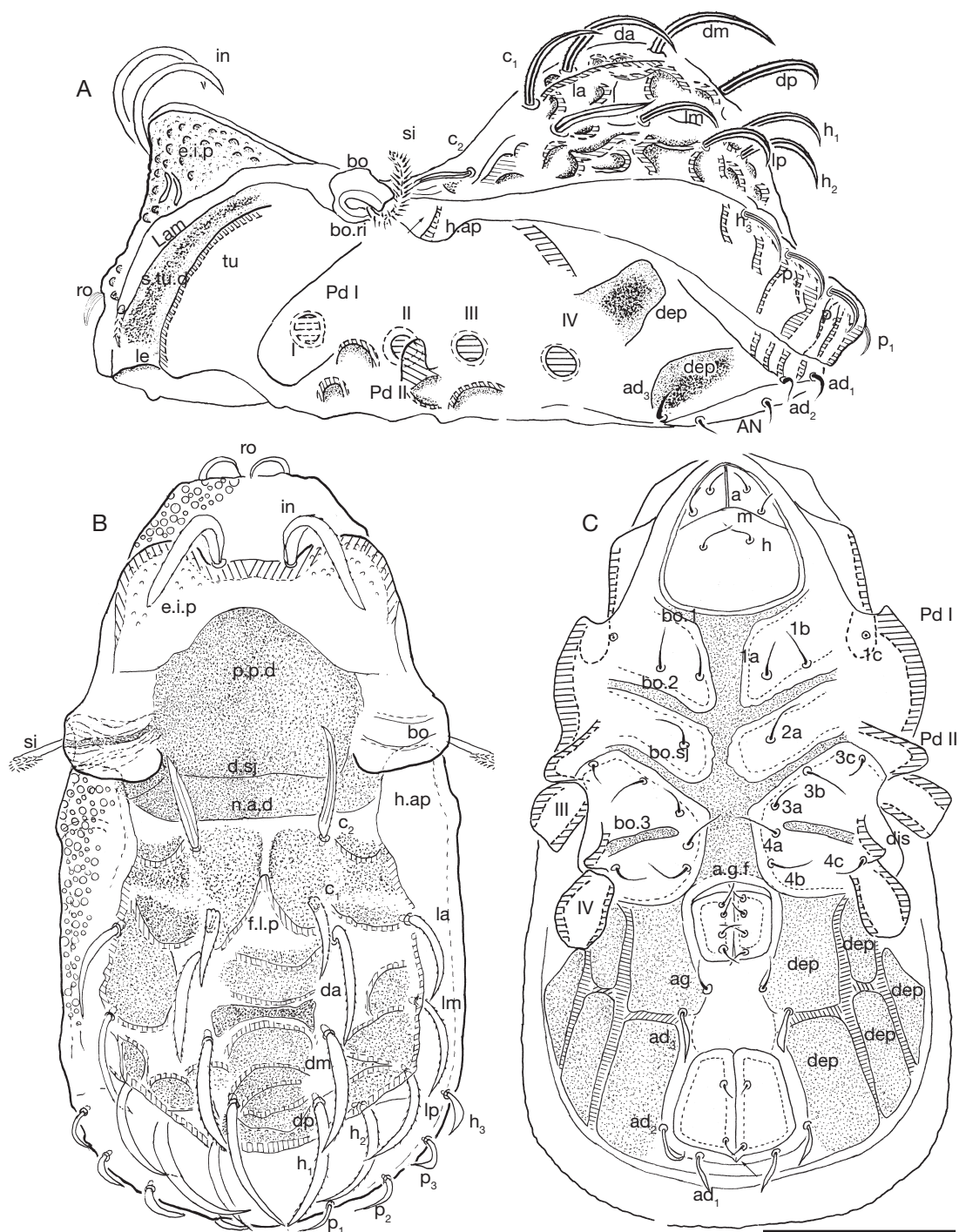
FIG. 8. — Congocepeus gabonensis n. sp. adult: A , lateral view; B , dorsal view; C , ventral view. Abbreviations: see Material and methods. Scale bar: 100 μm.
