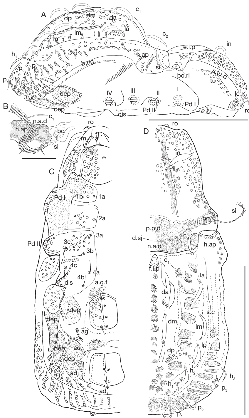
FIG. 13. — Congocepheus extactesi n. sp. adult: A , lateral view; B , zone notogastral anterior depression, detail; C , ventral view; D , dorsal view. Abbreviations: see Material and methods. Scale bars: A, 200 \mu m; B, 30 \mu m; C, D, 230 \mu m.
