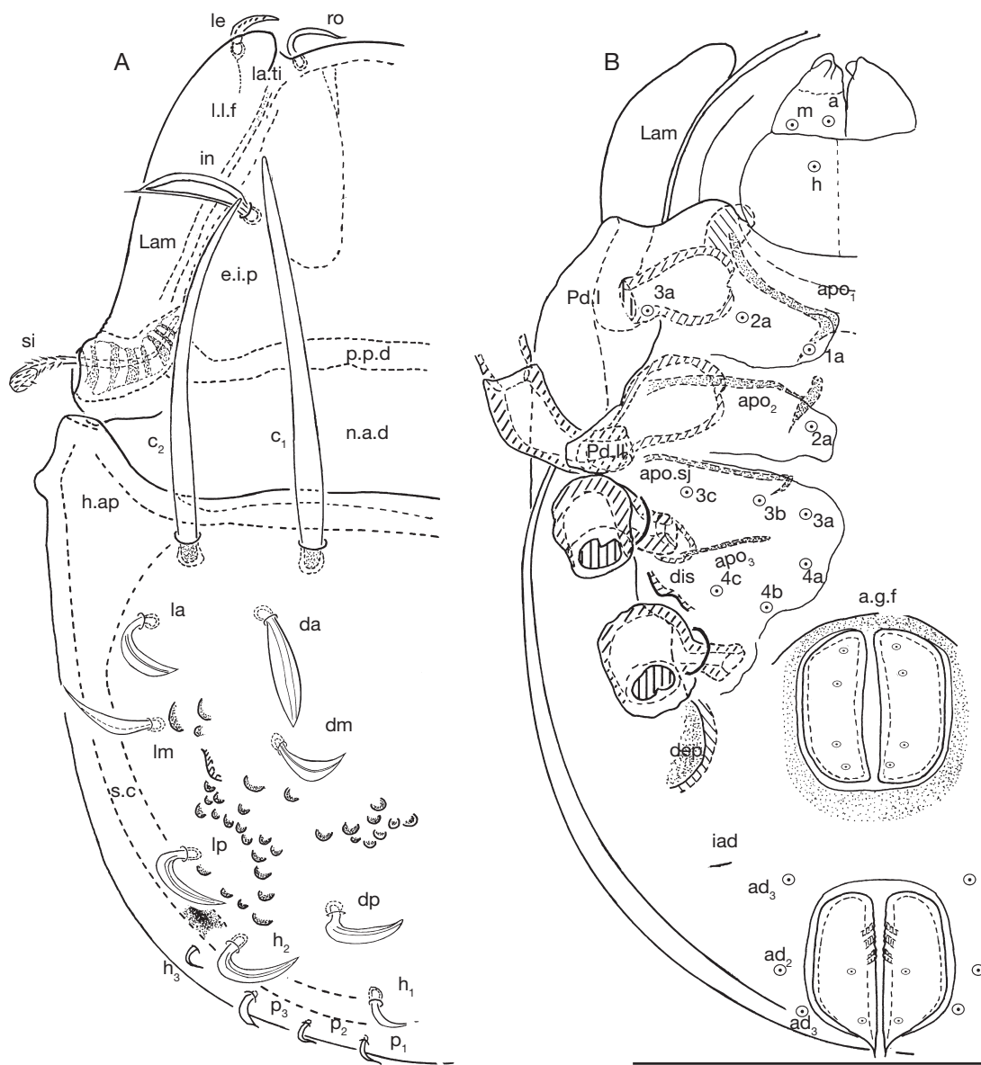
FIG. 2. — Congocepheus involutus Mahunka, 1997, adult: A , Dorsal view; B , ventral view. Abbreviations: see Material and methods. Scale bar: 100 \mu m.
