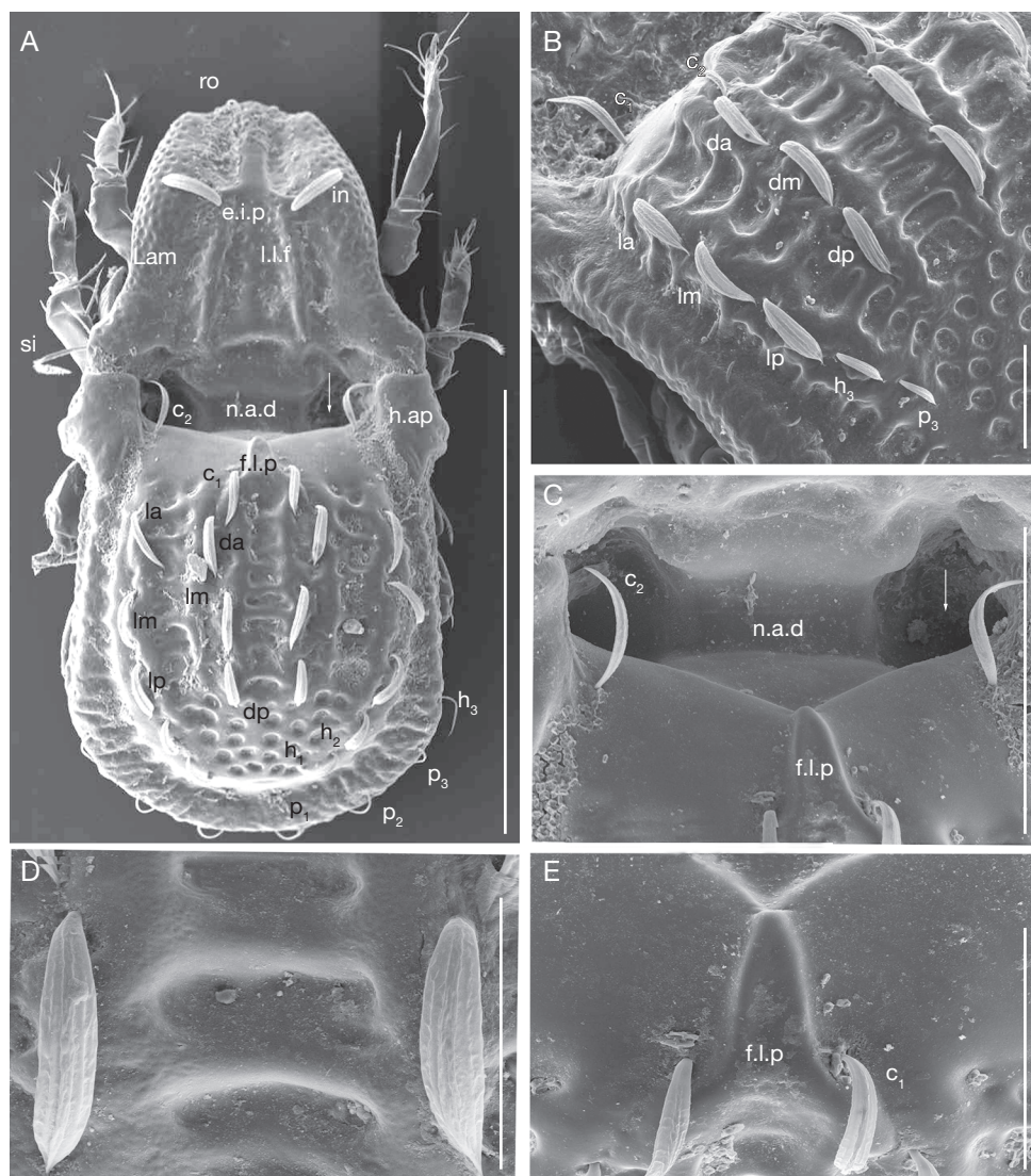
FIG. 11. — Congocephus extactesi n. sp. adult. scanning electron micrographs: A , dorsal view; B , anterior notogastral zone; C , notogastral anterior depression, dorsal view; D , microsculpture, between dp, notogastral setae; E , finger-like projection zone. Abbreviations: see Material and methods. Scale bars: A, 300 \mu m; B, E, 50 \mu m; C, 100 \mu m; D, 40 \mu m.
