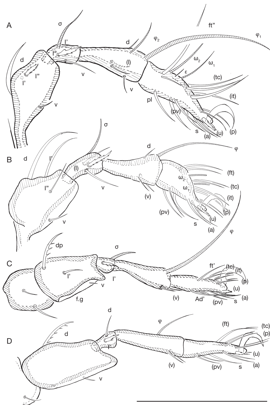
Fig. 10. — Congocepeus gabonensis n. sp. adult pattes. A , legs I, antiaxial; B , legs II, antiaxial; C , legs III, antiaxial; D , legs IV, antiaxial. Abbreviations: see Material and methods. Scale bar: 100 \mu m.
