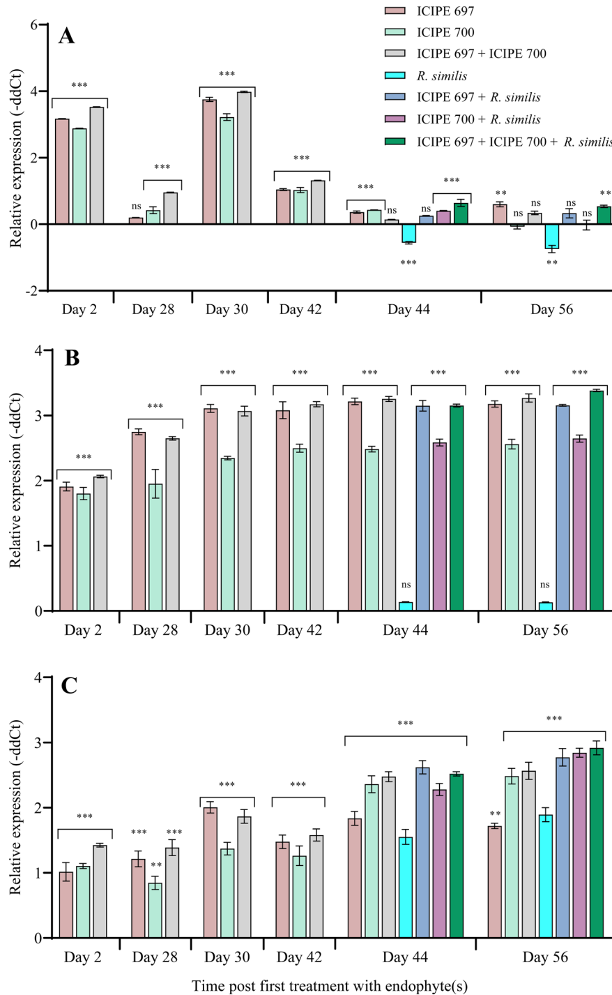
Fig. 5. Expression of defence-related genes calmodulin-Ca 2+ (A), \beta -1,3-glucan synthase (B) and PR-1 (C) in roots of fungal endophyte inoculated banana plants 'Ng'ombe' (EA-AAA) infected with or without 1000 Radopholus similis relative to non-treated control plants. At each day, asterisks indicate statistical significance relative to non-treated control as shown by Tukey's (HSD) test (*** P < 0.0001 ; ** P < 0.01 ; ns: no significant difference).
